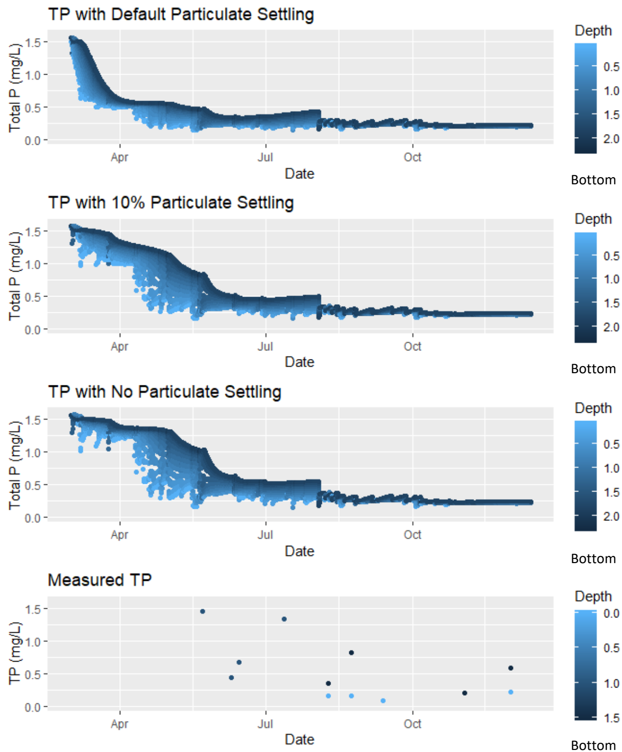
Figure 15: Comparison of model total phosphorus (TP) results with default particulate settling (POMS = 0.1 m/day), 10% particulate setting (POMS = 0.01 m/day) and no particulate settling (POMS = 0.0 m/day).
