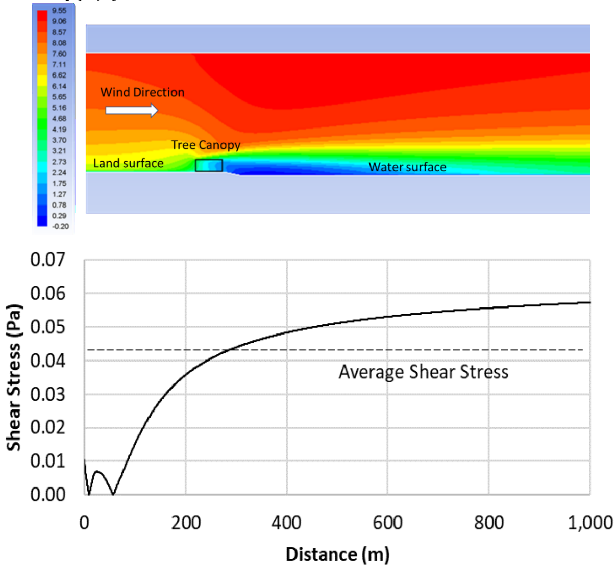
Figure 13: Sample output from a Fluent model, showing the wind velocity distribution (upper panel) going from upwind (left), over a 20-m (66-ft) wide line of trees, and onto a pond or lake surface, and the corresponding shear stress distribution on the water surface (lower panel).
