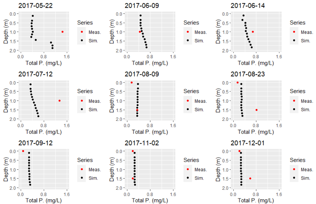
Figure A-4. Comparison of measured total phosphorus concentration profiles to corresponding total phosphorus concentration profiles from model output.
