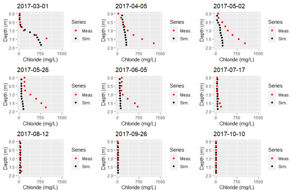
Figure A-1a. Comparison of measured chloride concentration profiles to corresponding chloride concentration profiles from model output. Part 1 of 2.
