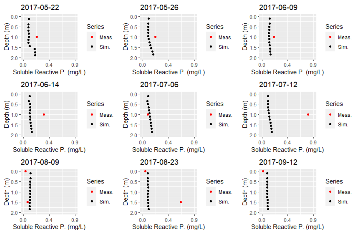
Figure A-3a. Comparison of measured soluble reactive phosphorus concentration profiles to corresponding soluble reactive phosphorus concentration profiles from model output. Part 1 of 2.
