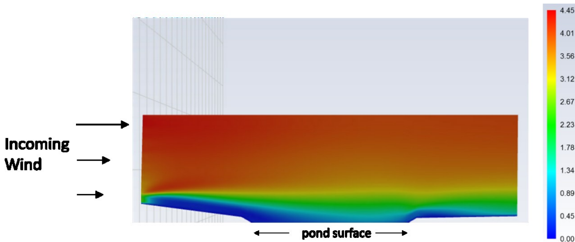
Figure 23: The first graph shows the simulated wind velocity distribution in and around the Shoreview pond (map view). The blue areas are forested and sheltered areas with low wind velocity. The simulation domain is approximately 300 m long x 300 m wide x 100 m tall (980 ft x 980 ft x 320 ft). The second graph shows the simulated wind velocity distribution in and around the Alameda pond (cross-section view along pond centerline), showing the approximate pond embankment and the surrounding topography. The blue areas are forested and sheltered areas with low wind velocity.
