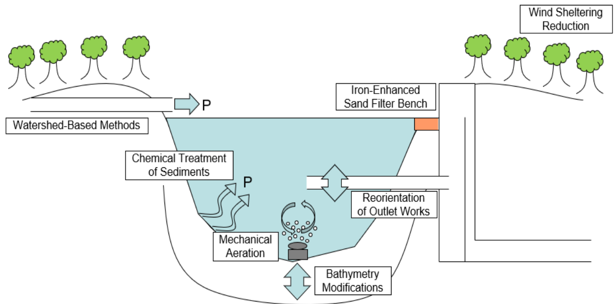
Figure 1: Conceptual diagram of the seven remediation strategies.
