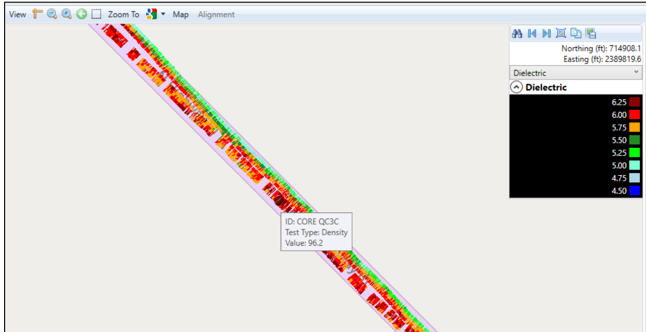
Figure 16. Screenshot. Location of single acceptance core.
