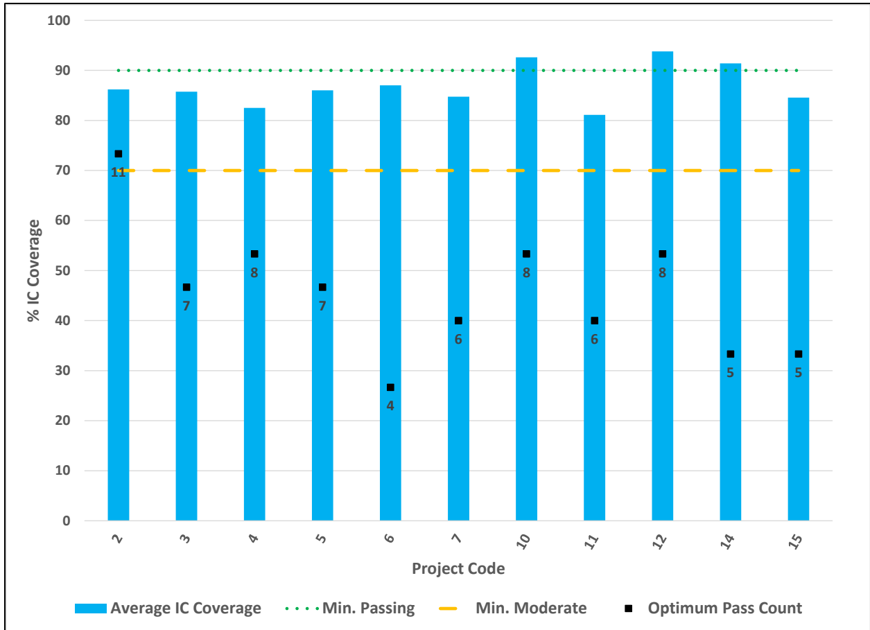
Figure 26. Chart. Average IC coverage per project and optimum pass counts.
