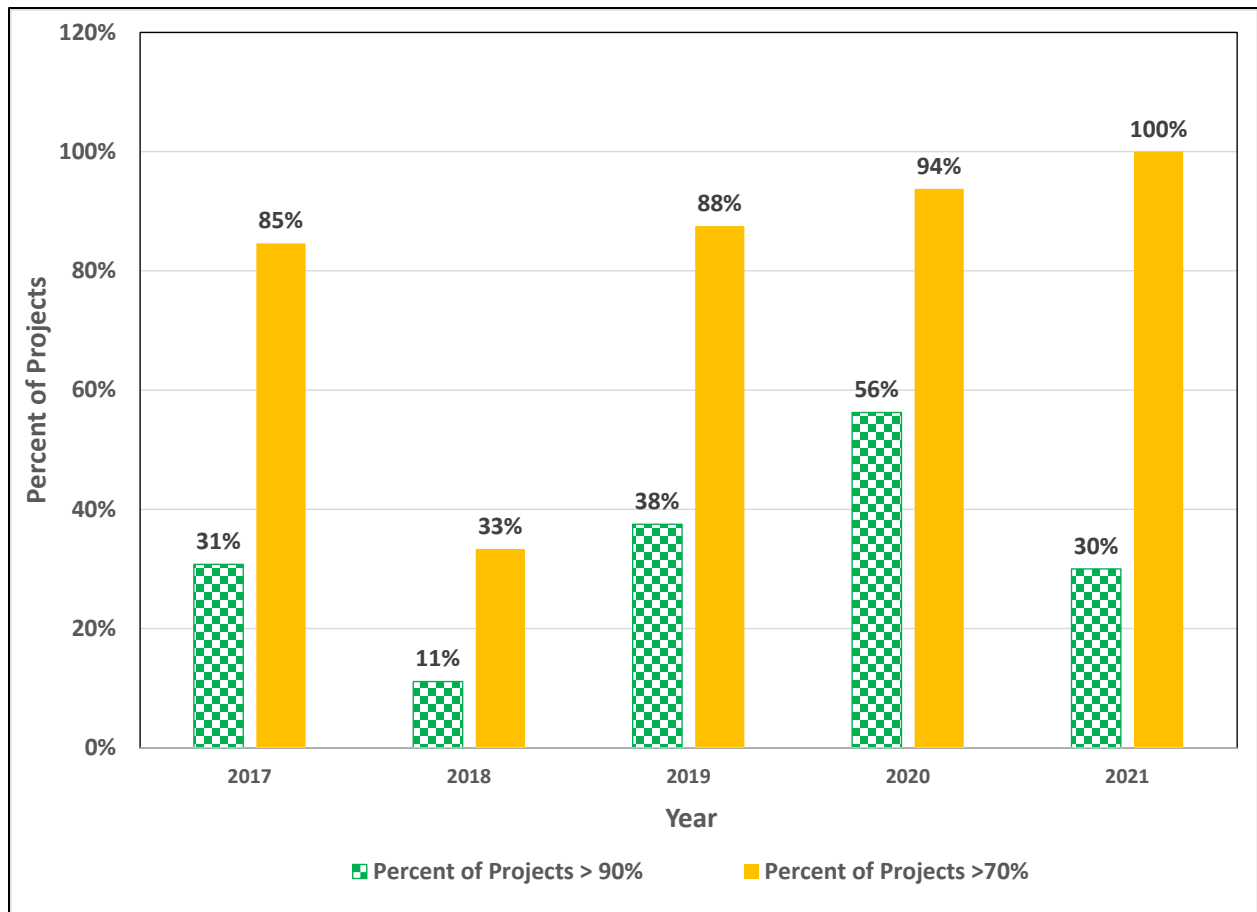
Figure 33. Chart. Percent of projects that meet the 70 percent and 90 percent thresholds per construction season.
