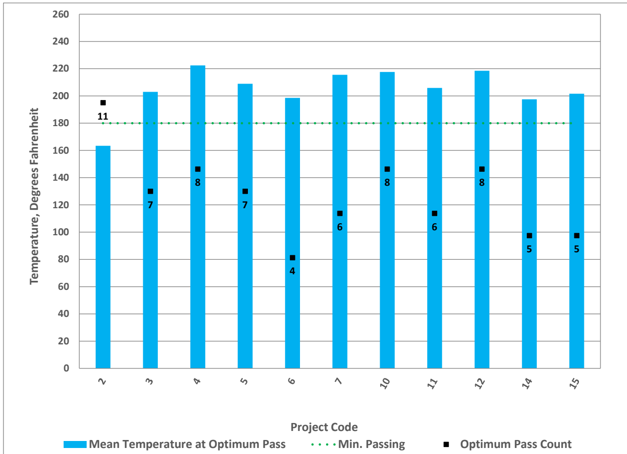
Figure 27. Chart. The average mean temperature at optimum pass count per project and optimum pass counts.
