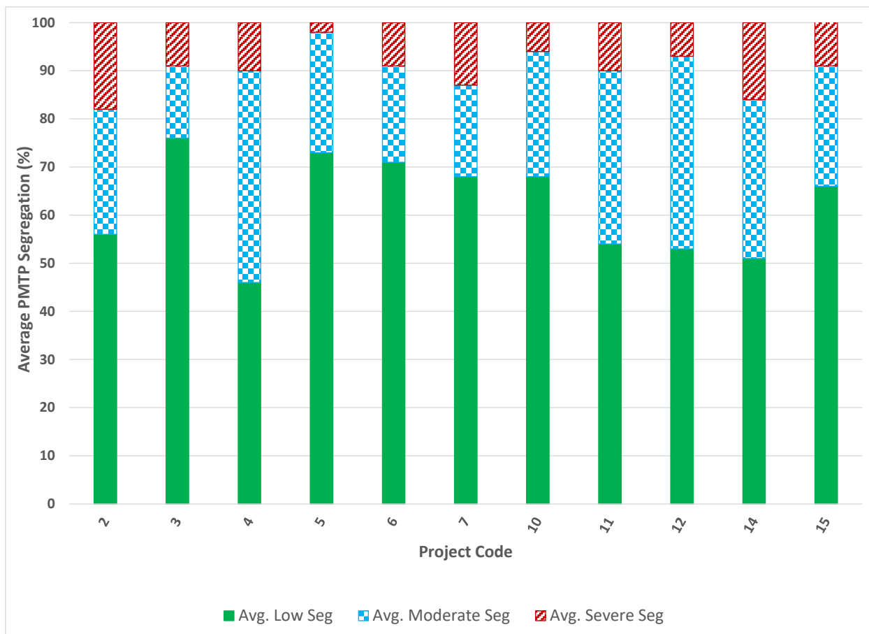
Figure 29. Chart. Average thermal segregation classification for each project.
