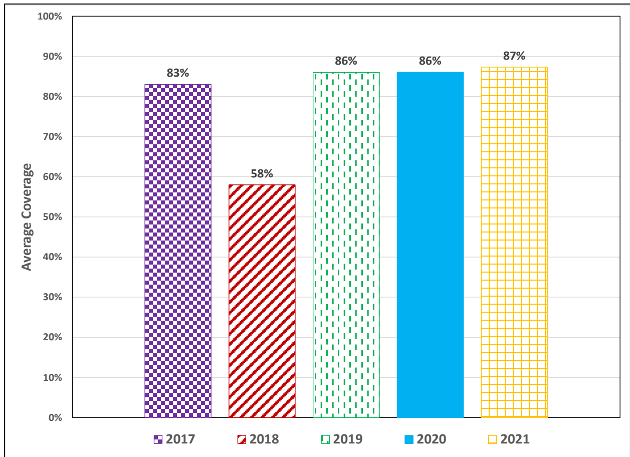
Figure 32. Chart. Average IC percent coverage for all projects per construction season.
