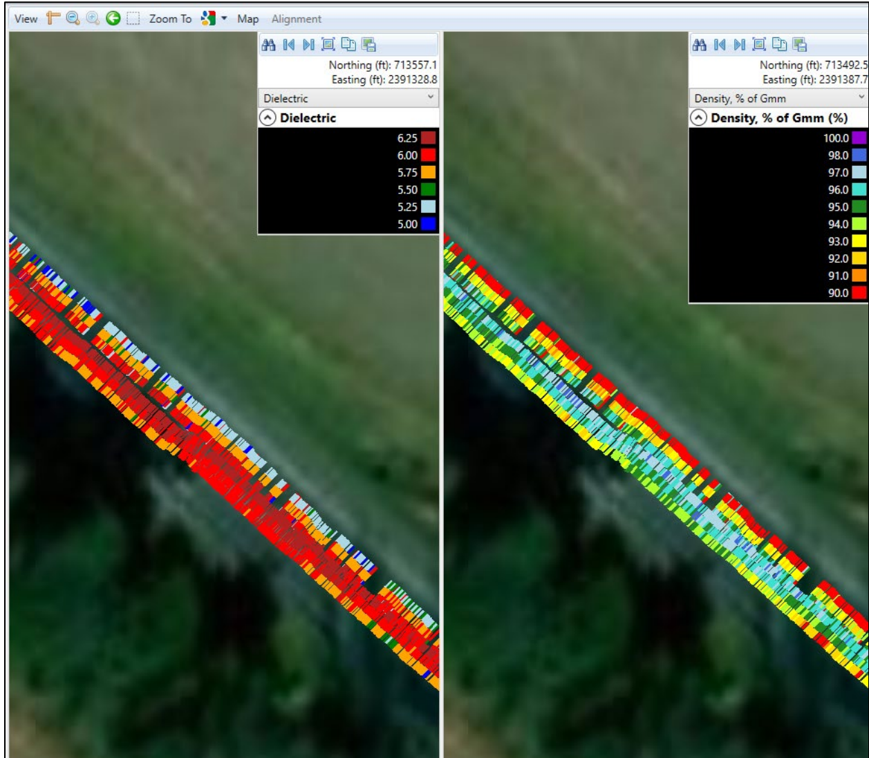
Figure 13. Screenshot. Low dielectric data (left) and estimated relative density (right) were observed at the data's edge.
