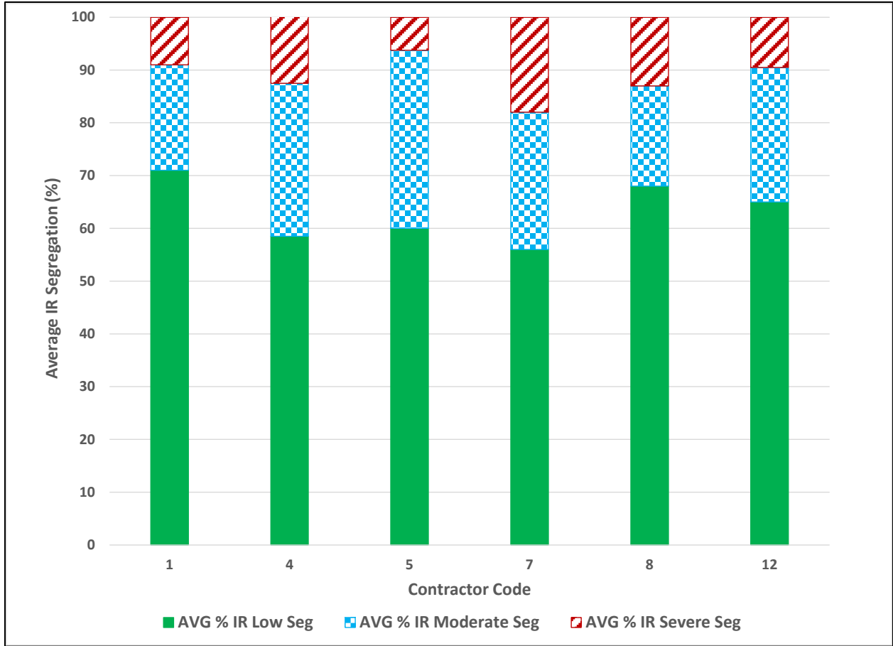
Figure 30. Chart. Average PMTP thermal segregation classification per contractor.
