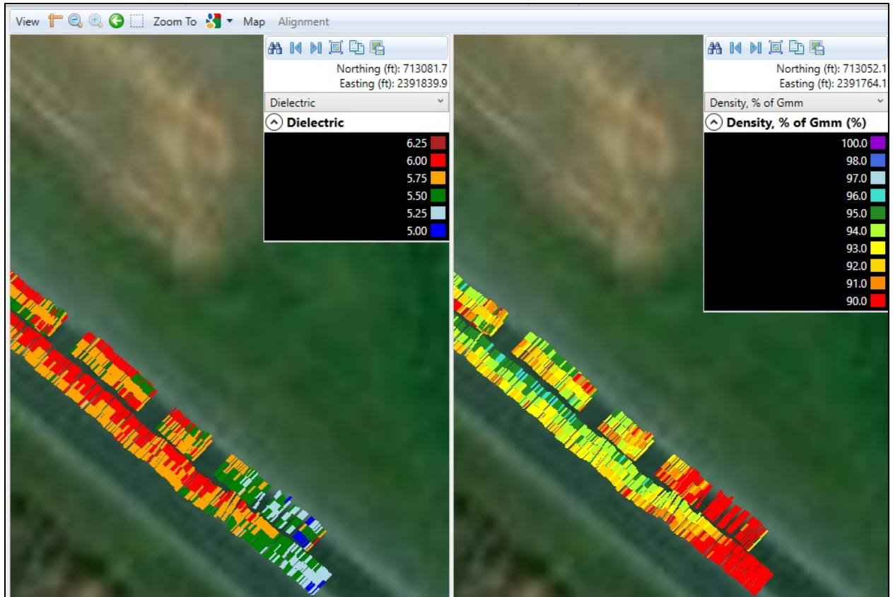
Figure 10. Screenshot. Relatively low dielectric data at the start of paving at the transverse joint.
