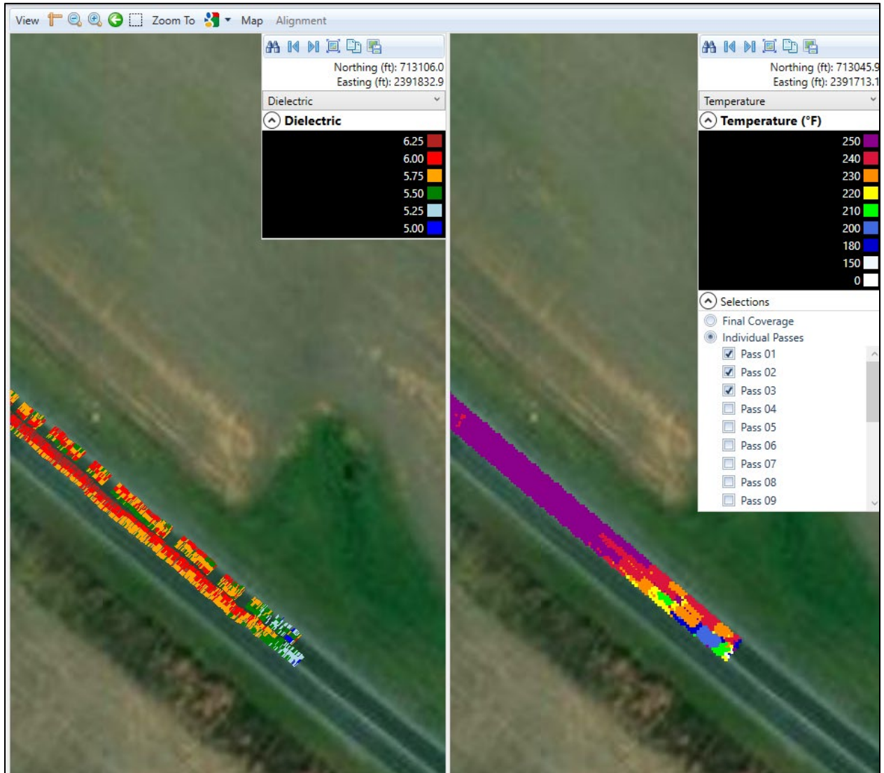
Figure 12. Screenshot. Cooler breakdown temperatures relative to the rest of production, with corresponding lower dielectric values.
