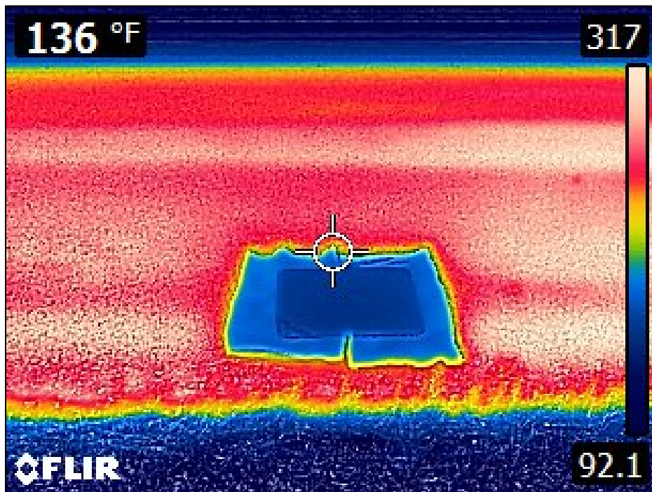
Figure 24. Photo. Improved reference object met the dimensions required and stayed below 150°F during testing.
