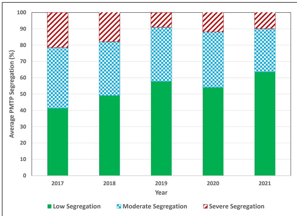
Figure 31. Chart. Average PMTP thermal segregation classification for all projects per construction season.
