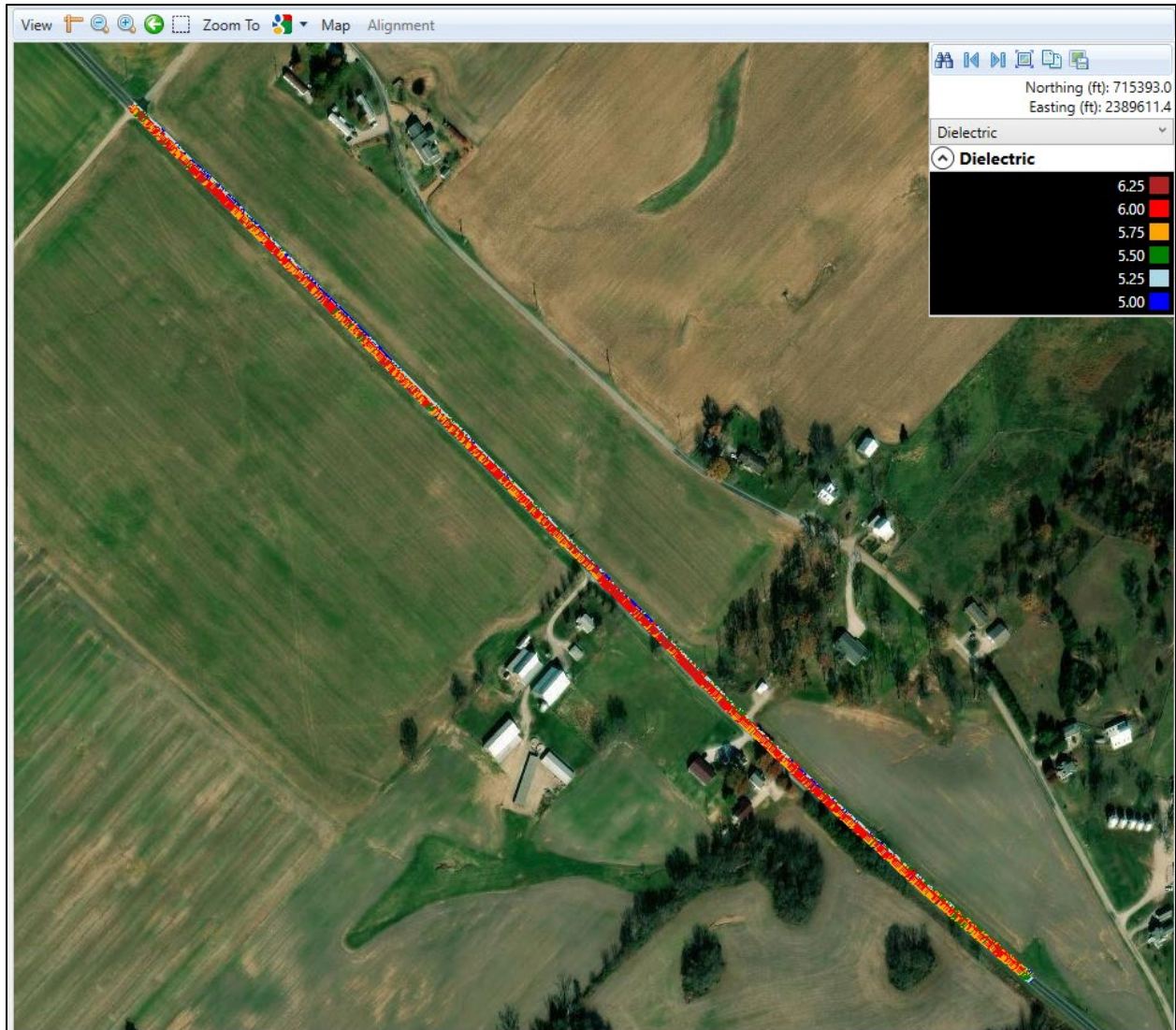
Figure 5. Screenshot. The extent of dielectric data collected using the RDM 2.0 on Project Code 4
