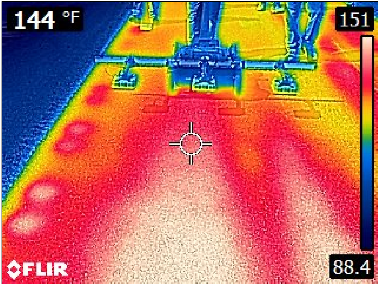
Figure 7. Photo. Example FLIR image capturing data collection temperatures
