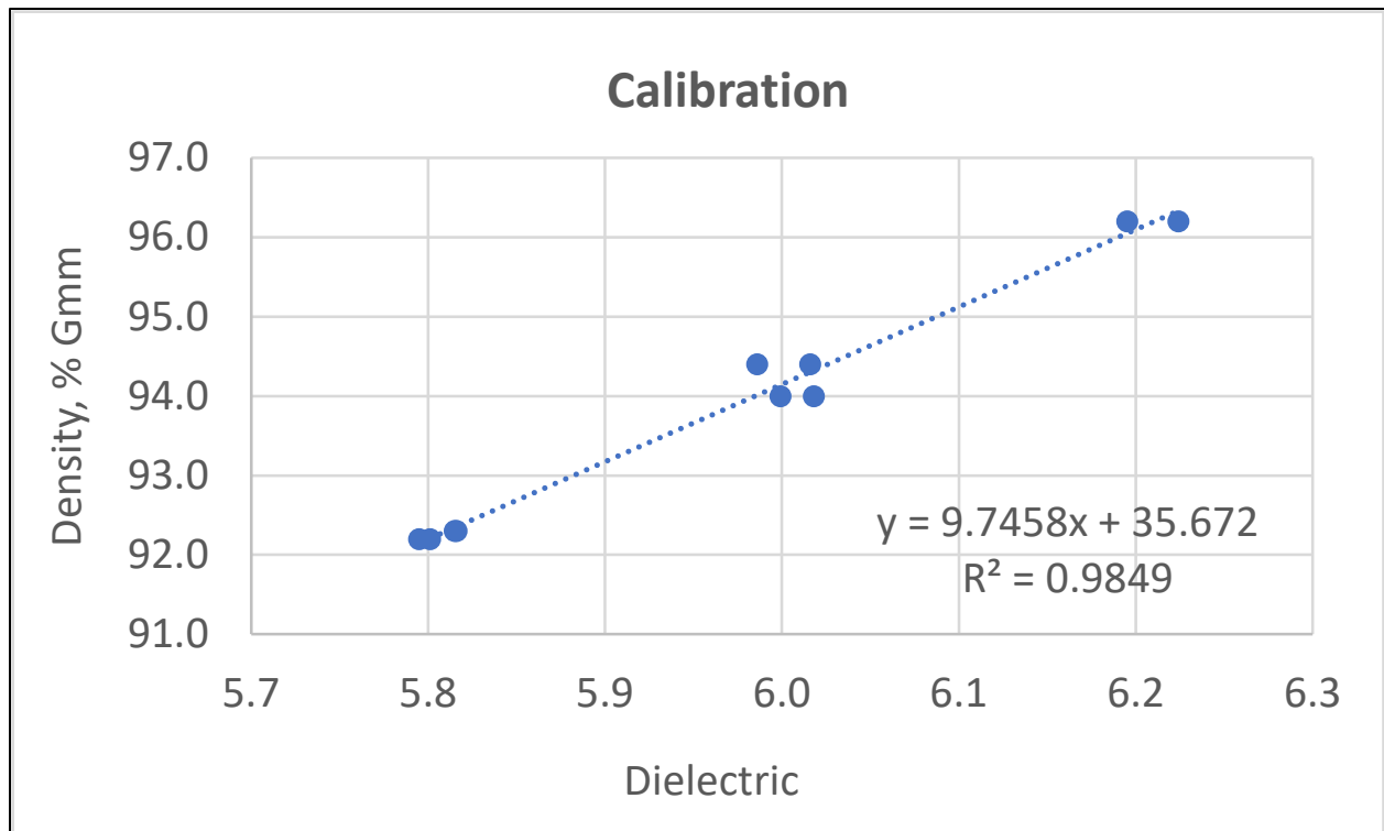
Figure 9. Graph. Calibration data from gyratory samples.
