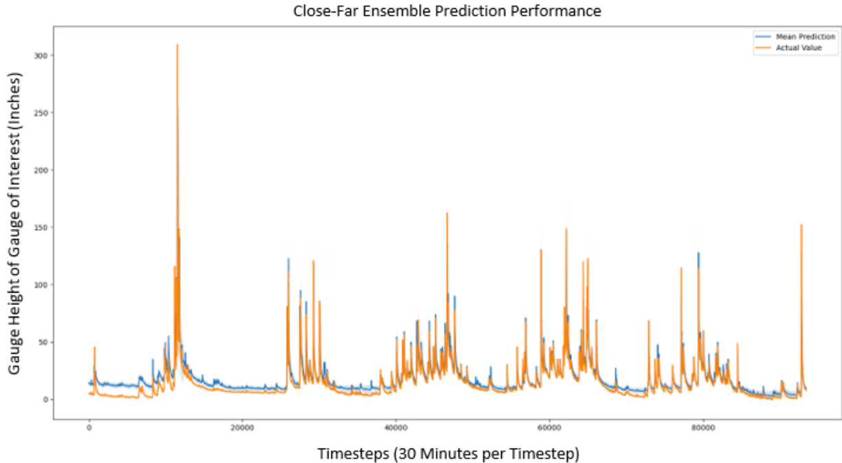
Figure 15: Comparison of Predicted and True Gauge Height Values for ‘Close-Far’ (CF) Gauge Grouping.
