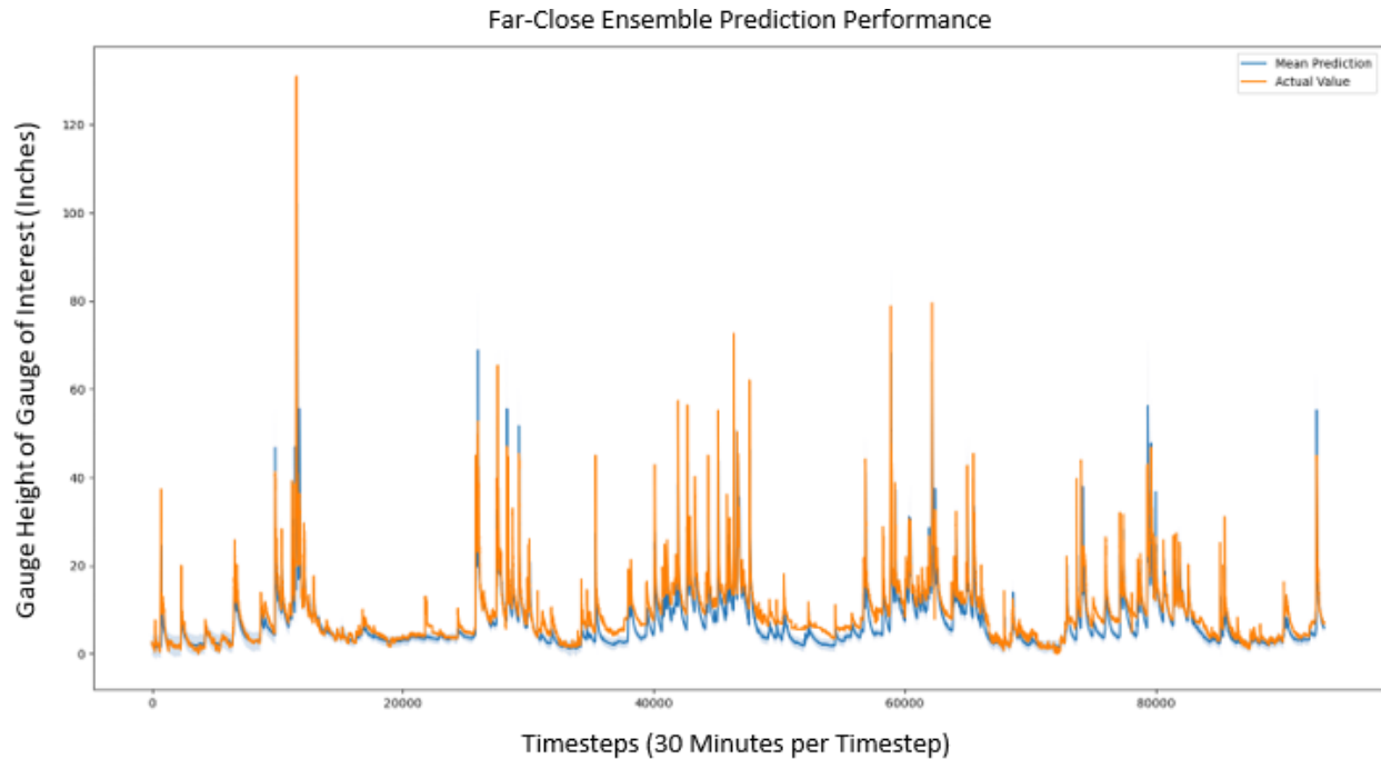
Figure 17: Comparison of Predicted and True Gauge Height Values for ‘Far-Close’ (FC) Gauge Grouping.
