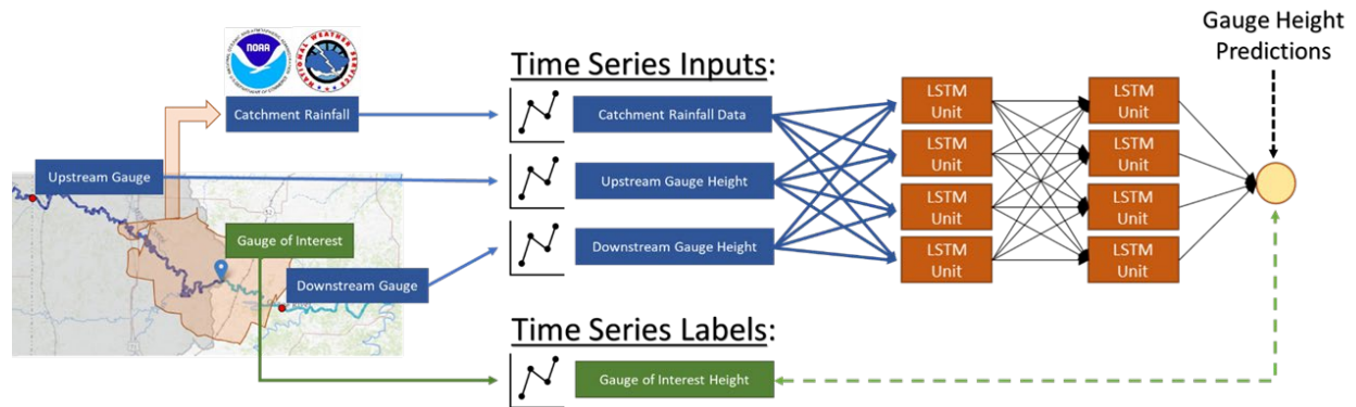
Figure 9: LSTM Deep Learning Neural Networks Framework for Gauge Height Predictions.
