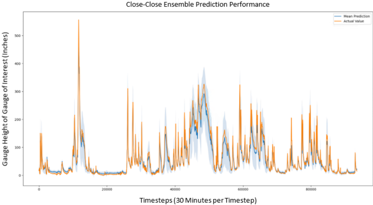
Figure 13: Comparison of Predicted and True Gauge Height Values for ‘Close-Close’ (CC) Gauge Grouping.
