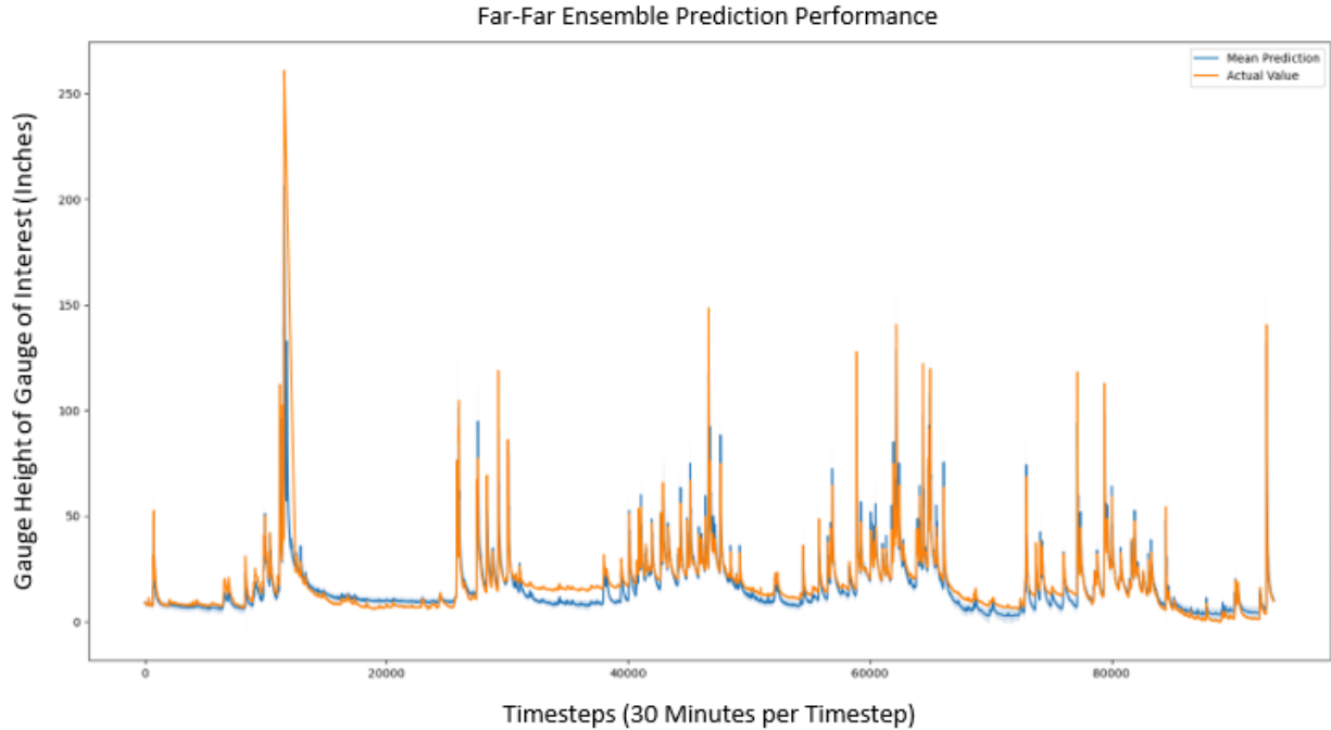
Figure 19: Comparison of Predicted and True Gauge Height Values for ‘Far-Far’ (FF) Gauge Grouping.
