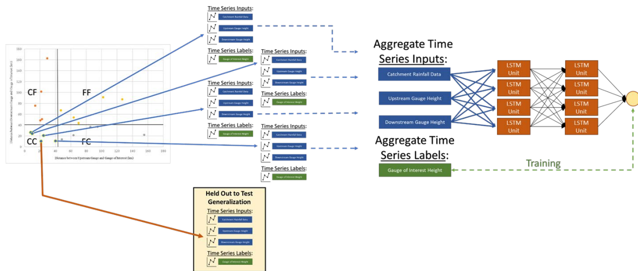
Figure 11: Gauge Groupings and Deep Learning Models.
