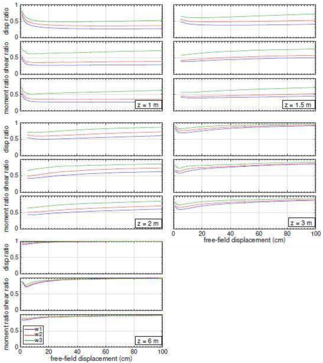
Figure 4.25 Bending demand ratios taken against the full-width embankment case for five crust thicknesses with D = 1.4\text{ m} and t = 6\text{ m}
