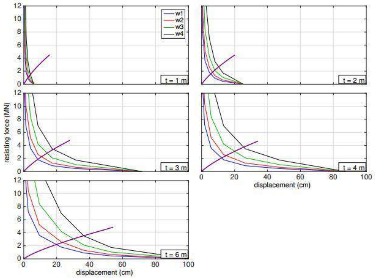
Figure 5.9 Determination of compatible displacement from pushover and slope deformation curves for five liquefiability layer thicknesses and four embankment crest widths with a 2.0-m crustal thickness and 1.4-m diameter shaft
