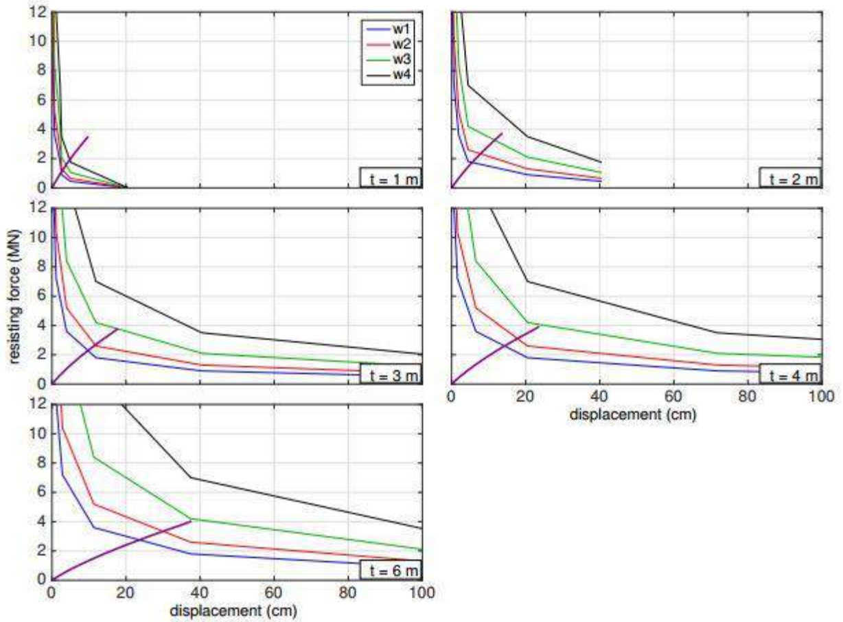
Figure 5.7 Determination of compatible displacement from pushover and slope deformation curves for five liquefiability layer thicknesses and four embankment crest widths with a 1.0-m crustal thickness and 1.4-m diameter shaft
