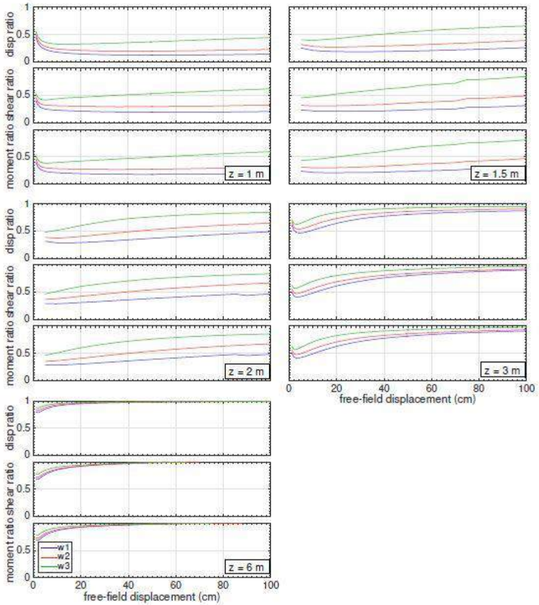
Figure 4.18 Bending demand ratios taken against the full-width embankment case for five crust thicknesses with D = 0.6 m and t = 3 m
