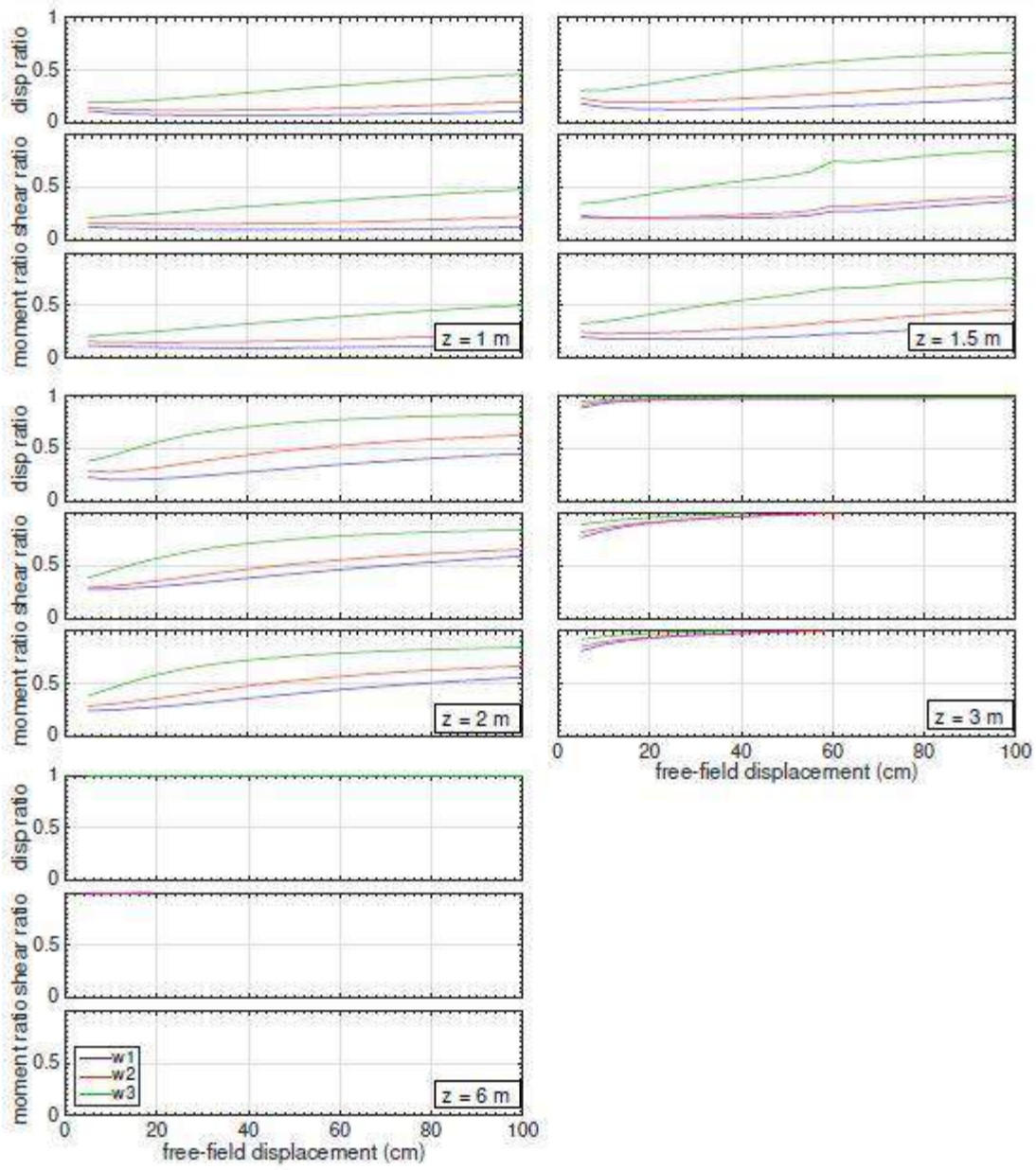
Figure 4.17 Bending demand ratios taken against the full-width embankment case for five crust thicknesses with D = 0.6 m and t = 2 m
