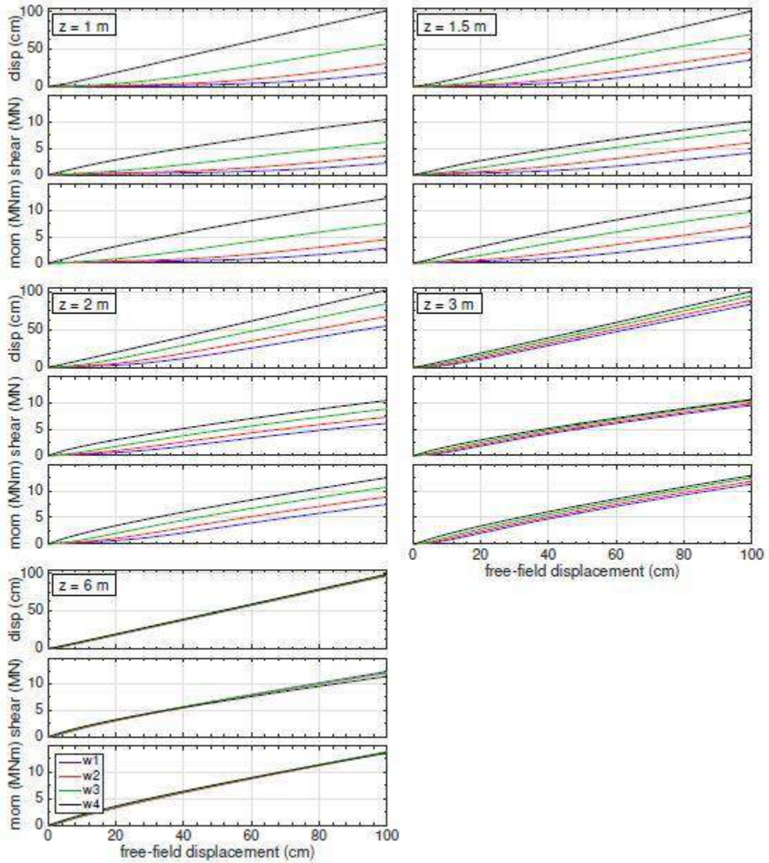
Figure 4.6. Maximum shaft bending demands with increasing free-field displacement for five crust thicknesses with D = 0.6 m and t = 1 m.
