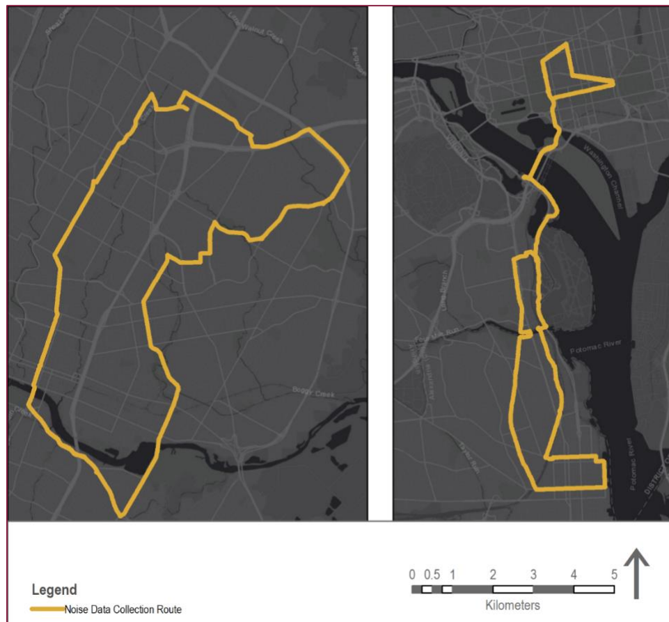
Figure 1. Noise data collection routes in Austin (TX) at left, and the Washington, D.C. metro area at right.
