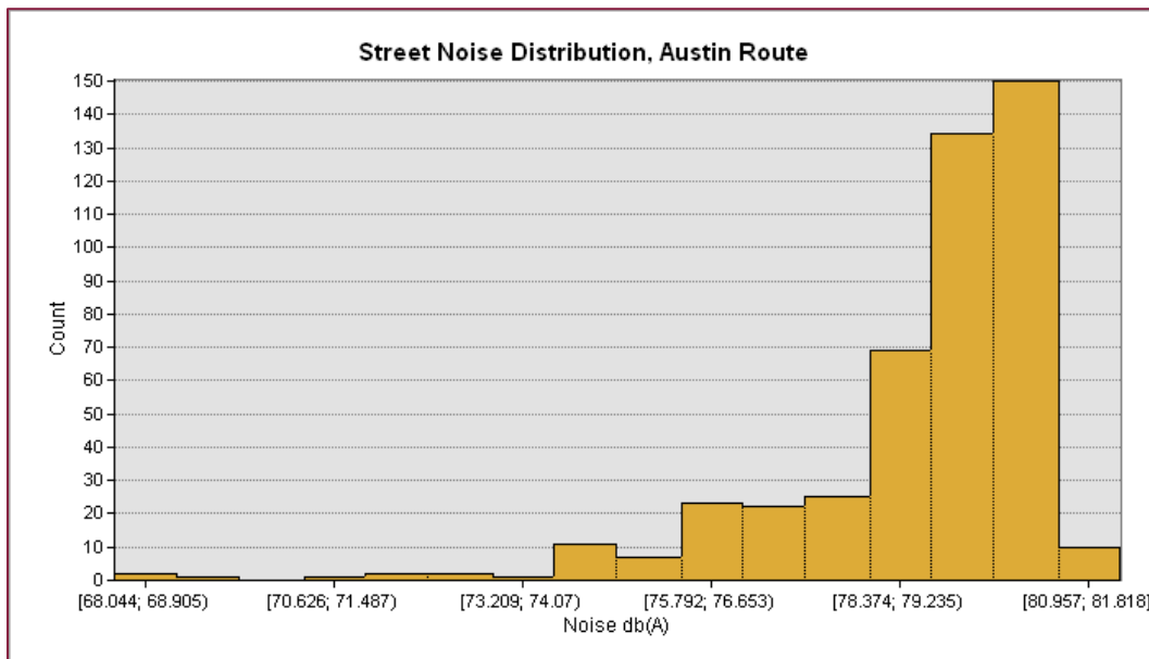
Figure 8. Histogram of average noise recorded by bicyclists along route in Austin, TX.
