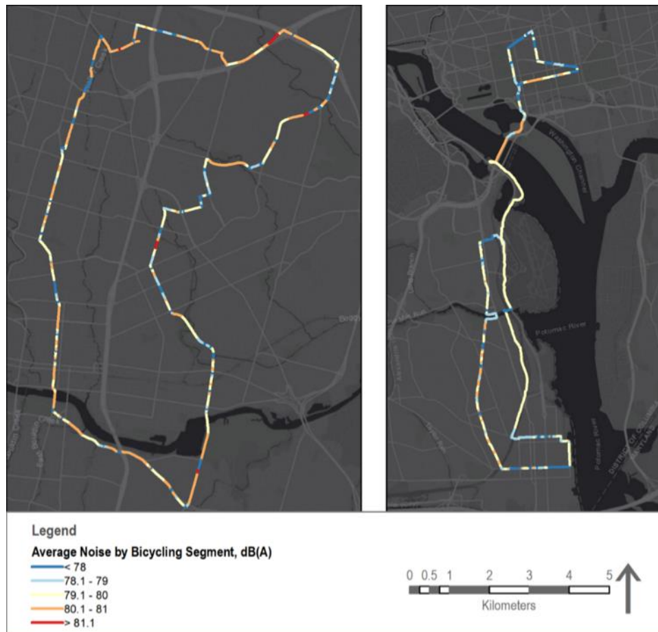
Figure 7. Average noise recorded by bicyclists along routes in Austin, TX (SH 290) at left, and the Washington, D.C. (I-395) metro area at right.
