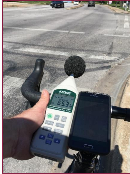
Figure 3. Street noise measurement with reference noise meter and bicycle-mounted smartphone.
