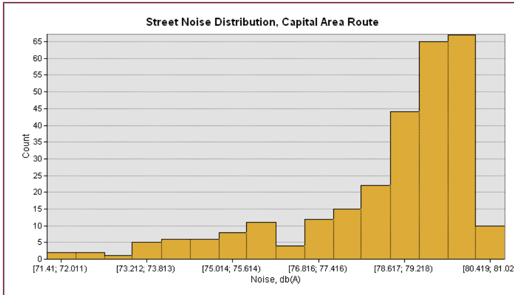
Figure 9. Histogram of average noise recorded by bicyclists along route in the Washington, D.C. metro area.
