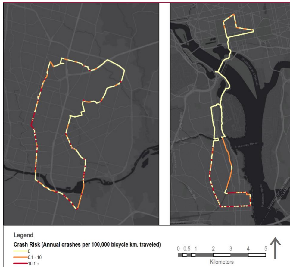
Figure 6. Bicycle crash risk (annual crashes per 100,000 bicycle kilometers, or 62,137 mi., traveled) along noise data collection routes in Austin, TX at left, and the Washington, D.C. metro area at right.
