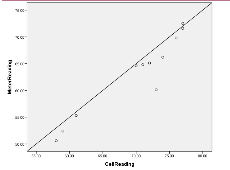
Figure 4. Scatter plot of cell reading/meter reading intercepts for each of the 11 sites.
