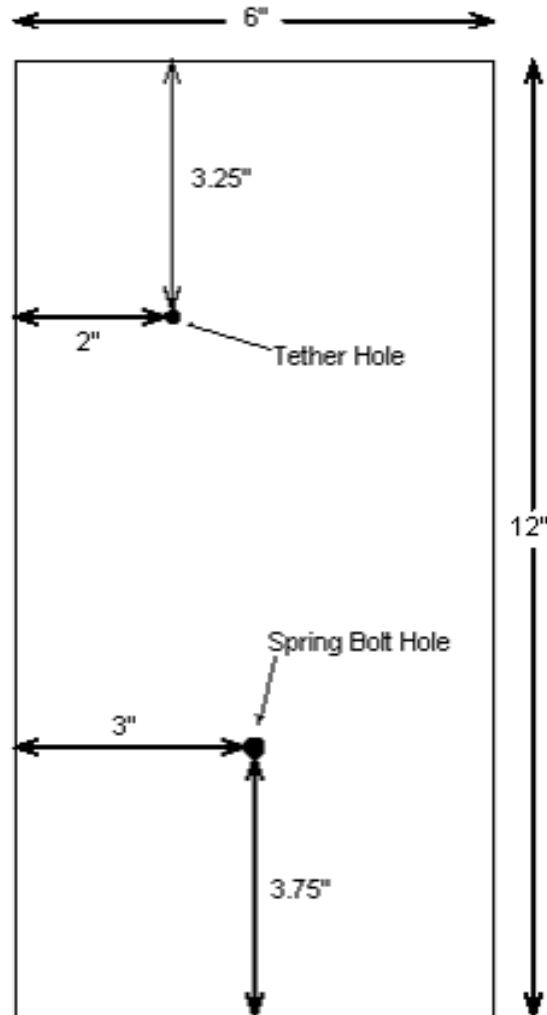
Figure 47. Backing Plate for Cutout
