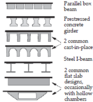
Figure 27. Cross-sections of Common Bridge Designs
