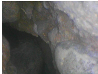
Figure 5-12: Boroscope view of gaps in non-grouted and deteriorated retaining walls by ME-concrete
