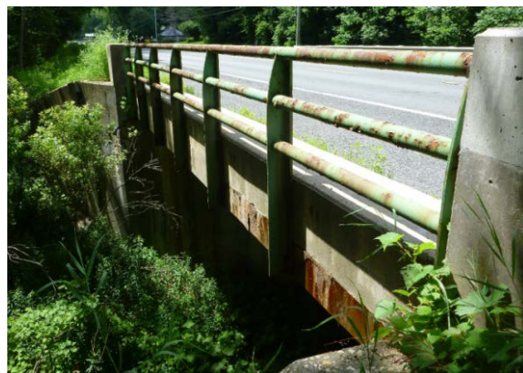
Figure 5-39: Concrete bridge selected in MA (MA-precast_concrete_2)
