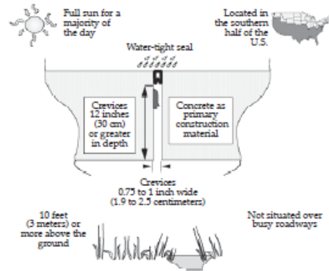
Figure 28. Ideal Highway Structure Roost Characteristics
