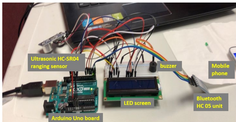
Figure 4.6 The prototype of Arduino based system
