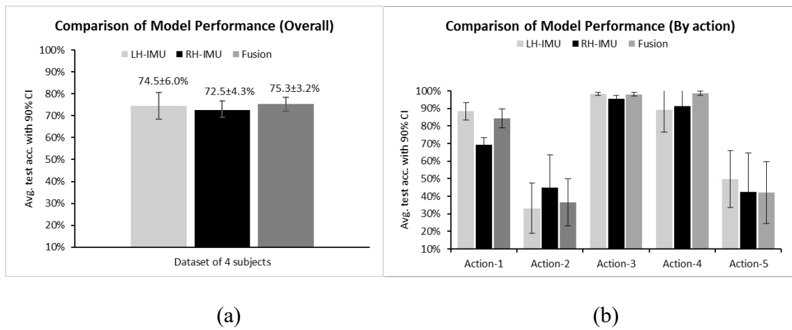
Figure 3.20 Model performance comparison (a), the comparison at action level (b)
