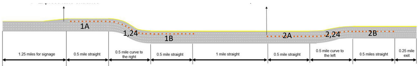
Figure 4-15: Express Lanes Layout
