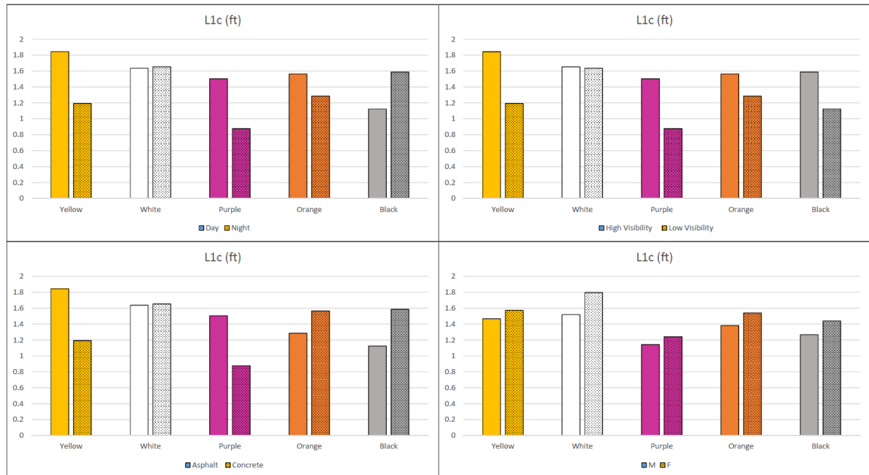
Figure 4-28: Effect of Color on Lane Deviation at 1-24 in Different Driving Conditions
