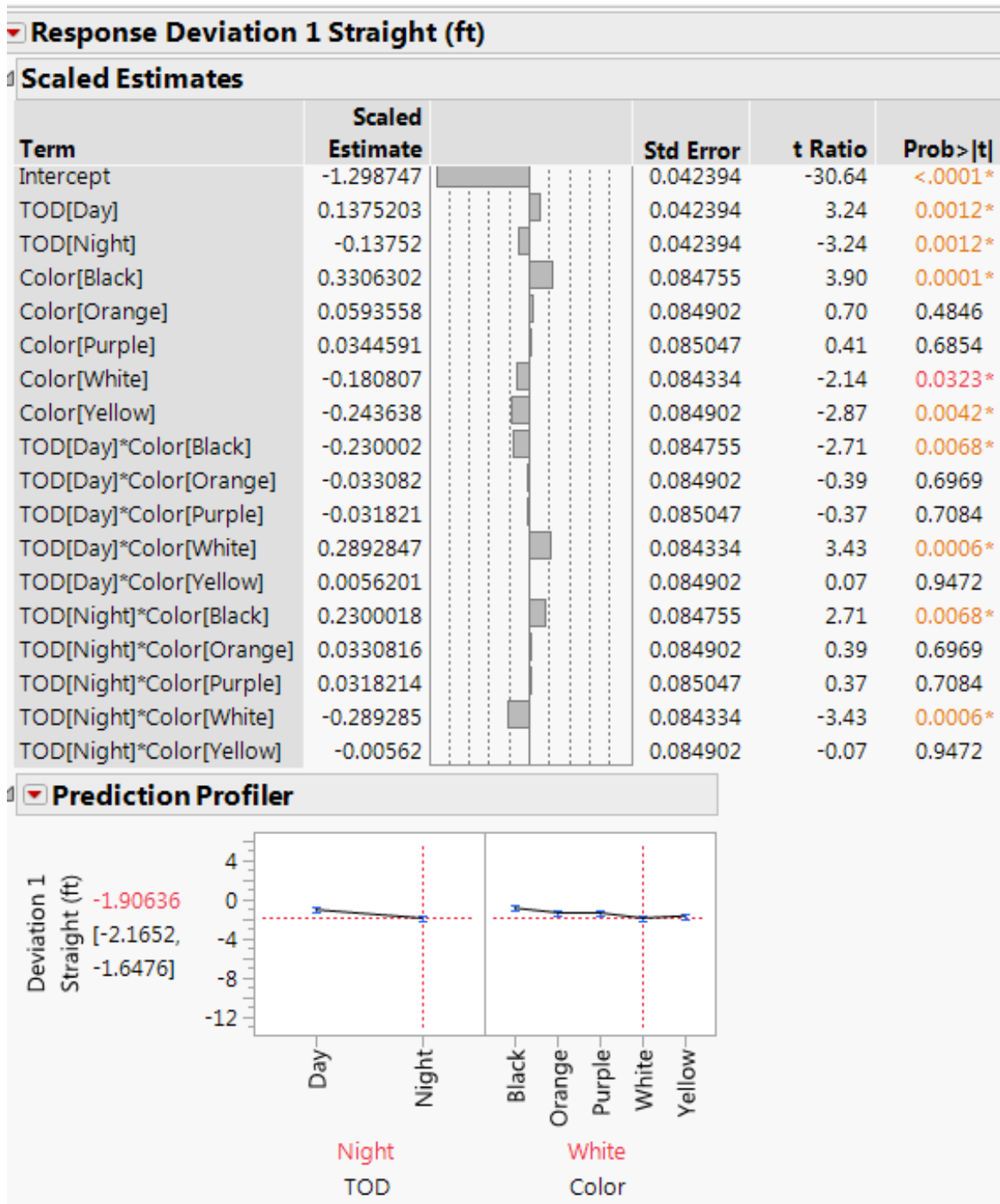
Figure 4-25: Time of Day and Color Effect on Lane Deviation at Section 1A
