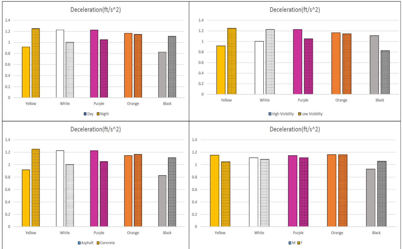
Figure 4-21: Effect of Color on Deceleration Rates in Different Driving Conditions
