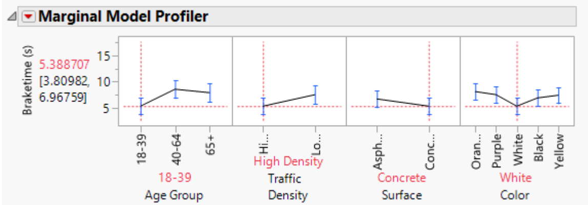
Figure 5-13: Profiler Results for Brake Time
