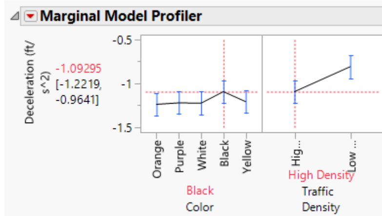
Figure 5-11: Profiler Results for Deceleration
