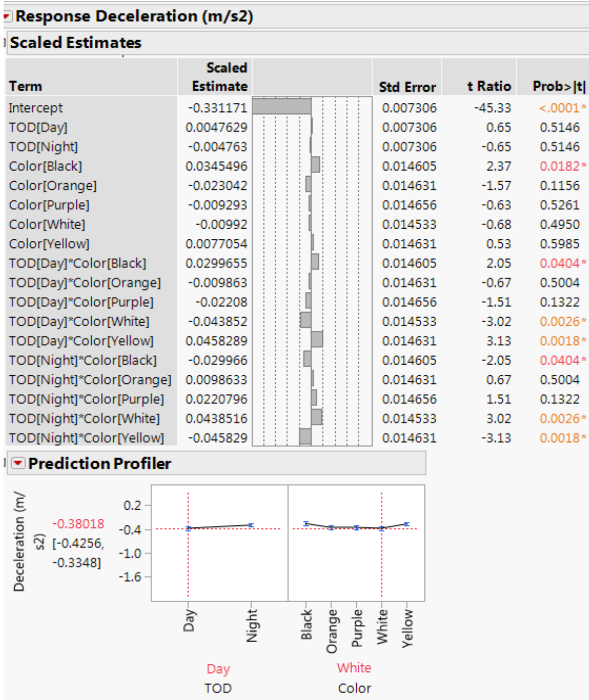
Figure 4-18: Time of Day and Color Effect on Deceleration Rates
