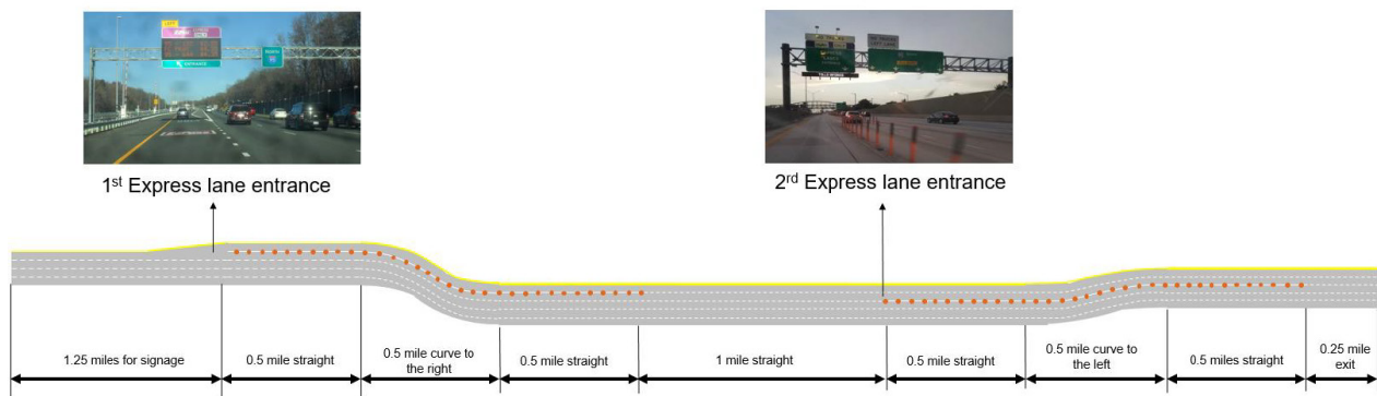
Figure 3-8: Roadbed and Lane Configurations
