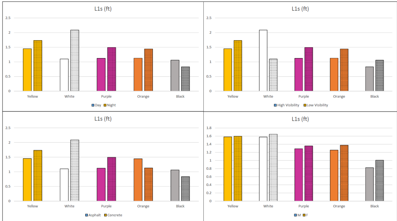
Figure 4-27: Effect of Color on Lane Deviation at 1A in Different Driving Conditions
