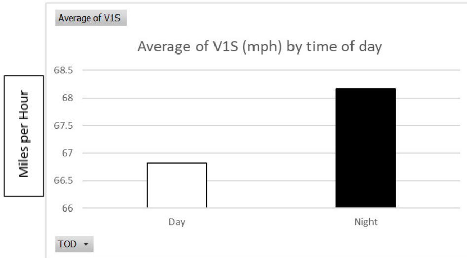
Figure 5-19: Impact of TOD on Entering Velocity
