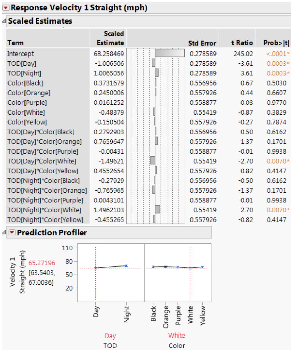
Figure 4-22: Time of Day and Color Effect on Speed at Section 1A
