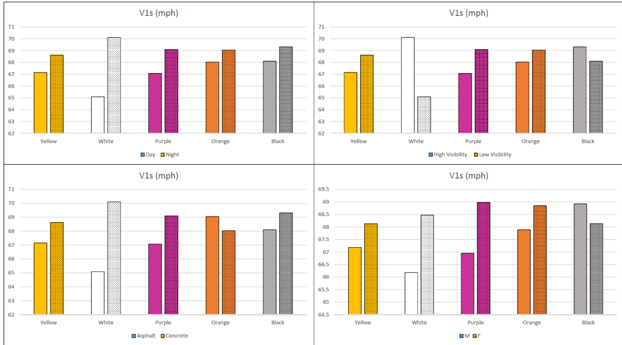
Figure 4-23: Color Effect on Speed at Section 1A in Different Driving Conditions
