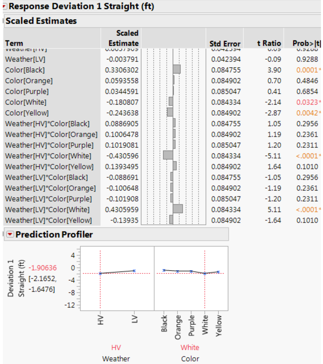
Figure 4-26: Effect of Color on Lane Deviation at Section 1A
