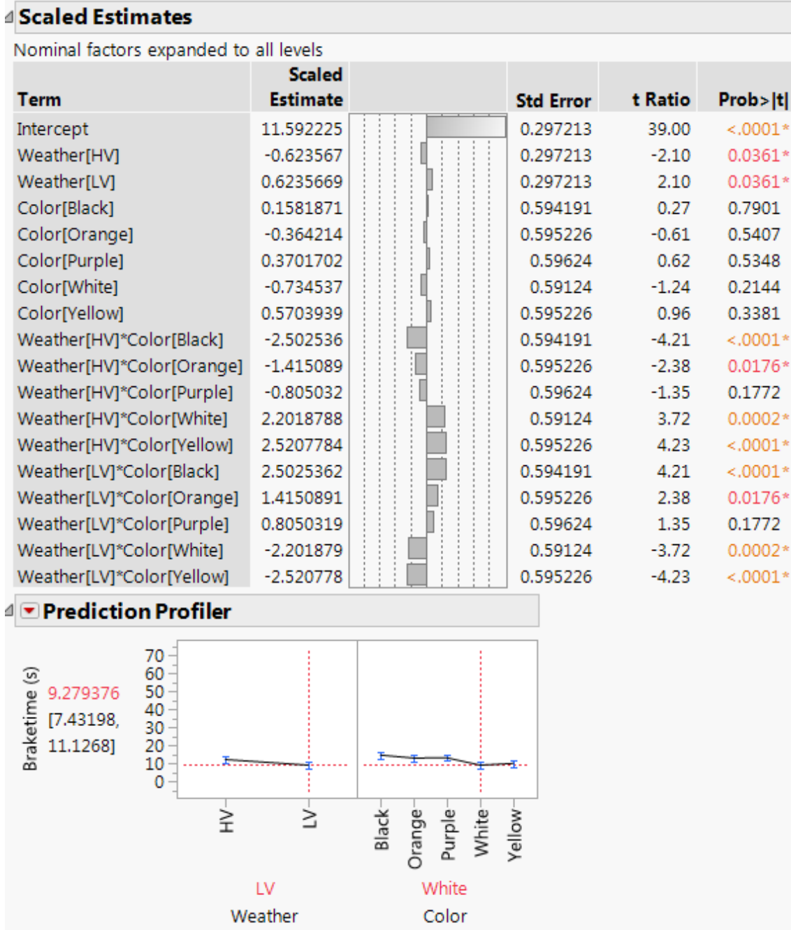
Figure 4-20: Weather and Color Effect on Brake Time
