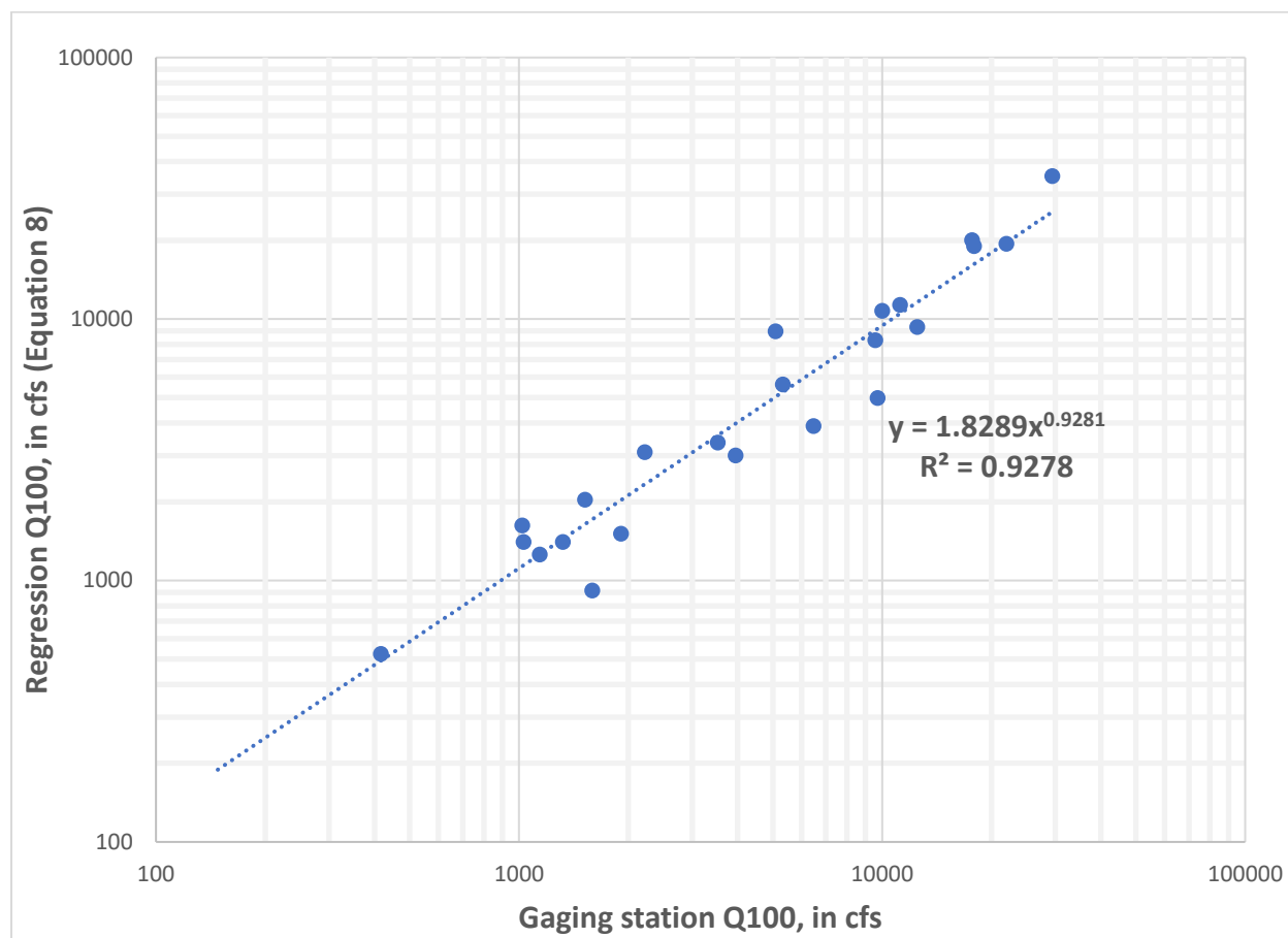
Figure 5. The 100-year regression estimates from Equation 8 plotted versus the 100-year estimates based on gaging station data for 23 stations in the Western Coastal Plain Region.
