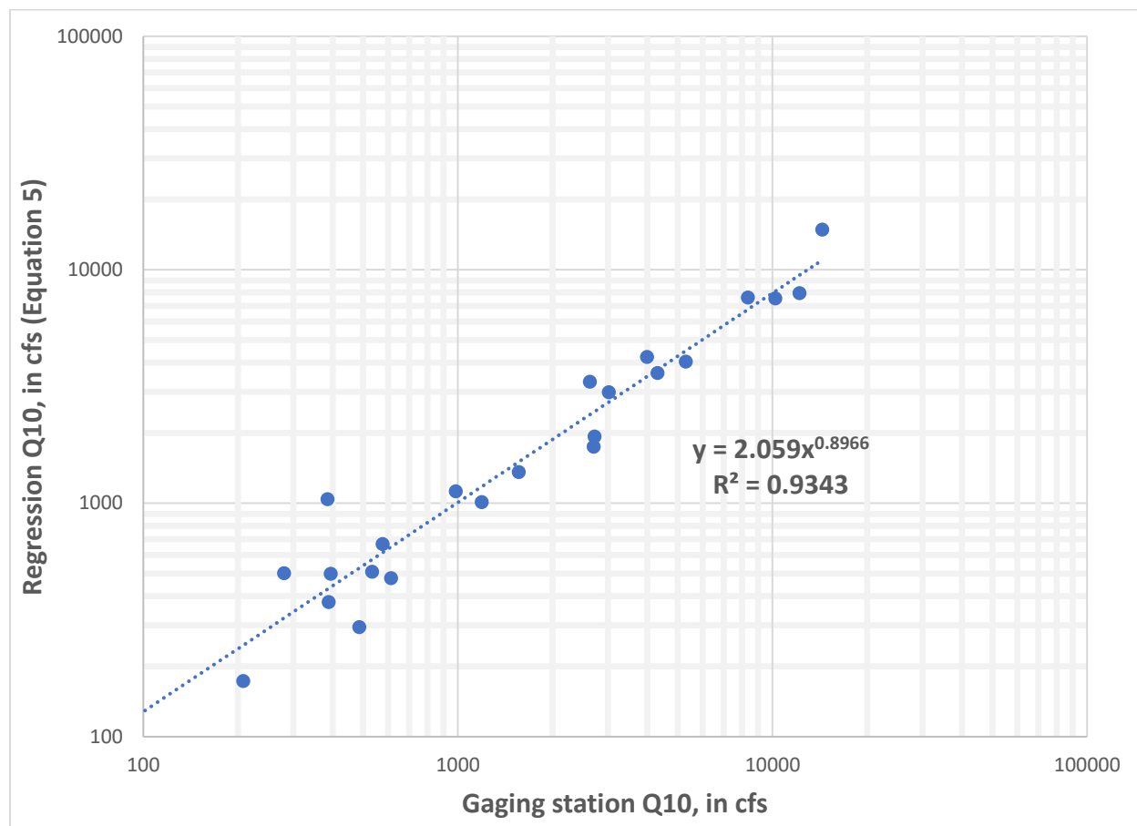
Figure 6. The 10-year regression estimates from Equation 5 plotted versus the 10-year estimates based on gaging station data for 23 stations in the Western Coastal Plain Region.
