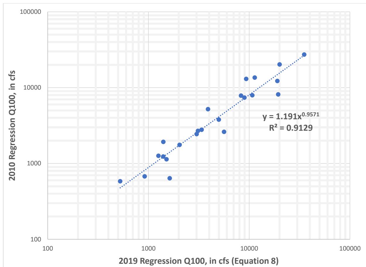
Figure 7. Comparison of the 100-year flood discharges for the 2010 and 2019 regression equations.
