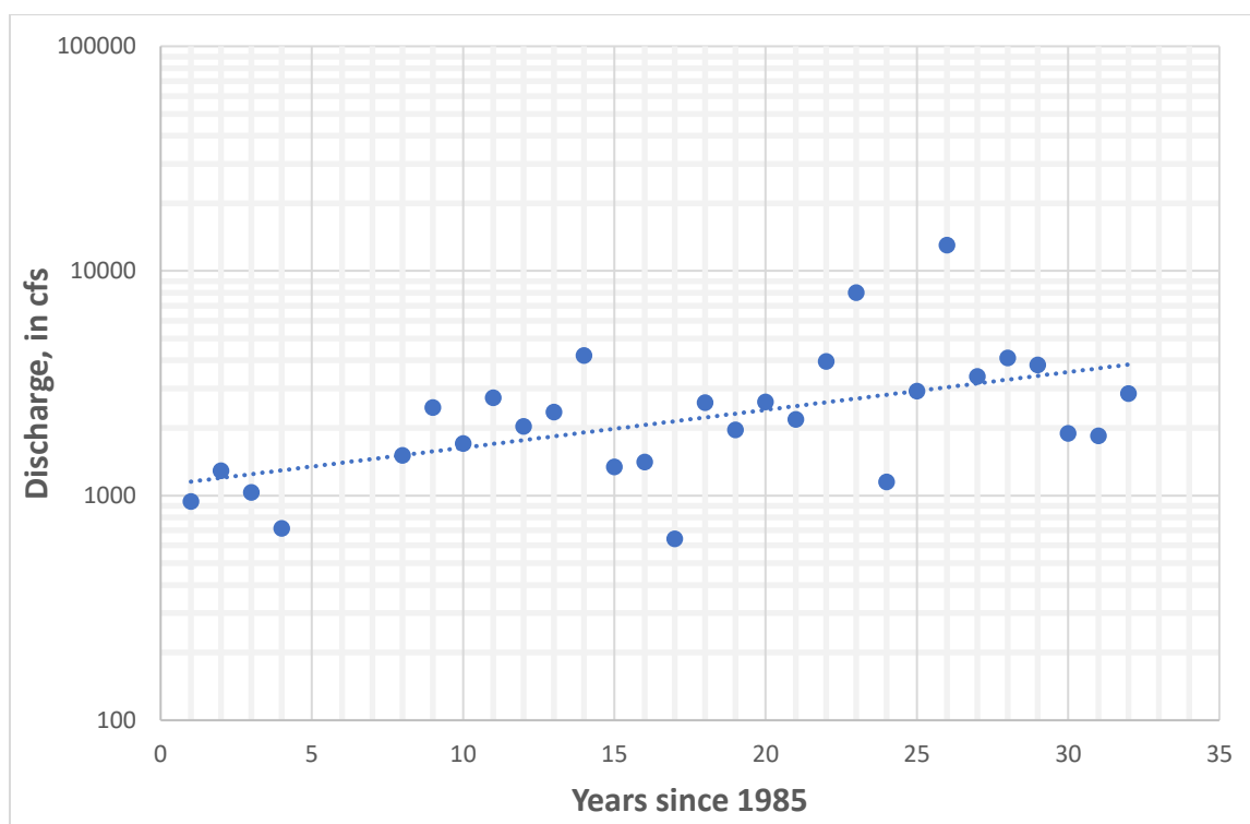
Figure A2-1. Relation between annual peak flows and years since 1985.
