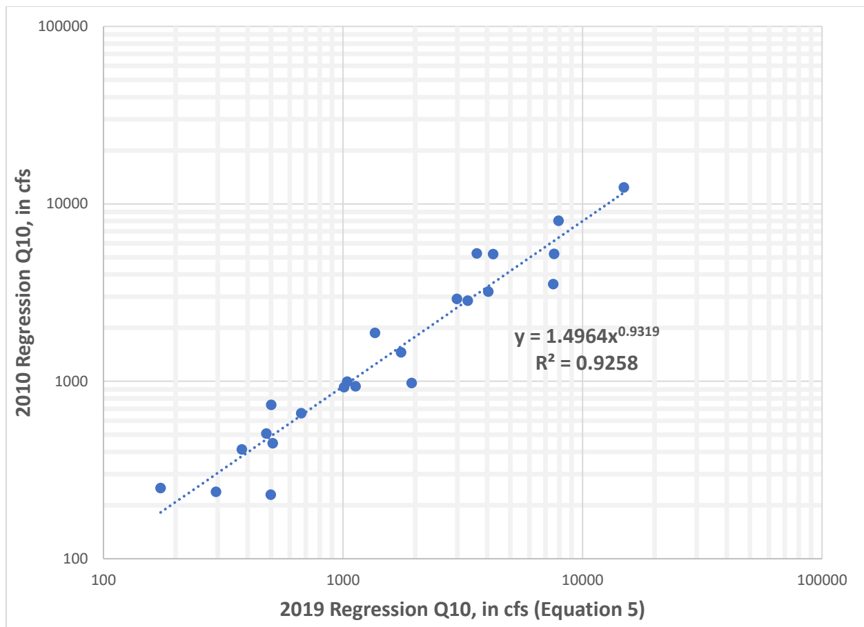
Figure 8. Comparison of the 10-year flood discharges for the 2010 and 2019 regression equations.
