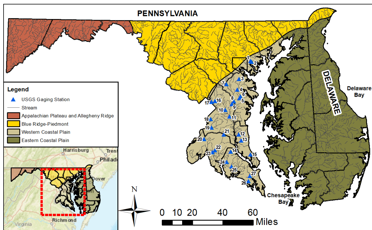
Figure 1. Location of 27 gaging stations in the Western Coastal Plain Region.
