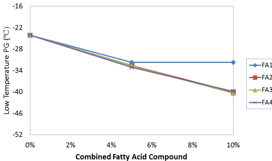
Figure 17. Impact of Combined Fatty Acid Compound on Low Temperature PG.
