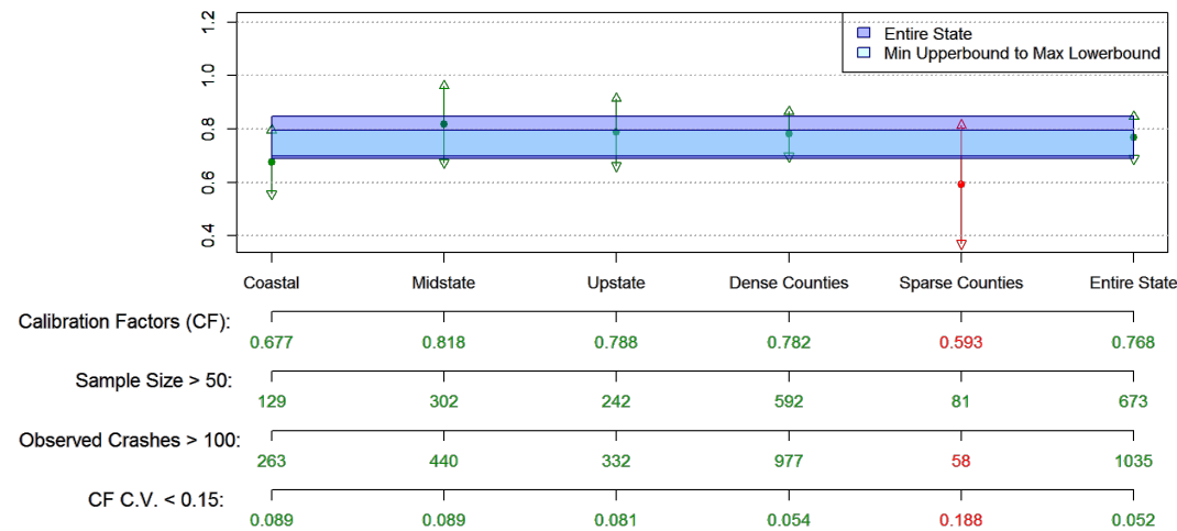
Figure 7.12 UST Calibration factor summary 2013:2015
