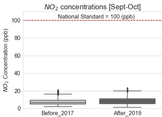
Figure 10 - Average Daily NO 2 Concentrations
