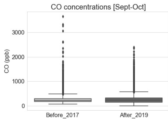
Figure 11 - Average Daily CO Concentrations
