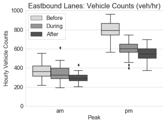
Figure 4 - Eastbound Traffic Volumes
