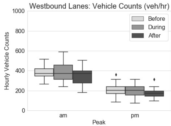
Figure 5 - Westbound Traffic Volumes
