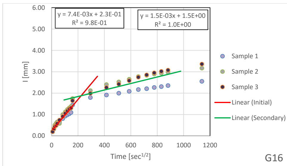
Figure B.1.34 – Absorption Results for G16
