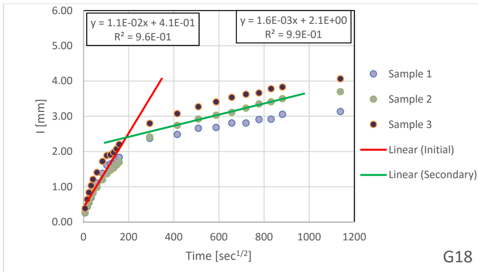
Figure B.1.36 – Absorption Results for G18
