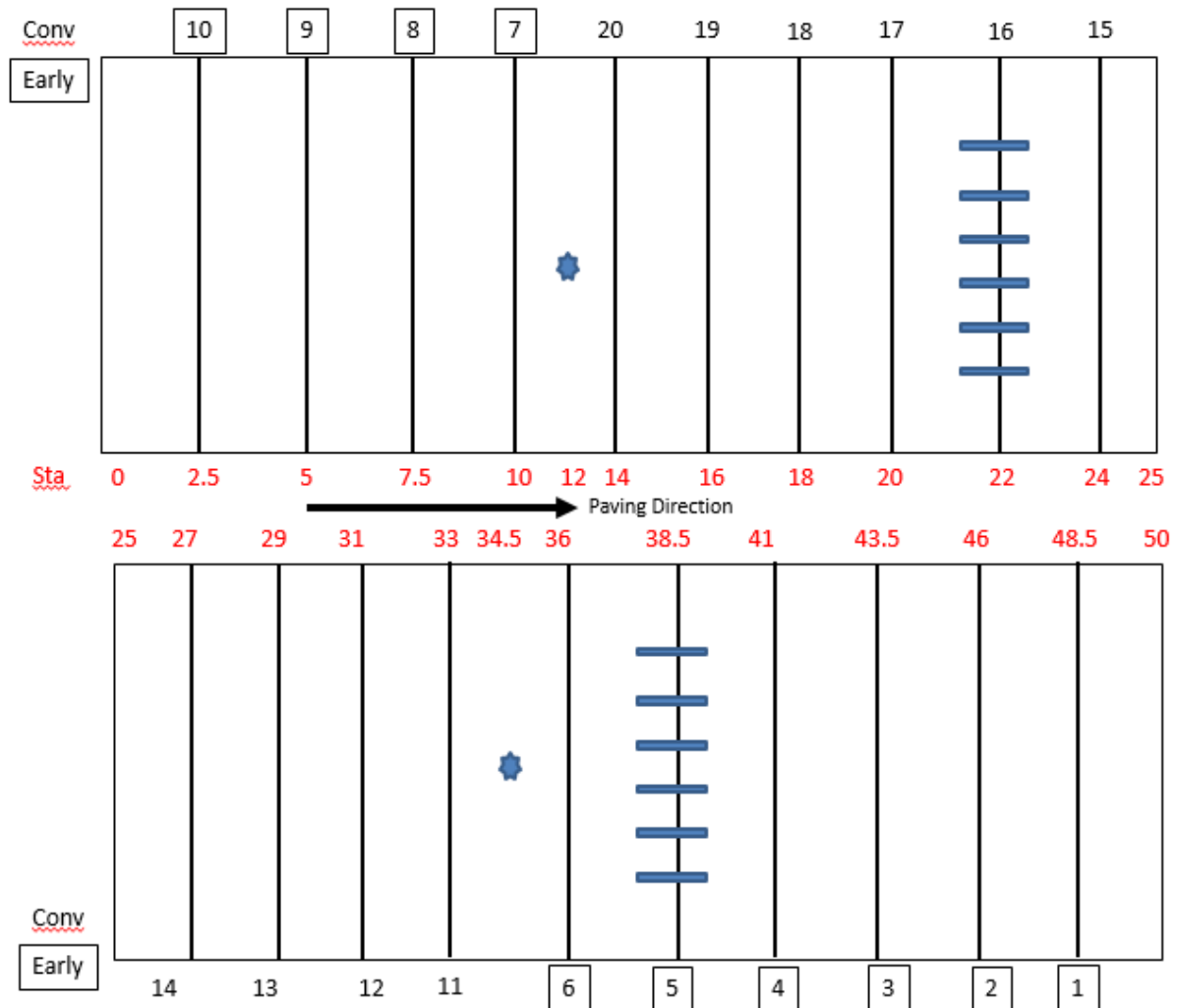
Figure 2.4.1. Layout Sketch of Saw Cut Joints Within Each Mixture Type (Note: Conv = Conventional Wet Saw Cut)
