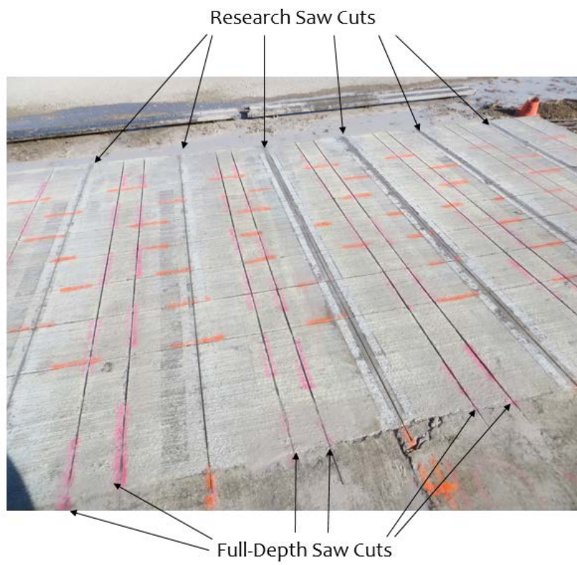
Figure 2.6.3. Full-Depth Sawing Pattern
