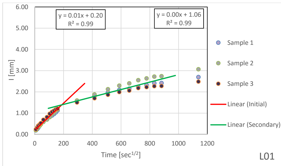
Figure B.1.1 – Absorption Results for L01
