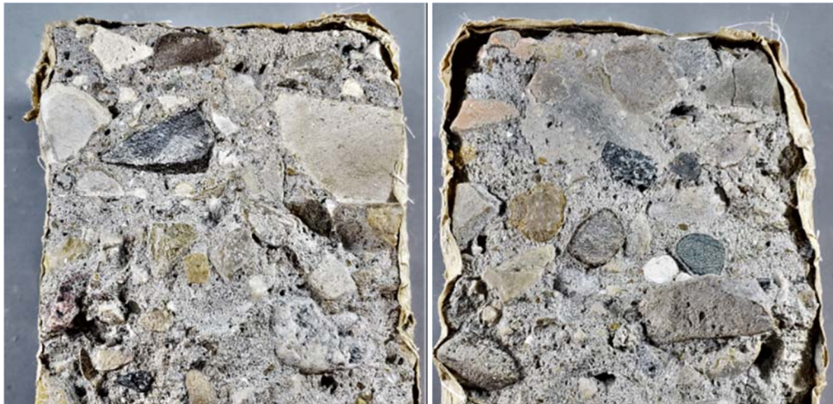
Figure 4.7.3. Samples with 1.5 in. Sawn Face Unsealed (left) and Sealed (right)
