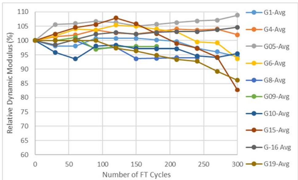
Figure 4.4.8. Granite Freeze-Thaw Results Reported for Relative Dynamic Modulus through 300 cycles
