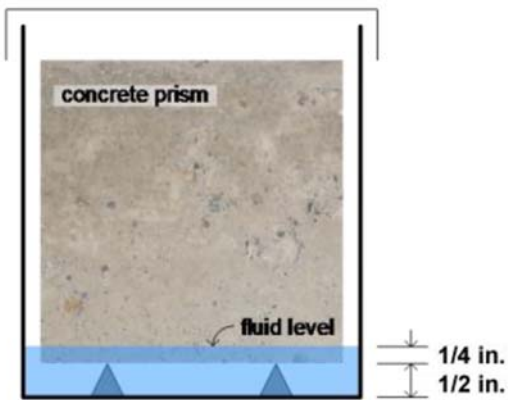
Figure 3.4.1. Schematic Diagram of the Modified Freeze-Thaw Test Employed on the Core Samples
