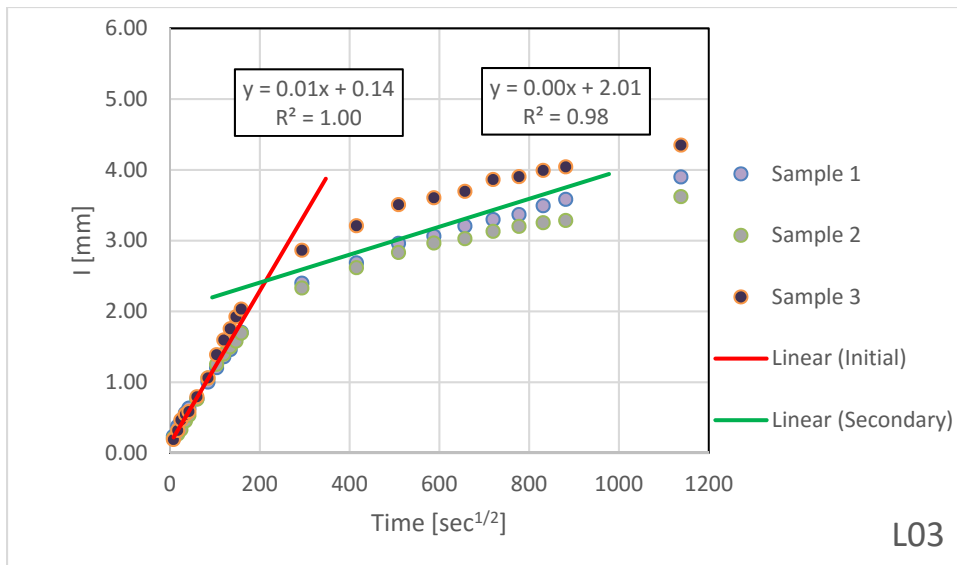
Figure B.1.3 – Absorption Results for L03
