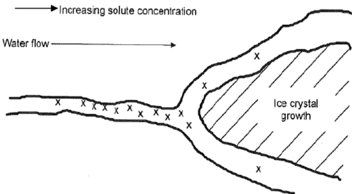
Figure 1.7.3. Conceptual Illustration of the Generation of Osmotic Pressure in Concrete Pores (Zhang, 2013)
