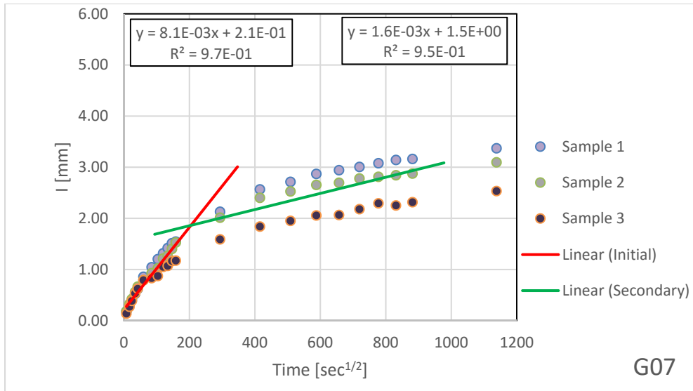
Figure B.1.26 – Absorption Results for G07
