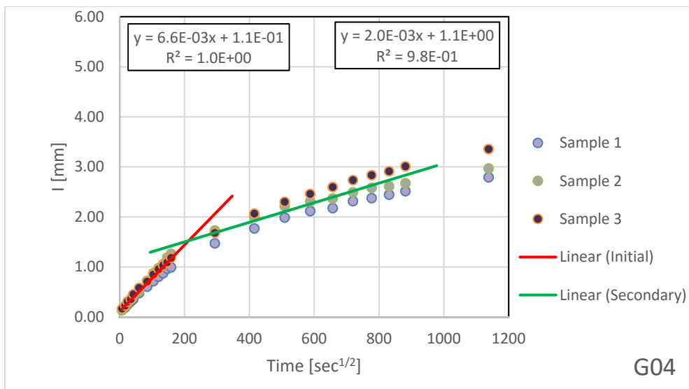
Figure B.1.23 – Absorption Results for G04
