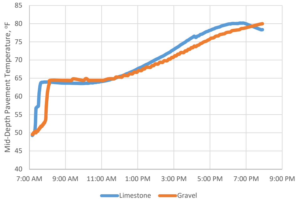
Figure 2.5.13. Mid-Temp Temperature Probe Readings After Paving
