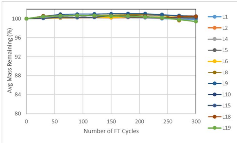
Figure 4.4.3. Limestone Freeze-Thaw Results Reported for Mass through 300 cycles
