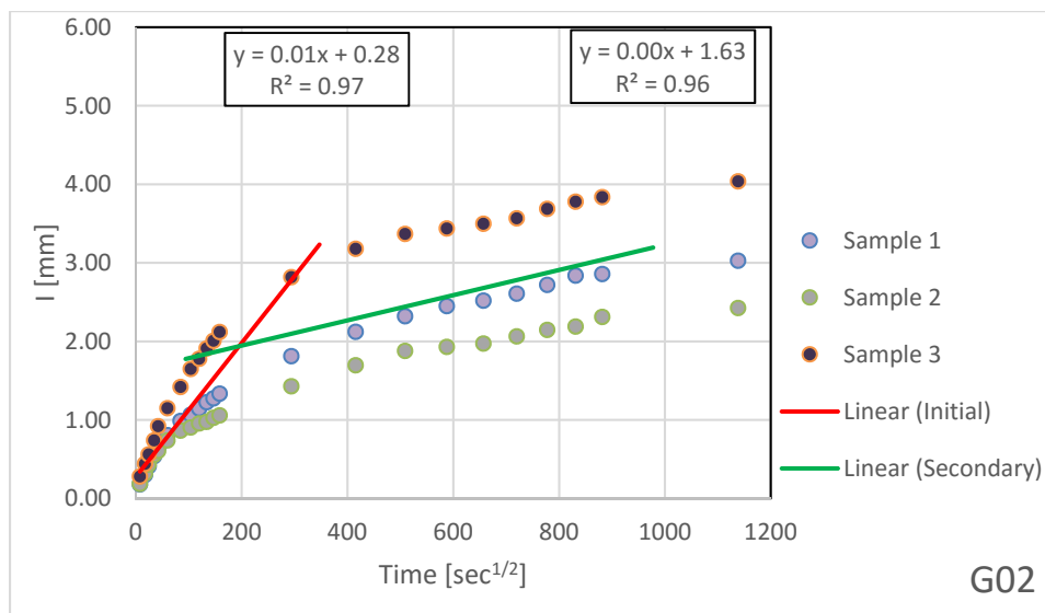
Figure B.1.21 – Absorption Results for G02
