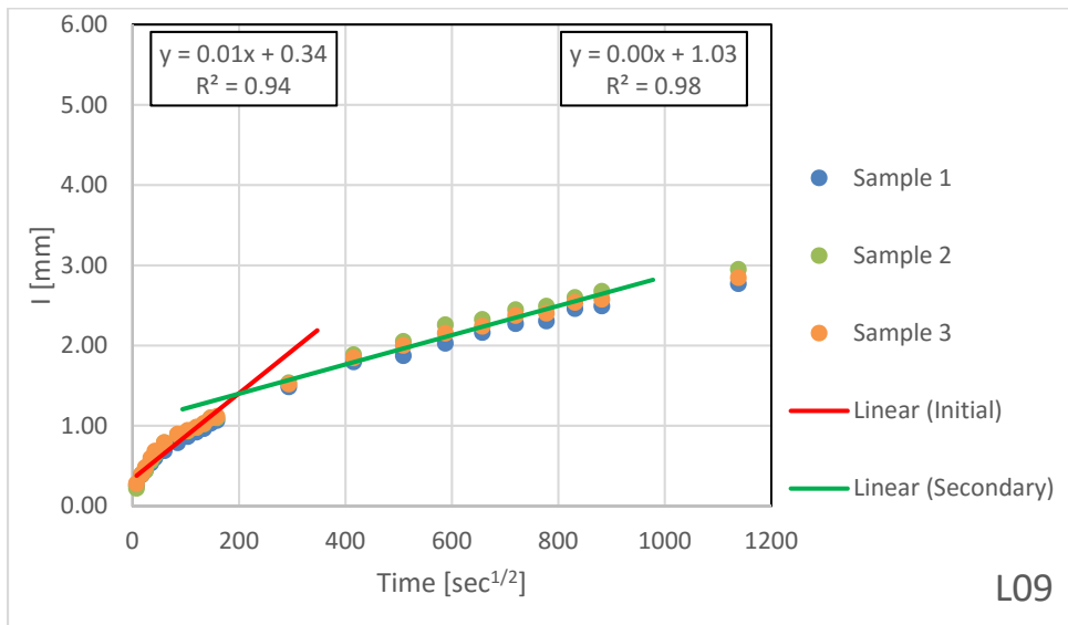
Figure B.1.9 – Absorption Results for L09
