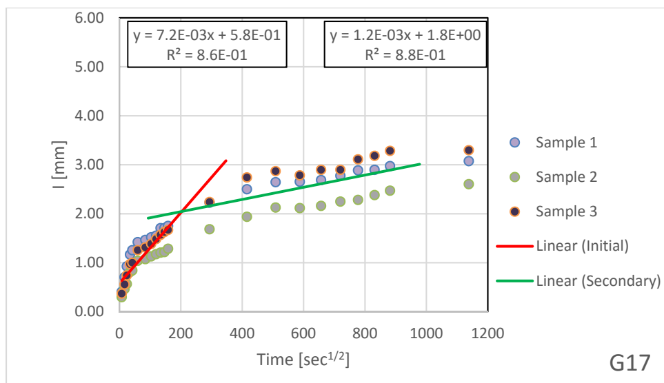
Figure B.1.35 – Absorption Results for G17
