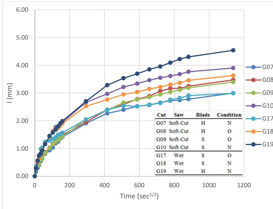
Figure 4.3.16. Absorption Results for Late Sawing Window for the Granite Aggregate Mixture
