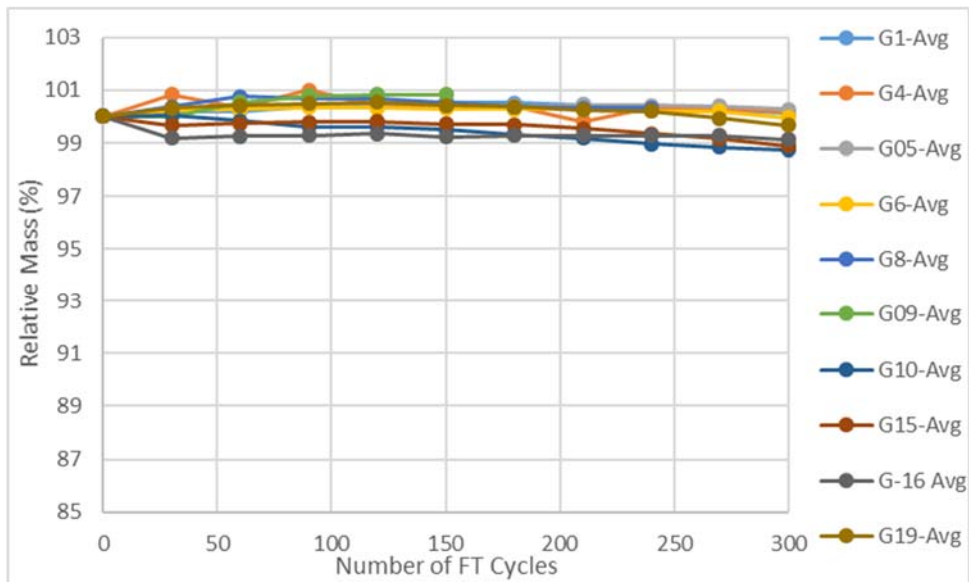
Figure 4.4.7. Granite Freeze-Thaw Results Reported for Mass through 300 cycles
