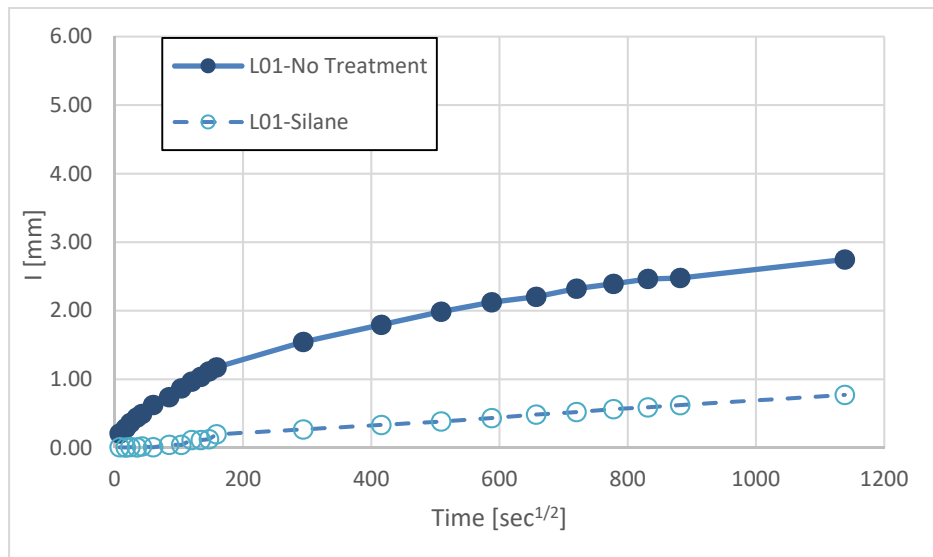
Figure 4.3.8. Absorption Results for L01 – Soft Cut Saw, Early Sawing Window, New Limestone Blade -Before and After Coating with Silane
