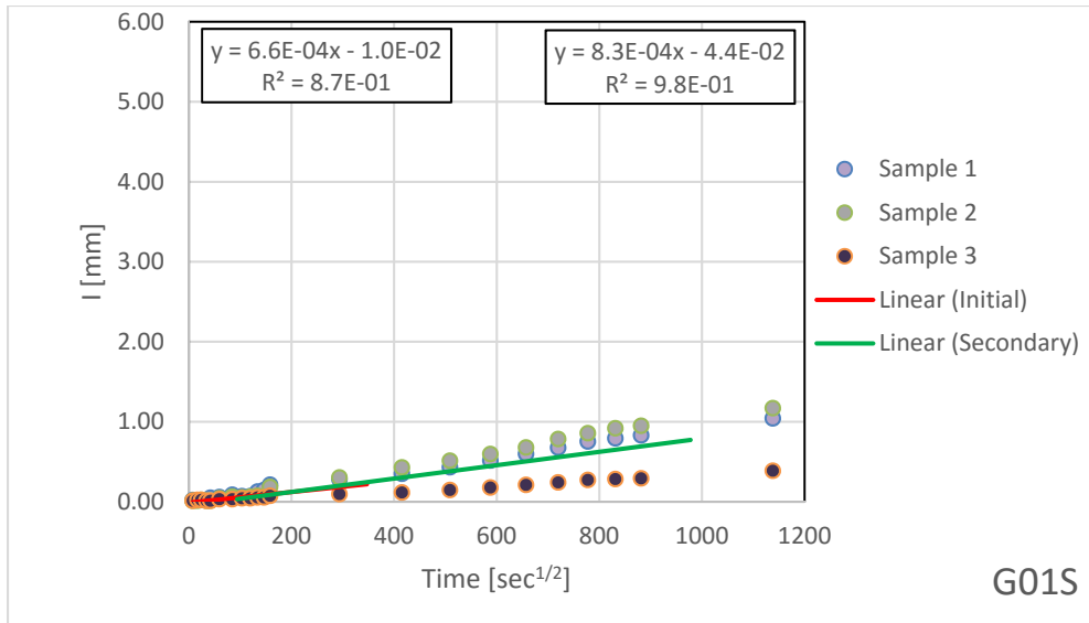
Figure B.1.38 – Absorption Results for G01-Silane Coated
