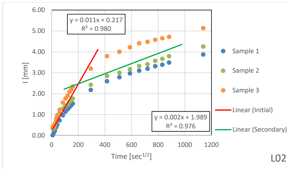
Figure 4.3.2. Absorption Results for L02 – Soft Cut Saw, Early Sawing Window, Old Limestone Blade
