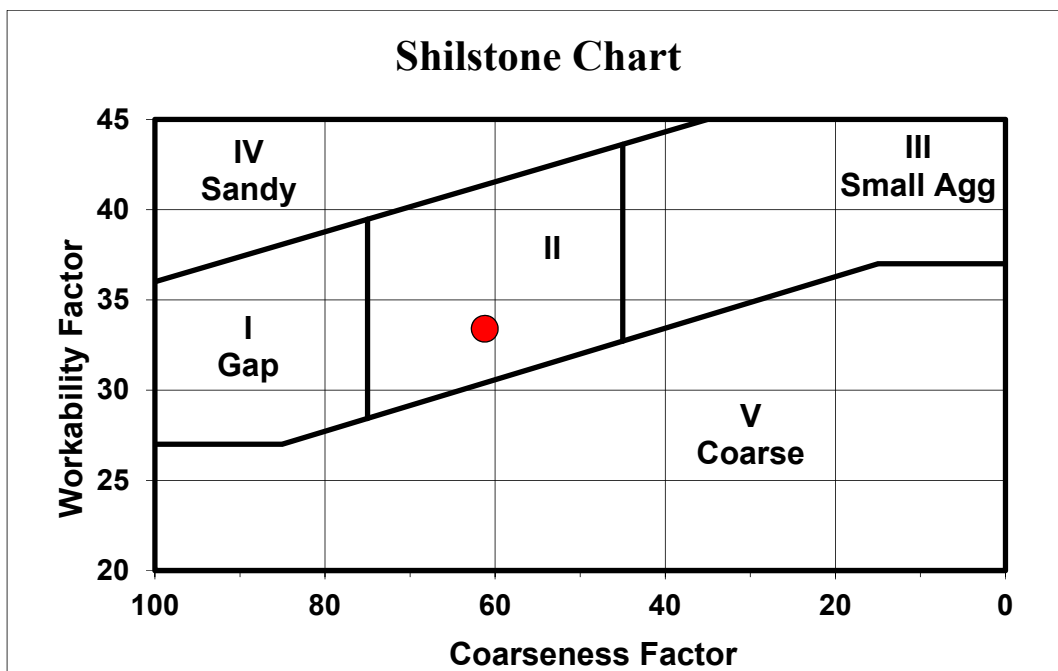
Figure 2.8.3. Coarseness Factor Analysis – CTH KC EB On-Ramp Mixture
