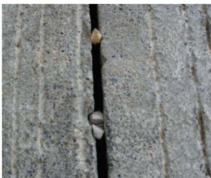
Figure 1.2.4. Incompressible Materials Causing Mechanical Damage, which can Lead to Further Distress (Taylor, et al. 2012b)
