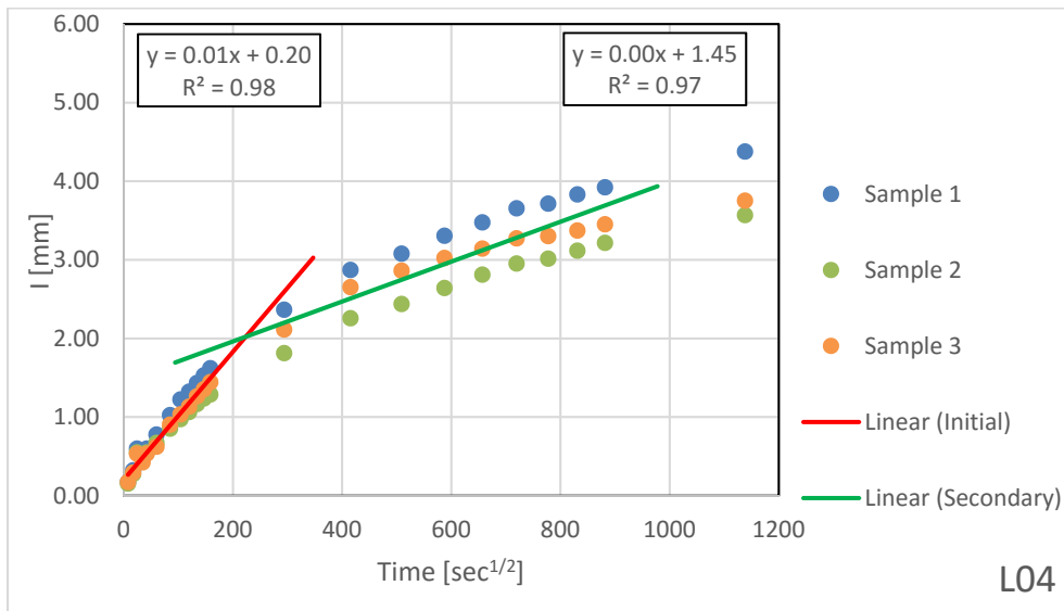
Figure B.1.4 – Absorption Results for L04
