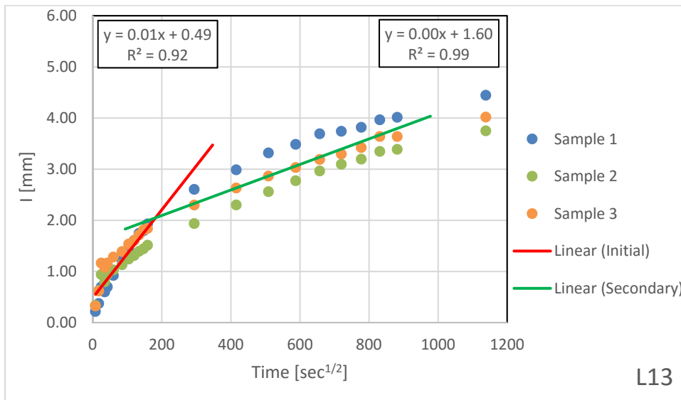
Figure B.1.13 – Absorption Results for L13
