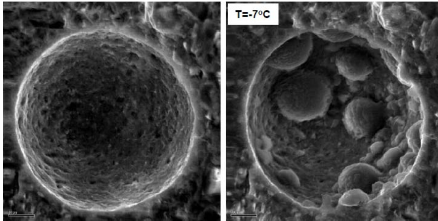
Figure 1.10.2. SEM Image of Air Void Before and After Freezing Occurs in Concrete (Zhang, 2013)
