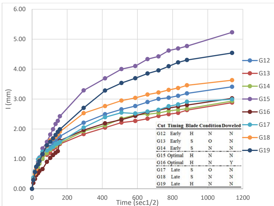
Figure 4.3.14. Absorption Results for Conventional Sawing of the Granite Aggregate Mixture
