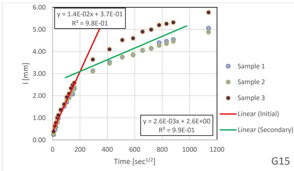
Figure B.1.33 – Absorption Results for G15
