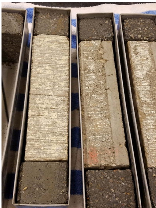
Figure 3.3.2. Freeze-Thaw Testing Setup
