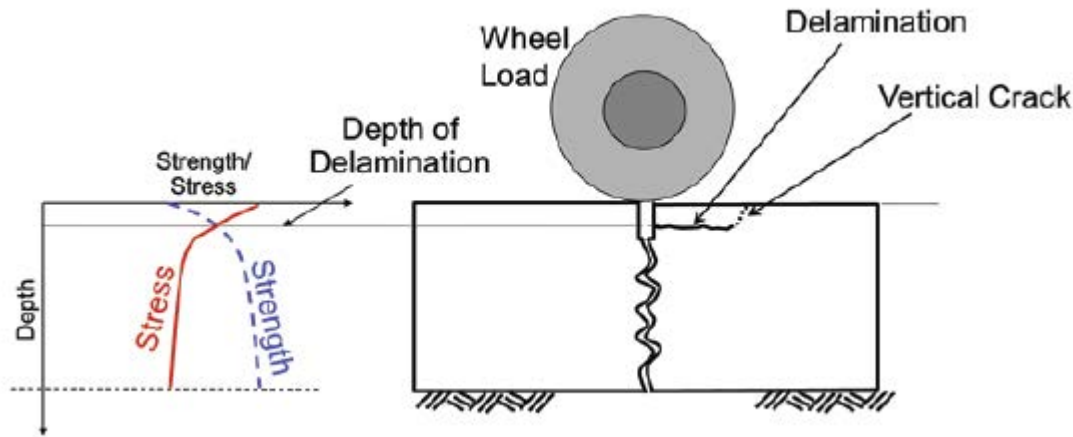
Figure 1.2.7. Early-Age Drying Stresses (left) and Resulting Vertical Cracking and Delamination Spalling (right) due to High Moisture Loss During Placement (Spragg et al., 2011)
