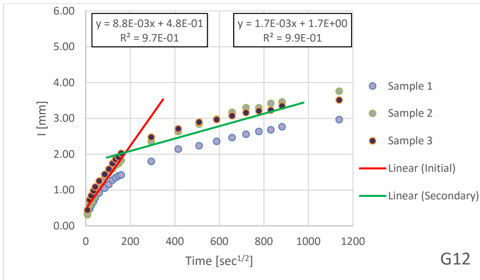
Figure B.1.30 – Absorption Results for G12
