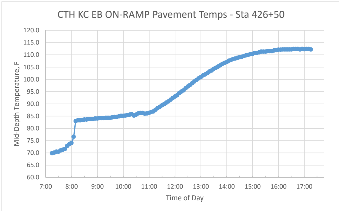
Figure 2.10.9. Mid-Temp Temperature Probe Readings After Paving
