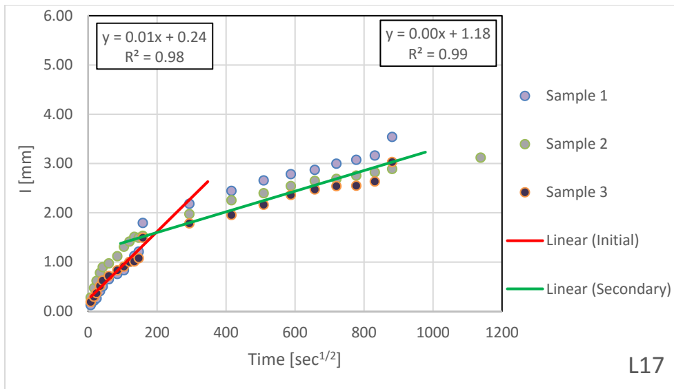
Figure B.1.16 – Absorption Results for L17
