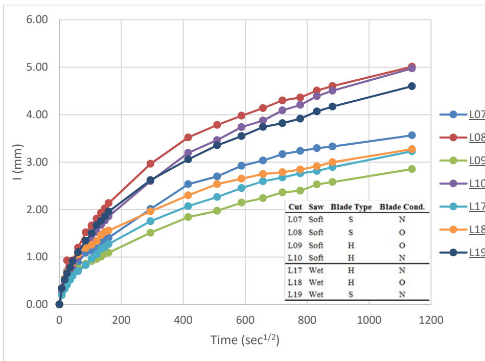
Figure 4.3.7. Comparison of Results for Late Slicing in the Timing Window of the Limestone Aggregate Mixture
