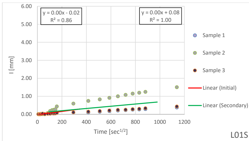
Figure B.1.19 – Absorption Results for L01 Silane-Coated
