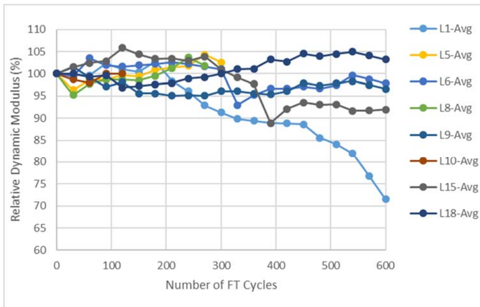
Figure 4.4.6. Limestone Freeze-Thaw Results Reported for Relative Dynamic Modulus through 600 cycles
