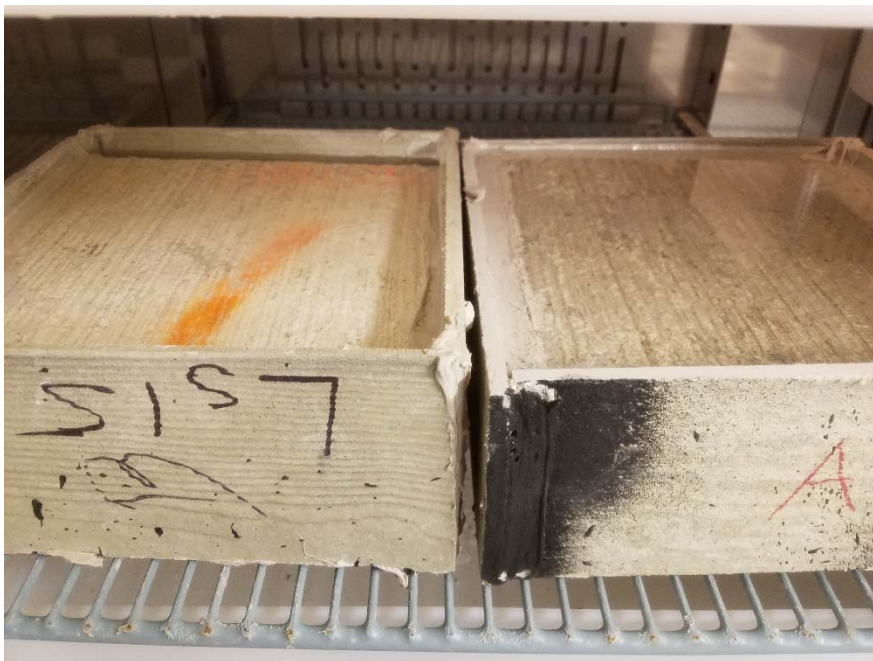
Figure 3.5.2. Deicer Testing with Silane (left) and Uncoated (right) Samples
