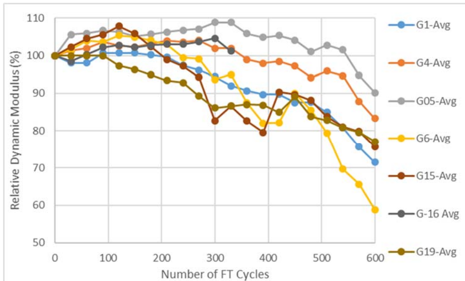
Figure 4.4.10. Granite Freeze-Thaw Results Reported for Relative Dynamic Modulus Through 600 Cycles
