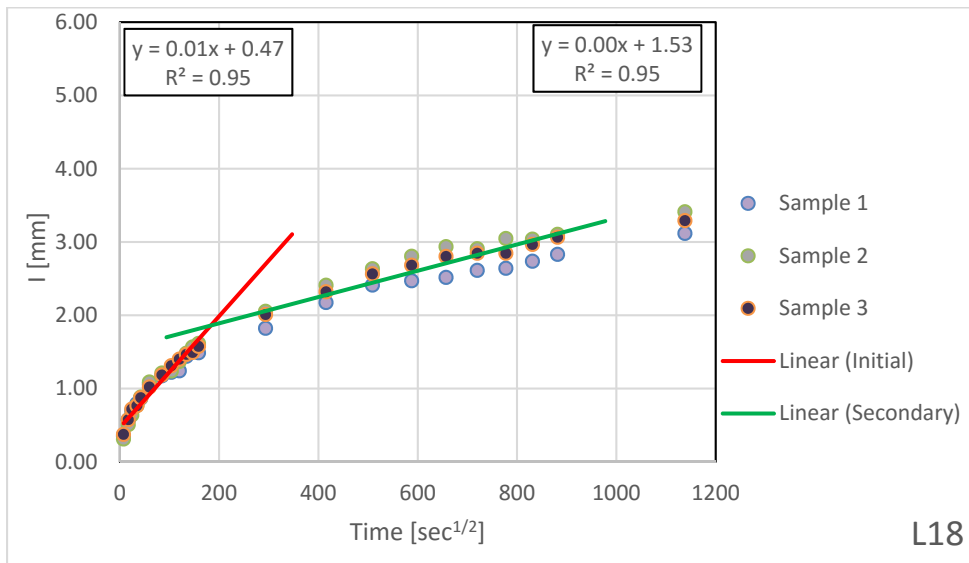
Figure B.1.17 – Absorption Results for L18
