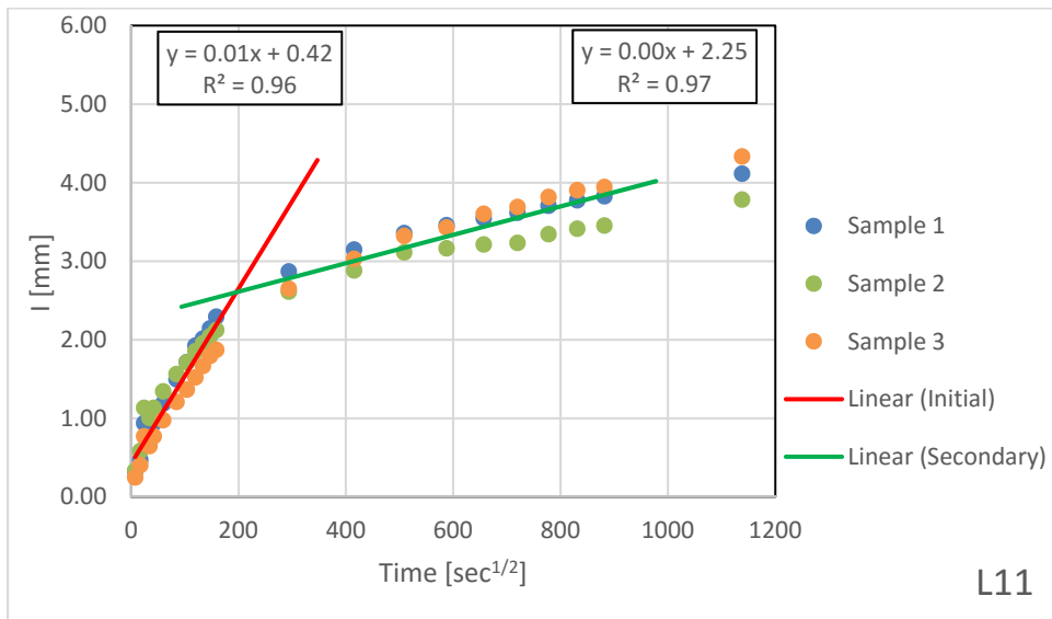
Figure B.1.11 – Absorption Results for L11
