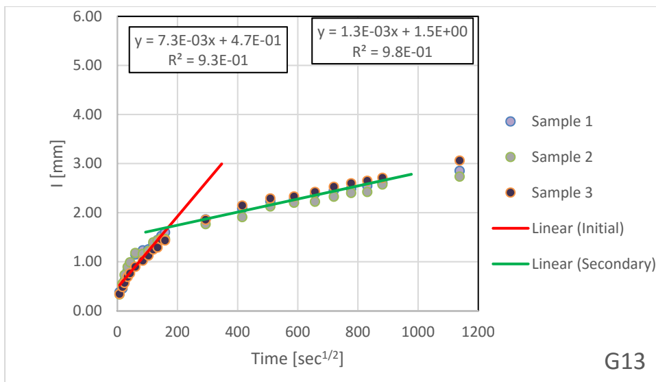
Figure B.1.31 – Absorption Results for G13
