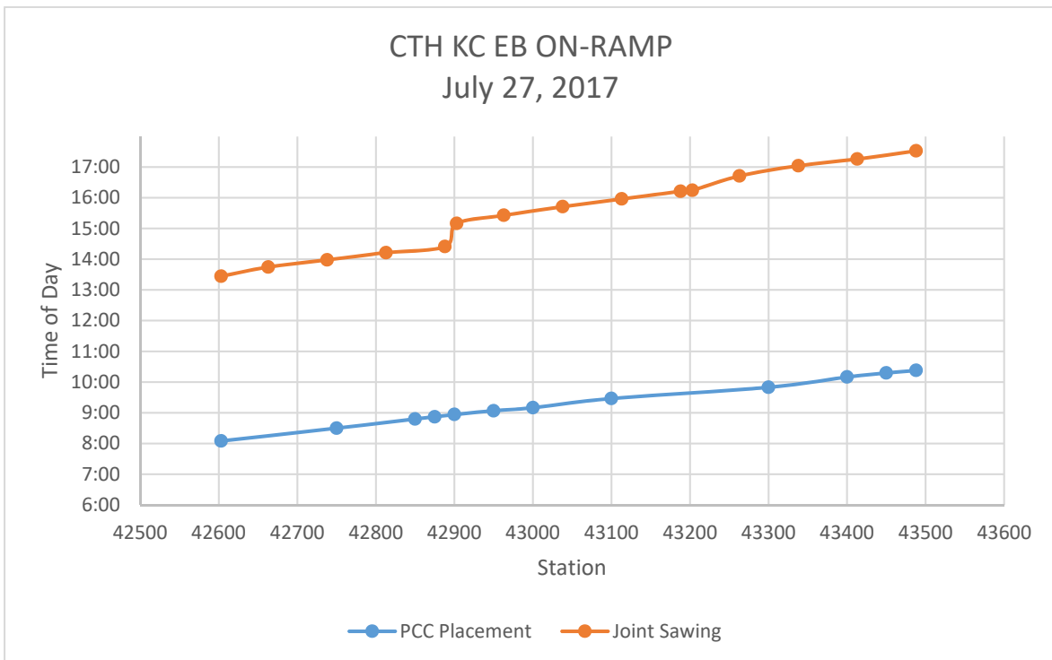
Figure 2.10.10. PCC Placement and Saw Cut Timing
