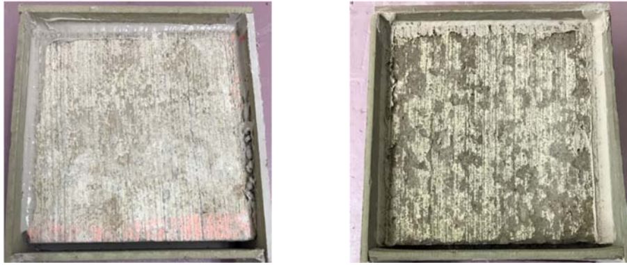
Figure 4.5.2. The Worst Performing Limestone Mixture (L16) Before (left) and After (right) 50 Deicer Cycles
