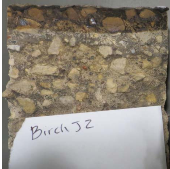
Figure 5.7.1. Typical Transverse Core Specimen After Cleaning (Birch J2)
