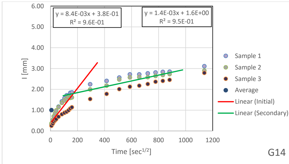
Figure B.1.32 – Absorption Results for G14
