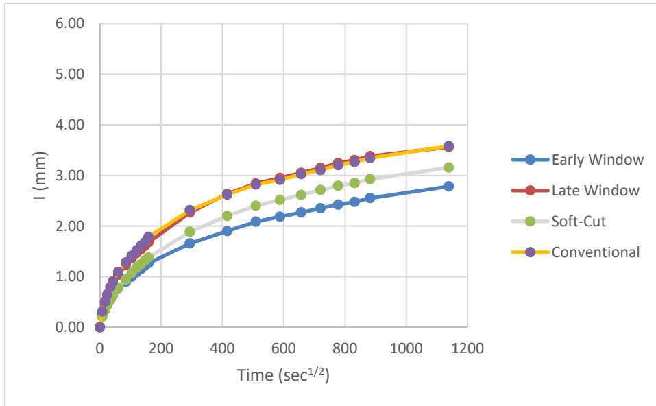
Figure 4.3.12. Average Absorption Results for All Granite Permutations Across Equipment and Timing
