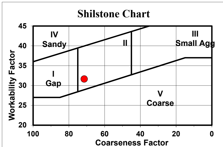
Figure 2.3.6. Coarseness Factor Analysis – Gravel Mixture
