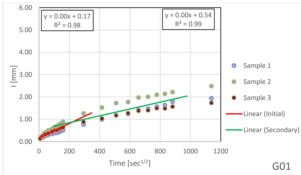
Figure B.1.20 – Absorption Results for G01
