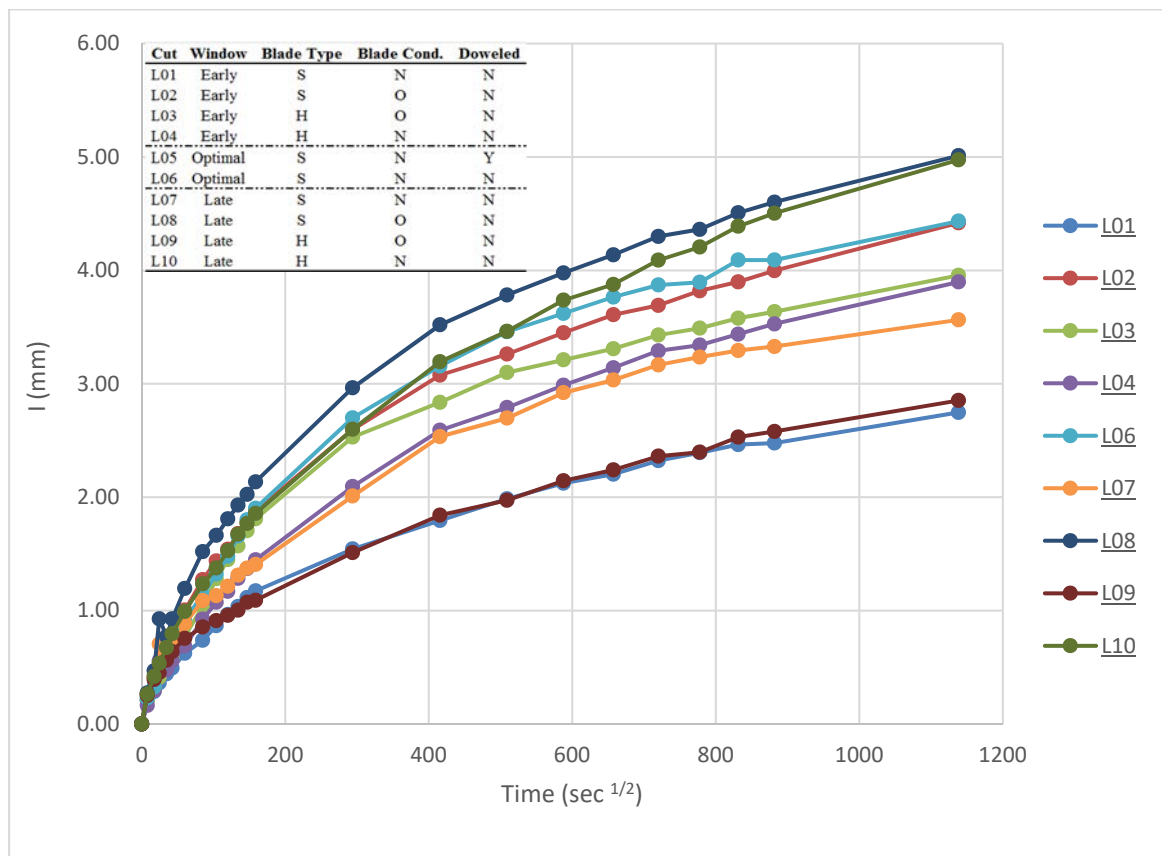
Figure 4.3.4. Comparison of Results for Soft-Cut Sawing of the Limestone Aggregate Mixture
