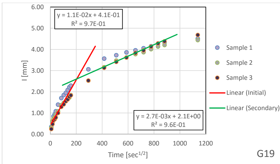
Figure B.1.37 – Absorption Results for G19
