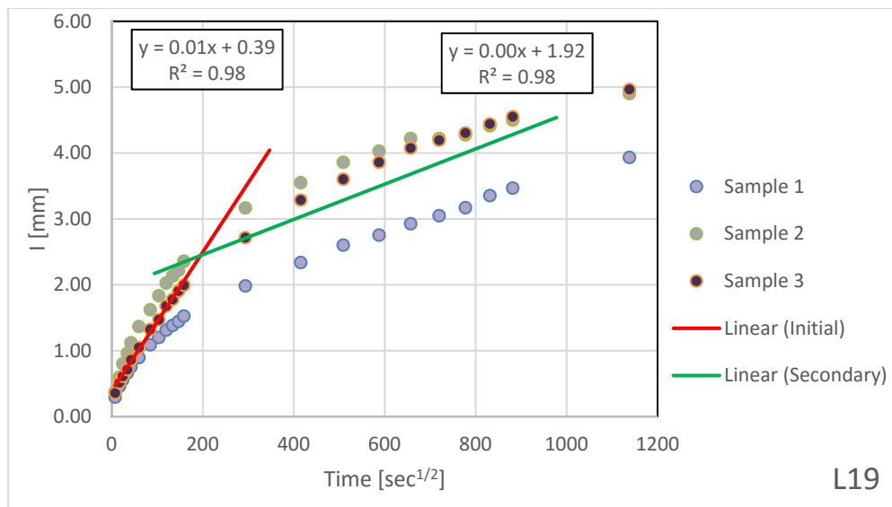
Figure B.1.18 – Absorption Results for L19
