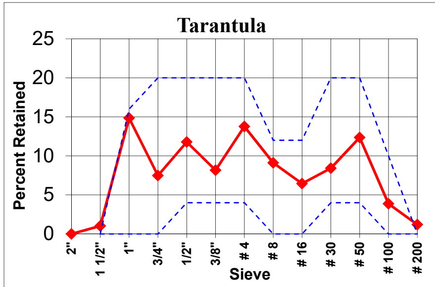
Figure 2.3.2. Combined Aggregate Analysis – Limestone Mixture
