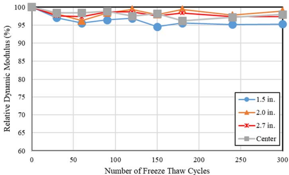
Figure 4.7.2. Freeze-Thaw Results Grouped by Depth of Sawing
