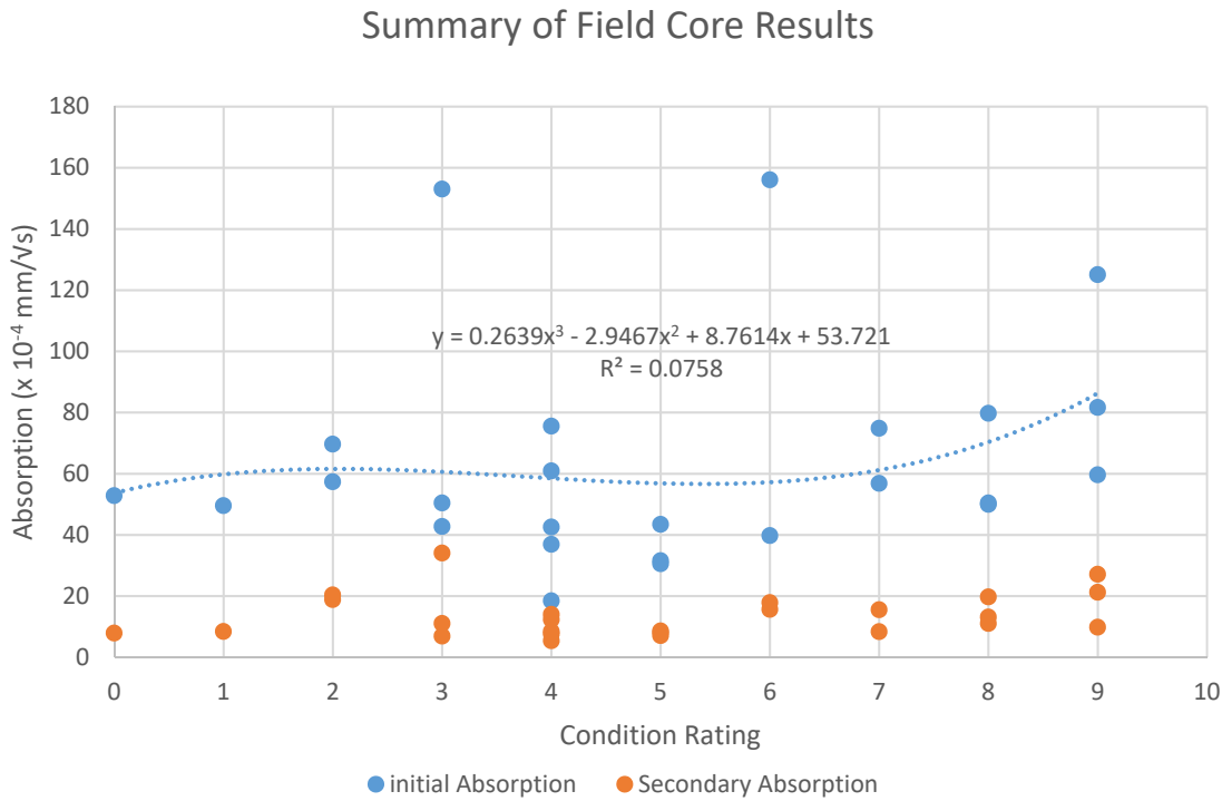
Figure 5.7.3. Absorption Rates versus Visual Joint Condition Ratings
