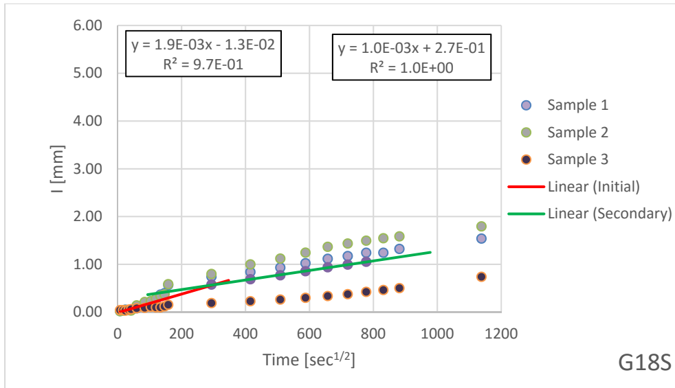
Figure B.1.40 – Absorption Results for G18-Silane Coated
