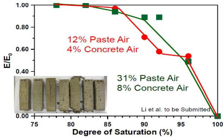
Figure 1.7.2. Relationship Between Degree of Saturation and Freeze-Thaw Durability (Li, et.al, 2012)
