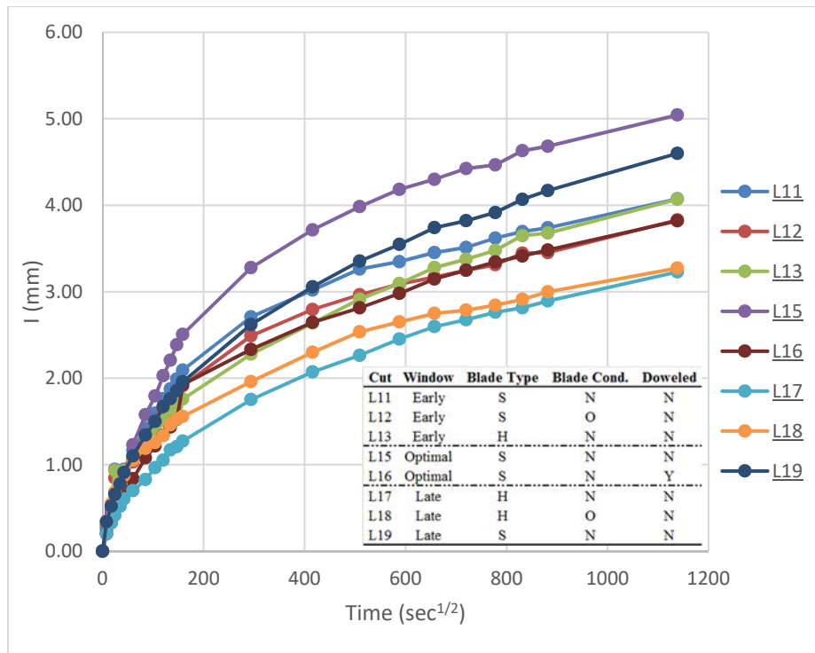
Figure 4.3.5. Comparison of Results for Conventional Sawing of the Limestone Aggregate Mixture
