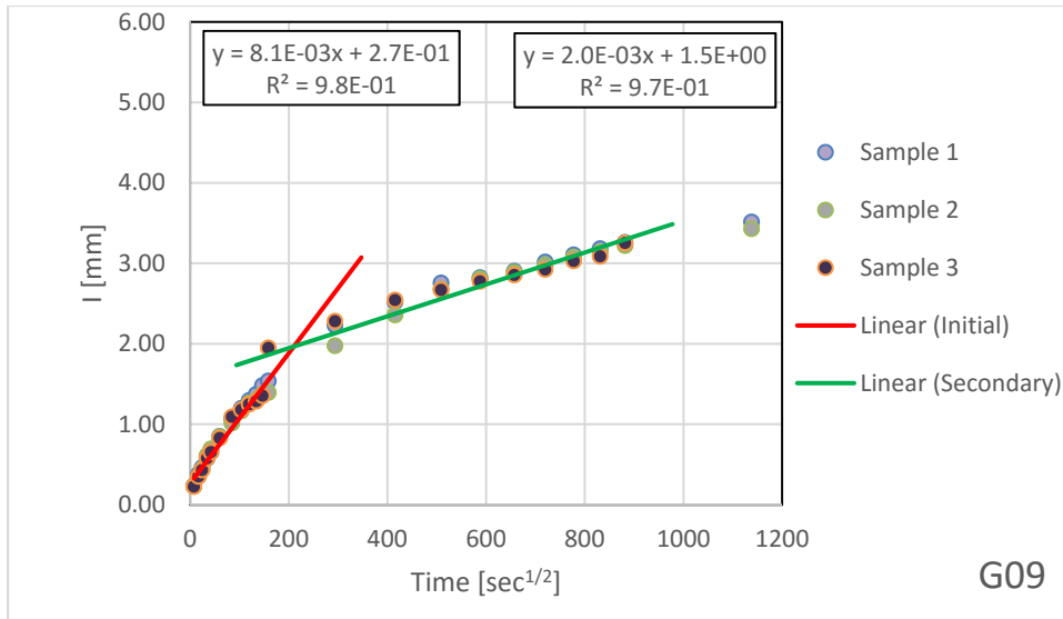
Figure B.1.28 – Absorption Results for G09
