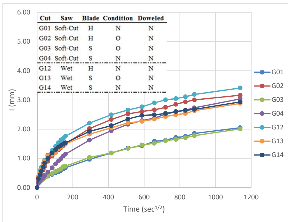
Figure 4.3.15. Absorption Results for Early Sawing Window for the Granite Aggregate Mixture
