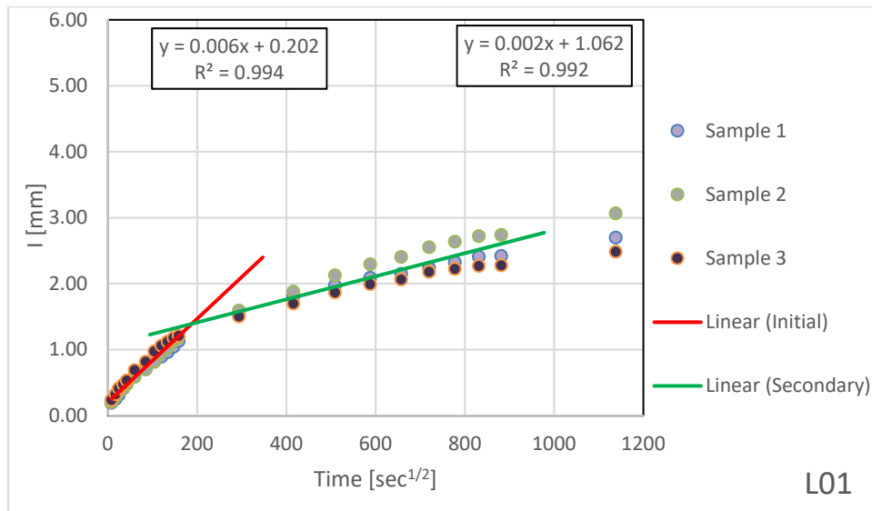
Figure 4.3.1. Absorption Results for L01 – Soft Cut Saw, Early Sawing Window, New Limestone Blade
