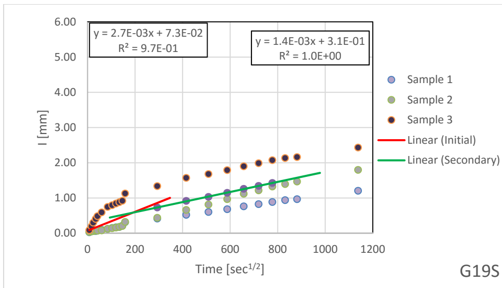
Figure B.1.41 – Absorption Results for G19-Silane Coated
