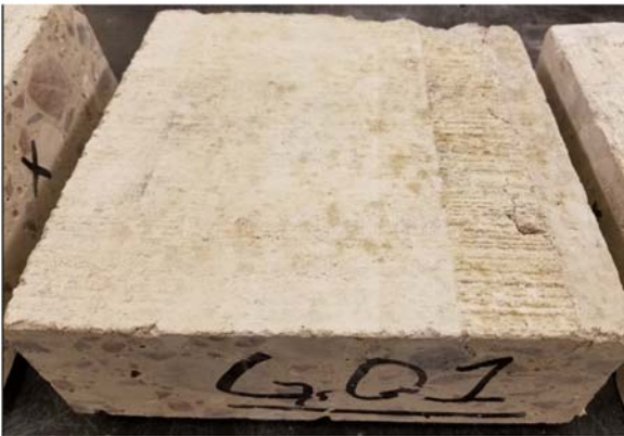
Figure 4.2.12. Joint Damage Observed for the Early Sawn Granite Samples
