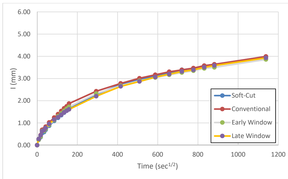
Figure 4.3.3. Average Performance Across Permutations for Equipment and Timing for the Limestone Aggregate
