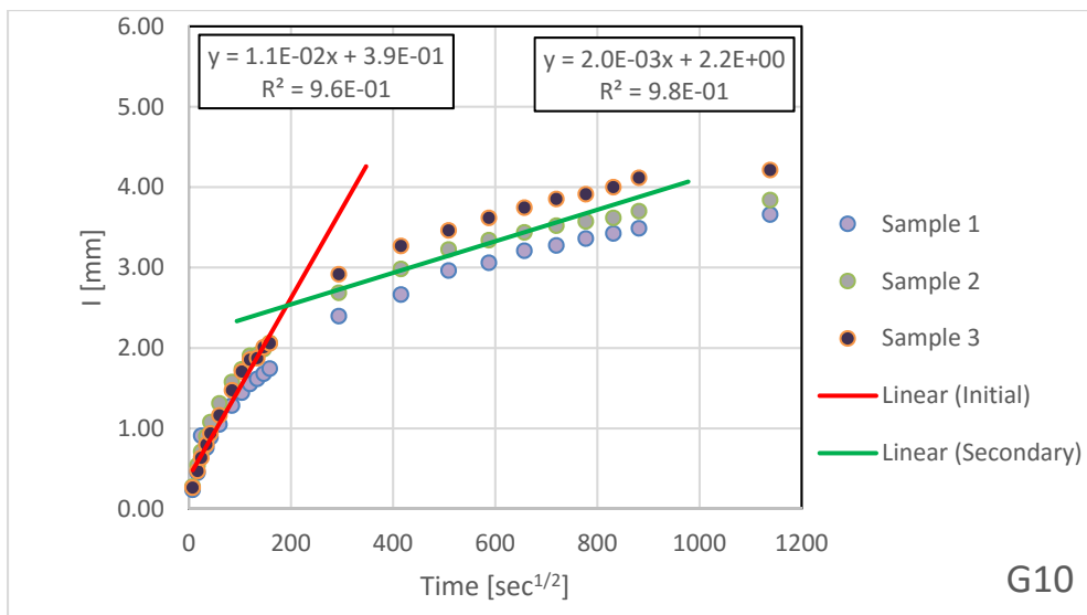
Figure B.1.29 – Absorption Results for G10
