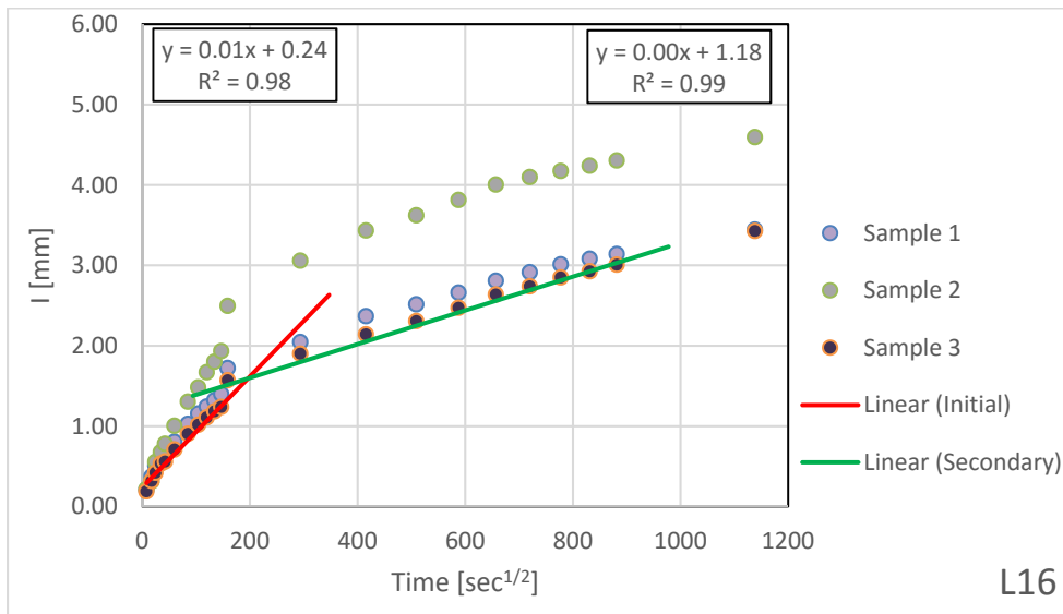
Figure B.1.15 – Absorption Results for L16
