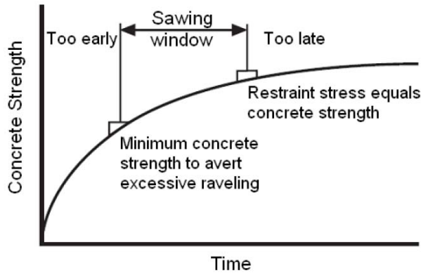
Figure 1.3.1. Concrete Sawing Window in Terms of Strength vs Time (Okamoto et al., 1994)
