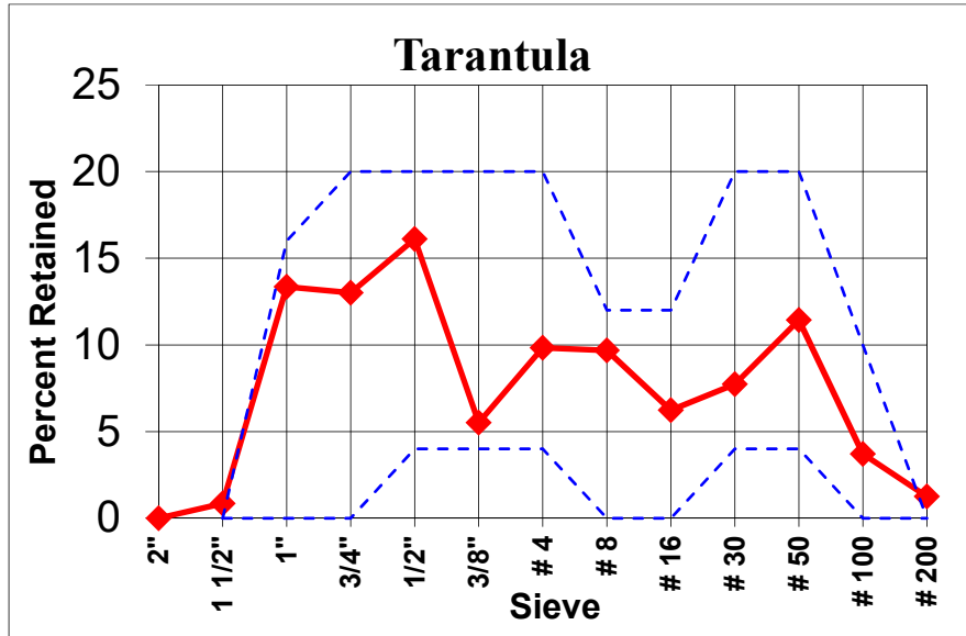
Figure 2.3.5. Combined Aggregate Analysis – Gravel Mixture
