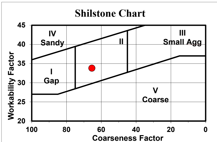
Figure 2.3.3. Coarseness Factor Analysis – Limestone Mixture
