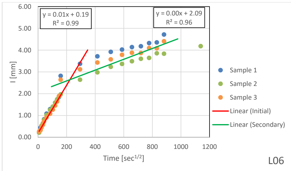
Figure B.1.6 – Absorption Results for L06
