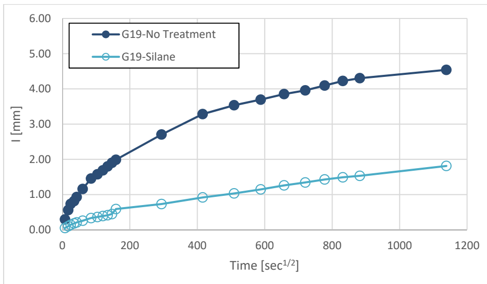
Figure 4.3.18. Absorption Results for G19 – Conventional Saw, Late Timing Window, New Granite Blade – Before and After Coating with Silane
