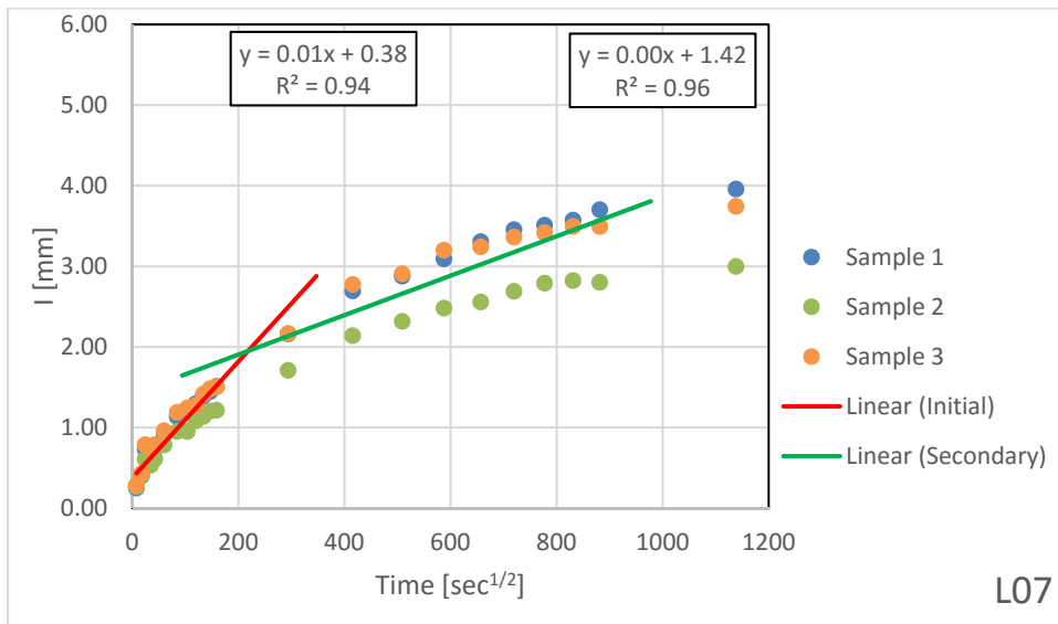
Figure B.1.7 – Absorption Results for L07
