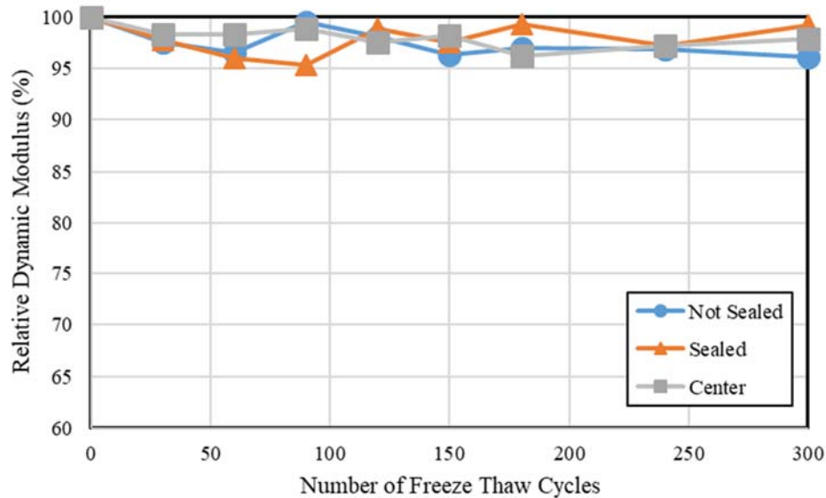
Figure 4.7.1. Freeze-Thaw Results Grouped by Treatment
