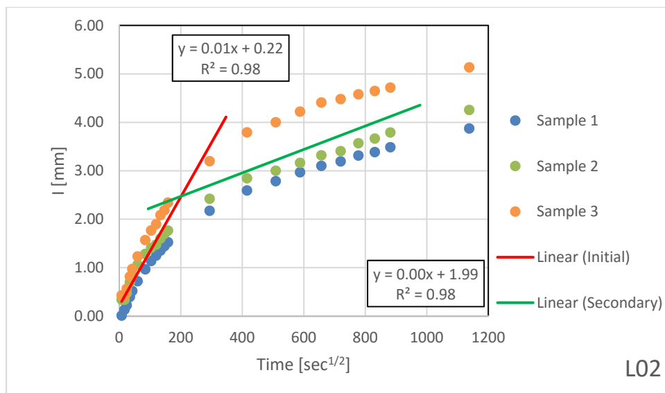
Figure B.1.2 – Absorption Results for L02
