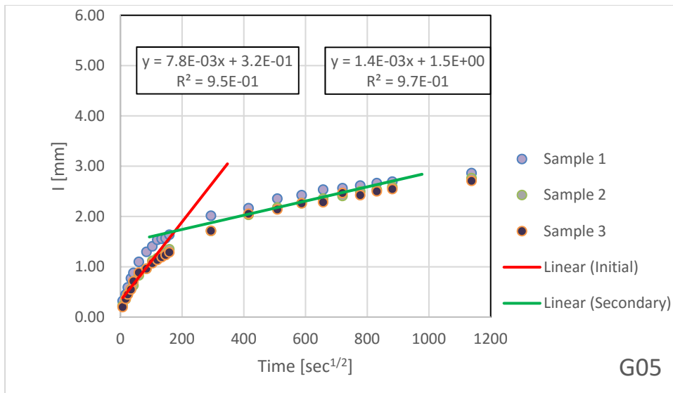
Figure B.1.24 – Absorption Results for G05
