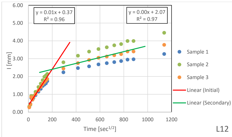
Figure B.1.12 – Absorption Results for L12
