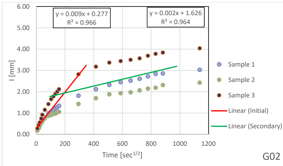
Figure 4.3.11. Absorption Results for G02 – Soft-Cut Saw, Early Timing Window, Old Granite Blade
