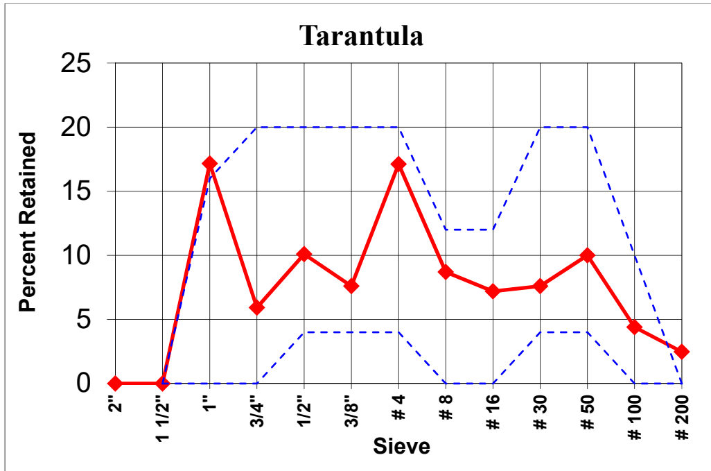
Figure 2.8.2. Combined Aggregate Analysis – CTH KC EB On-Ramp Mixture
