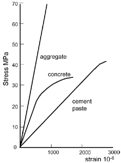
Figure 1.11.1. Comparative Stress Strain Curves for Aggregate, Paste and Concrete (Zhang, 2013)
