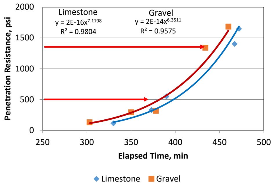
Figure 2.5.14. Resistance to Penetration Readings After Paving
