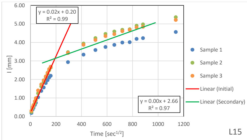
Figure B.1.14 – Absorption Results for L15
