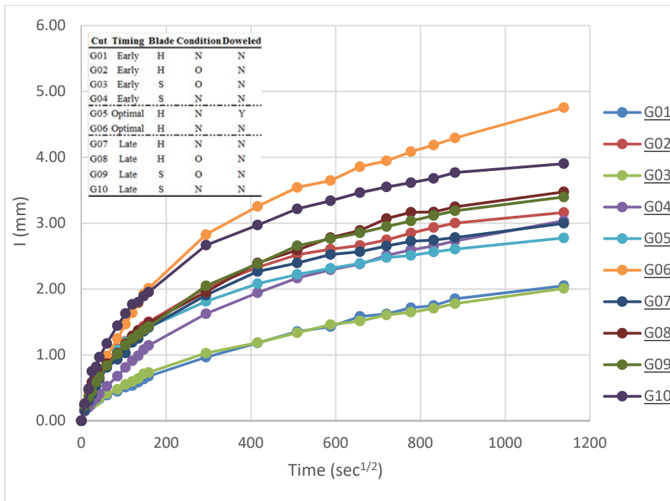
Figure 4.3.13. Absorption Results for Soft-Cut Sawing of the Granite Aggregate Mixture
