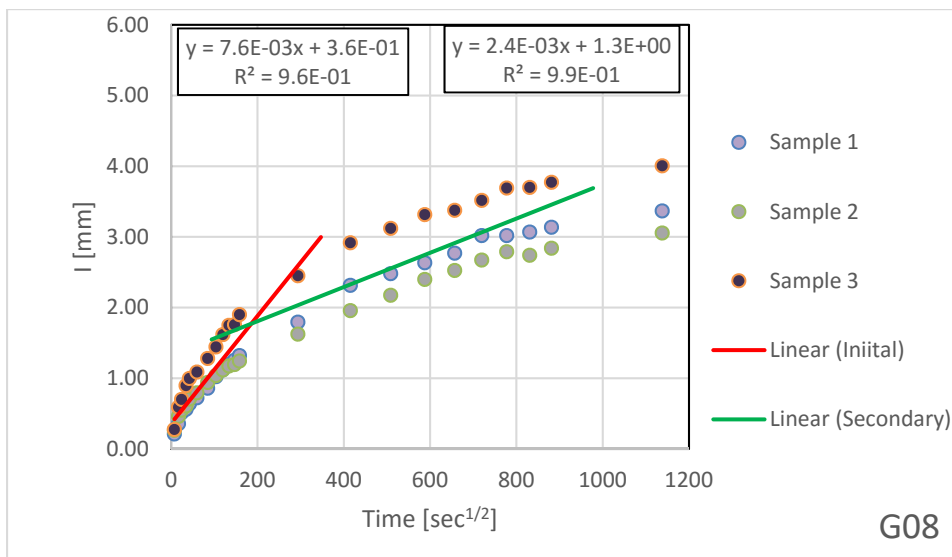
Figure B.1.27 – Absorption Results for G08
