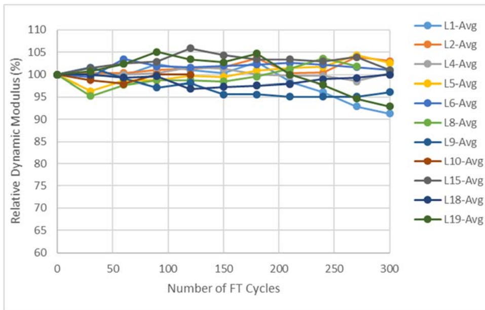
Figure 4.4.4. Limestone Freeze-Thaw Results Reported for Relative Dynamic Modulus through 300 cycles
