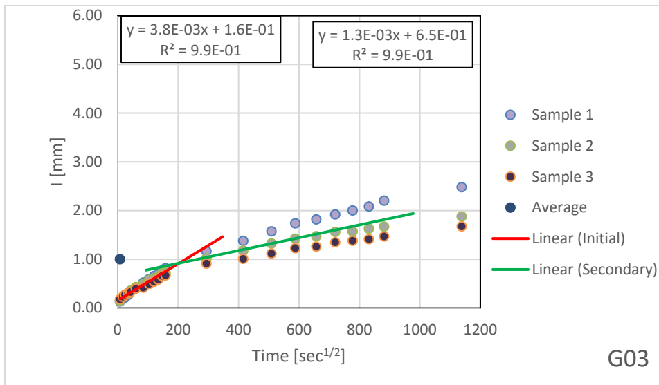
Figure B.1.22 – Absorption Results for G03
