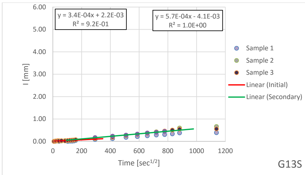
Figure B.1.39 – Absorption Results for G13-Silane Coated
