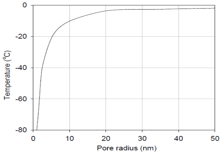
Figure 1.7.1. Relationship Between Capillary Pore Size and the Freeze Temperature (Zhang, 2013)
