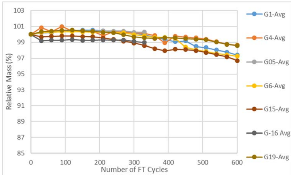
Figure 4.4.9. Granite Freeze-Thaw Results for Mass Through 600 Cycles
