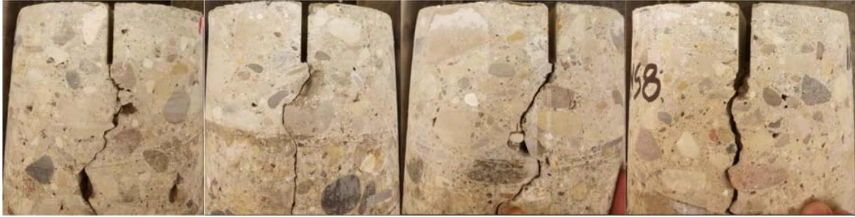
Figure 4.2.13. Core Samples Sawn to a Depth of 1.5 in.
