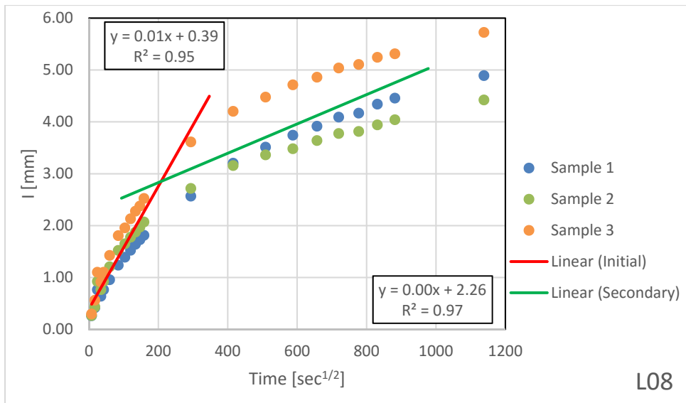
Figure B.1.8 – Absorption Results for L08
