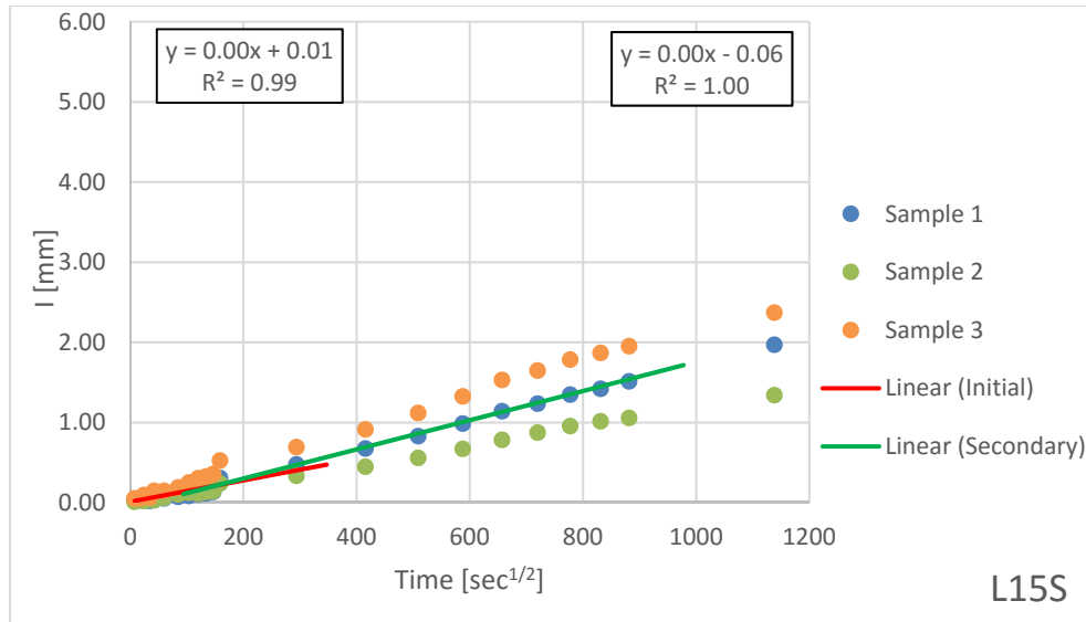
Figure B.1.19 – Absorption Results for L15 Silane-Coated
