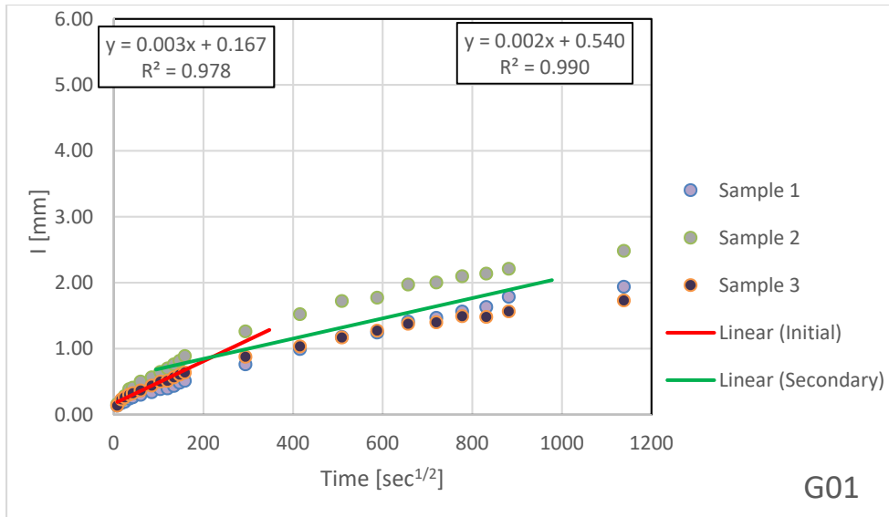
Figure 4.3.10. Absorption Results for G01 – Soft-Cut Saw, Early Timing Window, New Granite Blade
