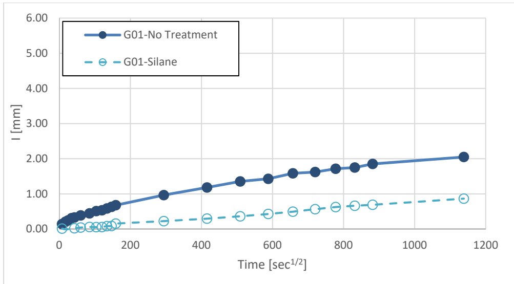
Figure 4.3.17. Absorption Results for G01 – Soft-Cut Saw, Early Timing Window, New Granite Blade – Before and After Coating with Silane
