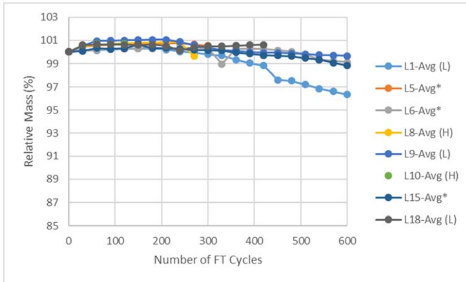
Figure 4.4.5. Limestone Freeze-Thaw Results Reported for Mass through 600 cycles
