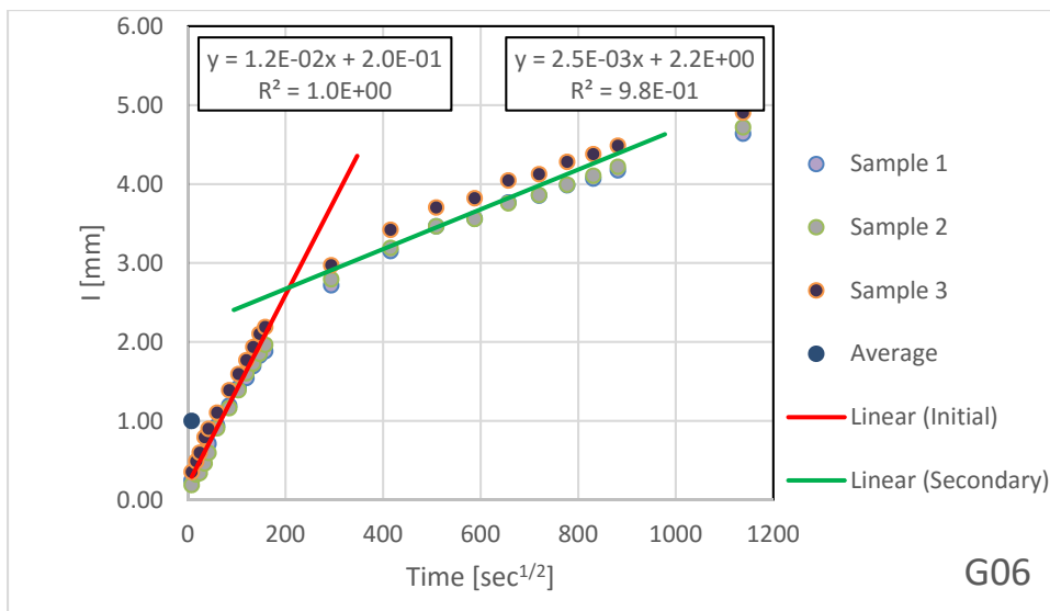
Figure B.1.25 – Absorption Results for G06
