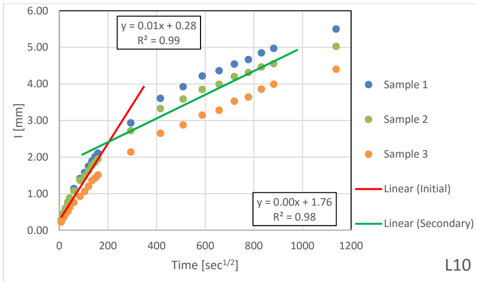
Figure B.1.10 – Absorption Results for L10
