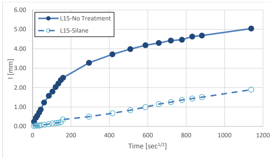
Figure 4.3.9. Absorption Results for L15 – Conventional Saw, Optimal Sawing Window, New Limestone Blade - Before and After Coating with Silane
