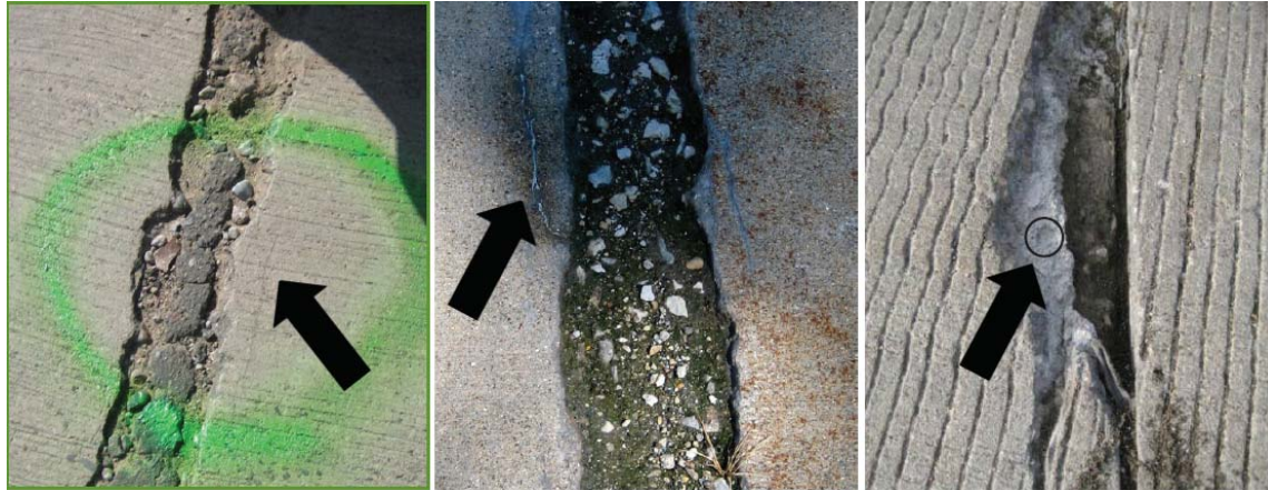
Figure 1.2.3. Incremental Cracking: Note (left to right) the crack parallel to the already patched face, the signs of water passing through the crack, and the exposed aggregate remaining in the concrete (Taylor et al., 2012a)
