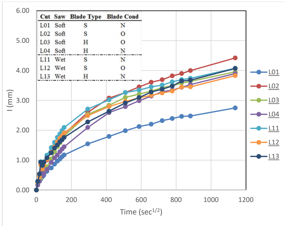
Figure 4.3.6. Comparison of Results for Early Slicing in the Timing Window of the Limestone Aggregate Mixture
