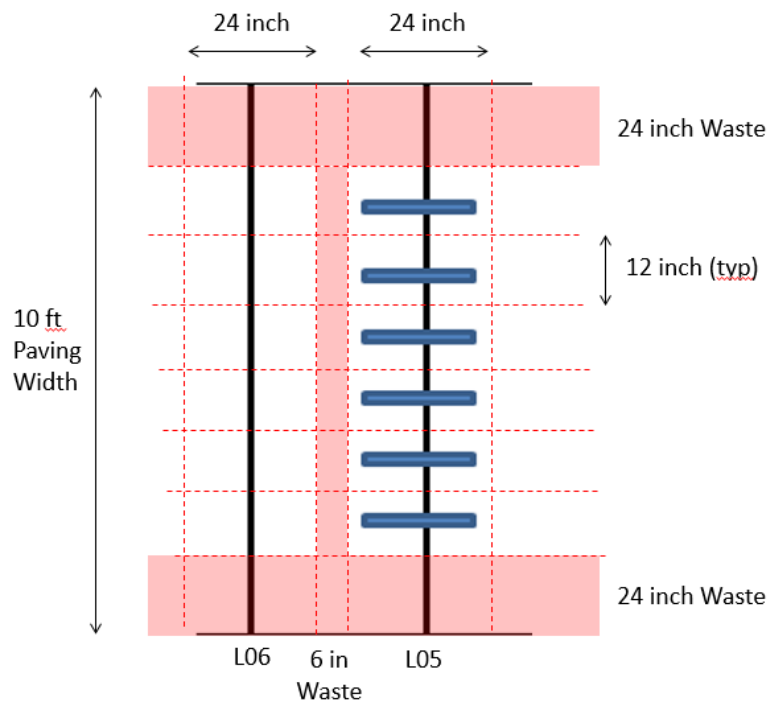
Figure 2.6.1. Typical Full-Depth Sawing Pattern
