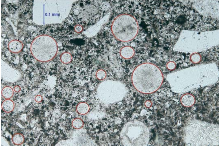
Figure 1.10.1. Secondary Ettringite Deposits in Air Voids (American Engineering Testing, Inc.)
