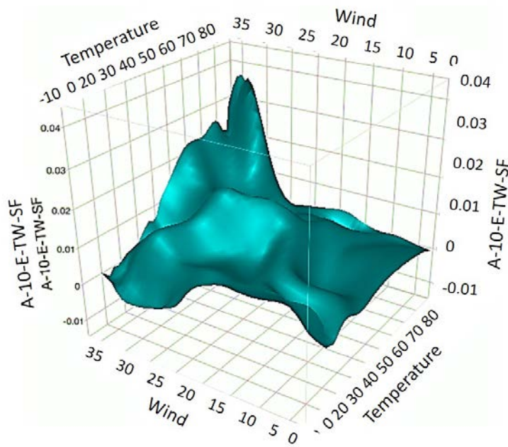
Figure 16. The relationship between the environmental variation to the acceleration response of the studying accelerometers.
