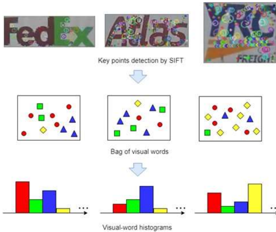
Figure 22: Sample BoW features.
