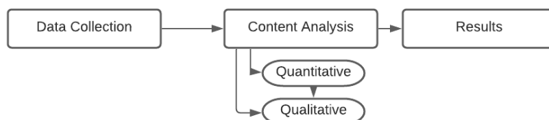
Figure 1. Research Methodology
