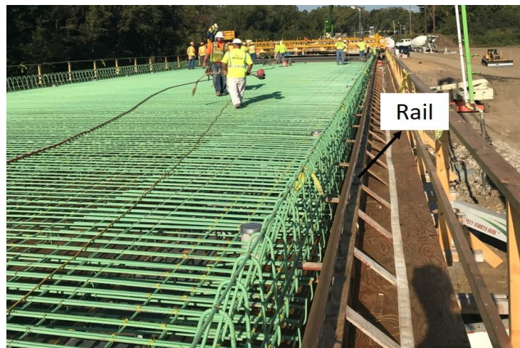
Figure 7. Screed-machine rail located outside the exterior girder on the overhang.
