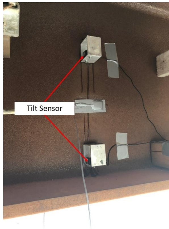
Figure 14. Tilt sensors with open aluminum boxes.
