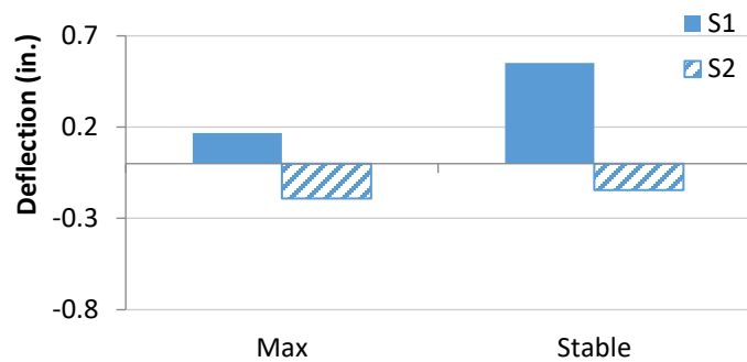
(b) Field measurement of deflection in the exterior girder
