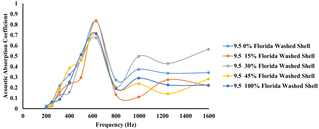
Figure 15. Acoustic absorption results of open-graded asphalt mixtures of 9.5 mm NMAAS
