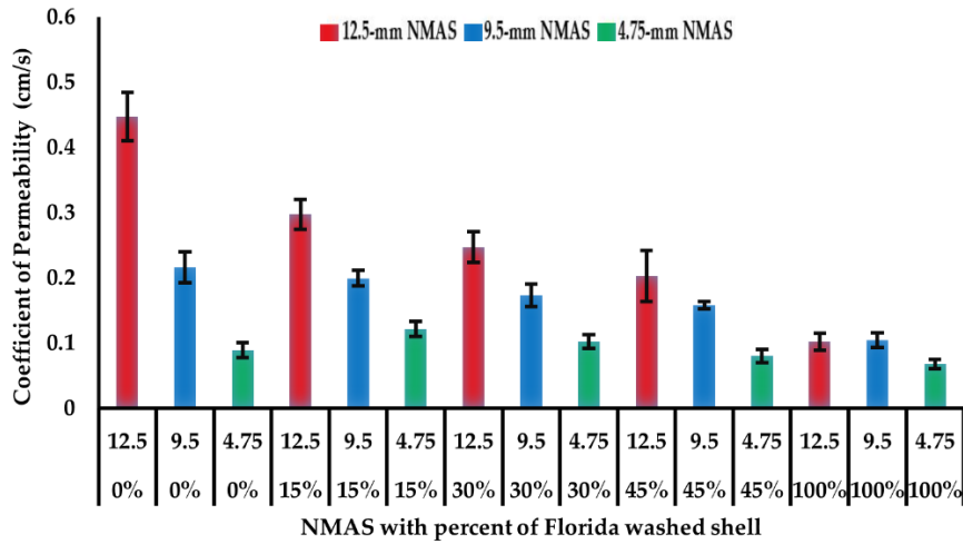
Figure 13. Permeability results of open-graded asphalt mixtures
