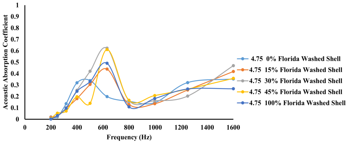
Figure 16. Acoustic absorption results of open-graded asphalt mixtures of 4.75 mm NMAAS
