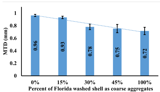
Figure 19. MTD results of open-graded asphalt mixtures of 4.75 mm NMAS
