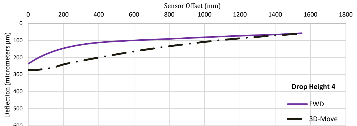
Figure C-25. Simulated Deflection Bowl for the SHRP section B310.
