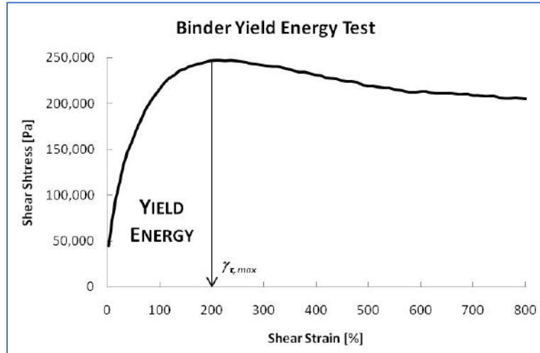
Figure 6. Typical stress-strain curve and parameter calculation for BYET test (4).
