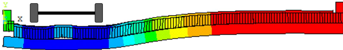
a) Exaggerated deformed shape (LC1)
