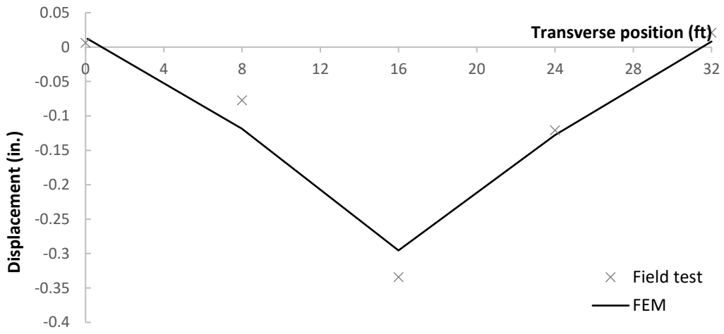
b) Displacement distribution at the middle span
