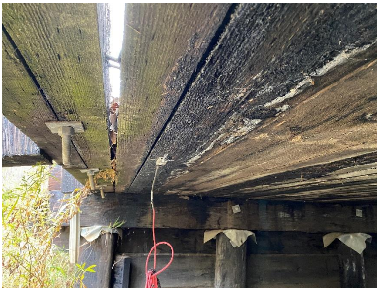
Figure 4-56 Delamination near edge of slab (Monroe Co. P410953)
