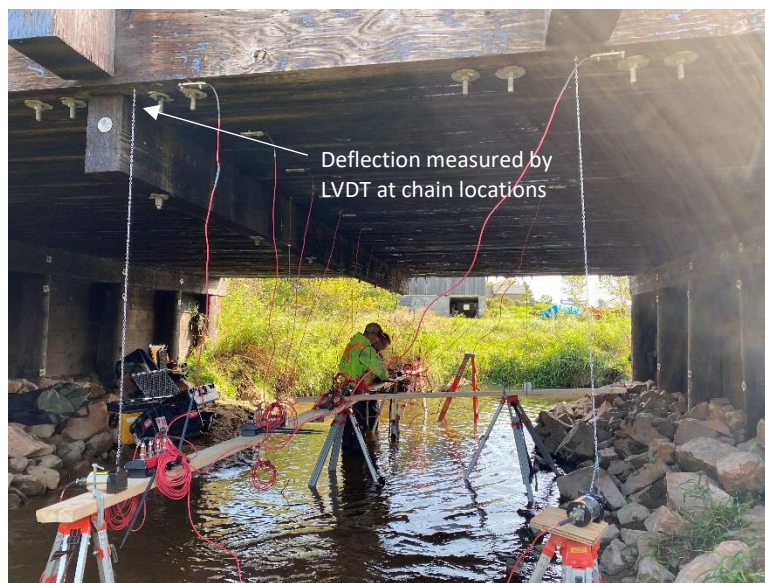
Figure 7-1 Deflection data collected via LVDTs
