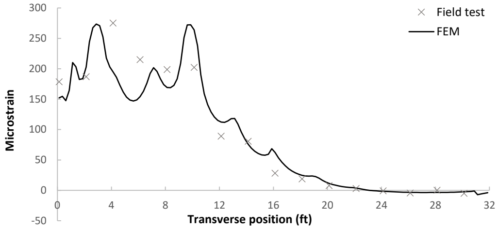
a) Strain distribution at the middle span
