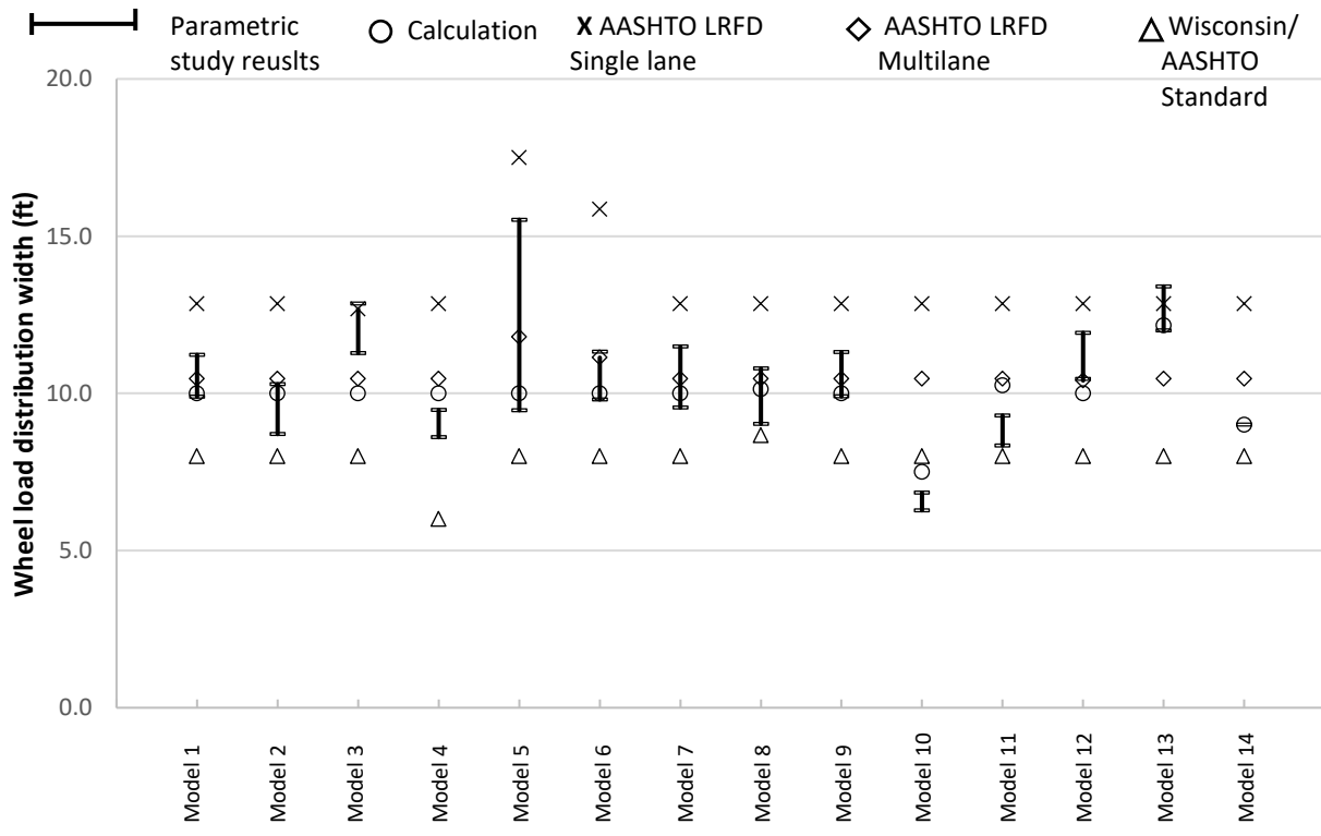
Figure 6-5 Validation of equation by parametric study results
