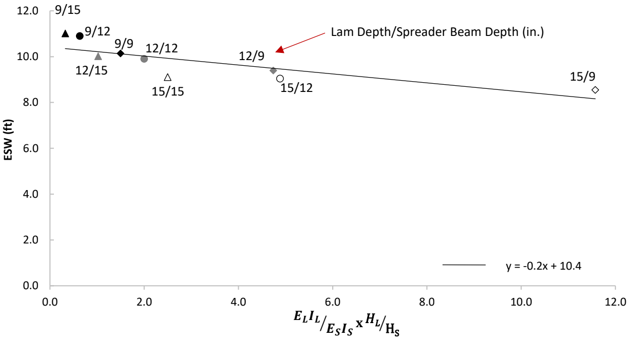
Figure 6-3 ESW with respect to E_L I_L / E_S I_S \times H_L / H_S
