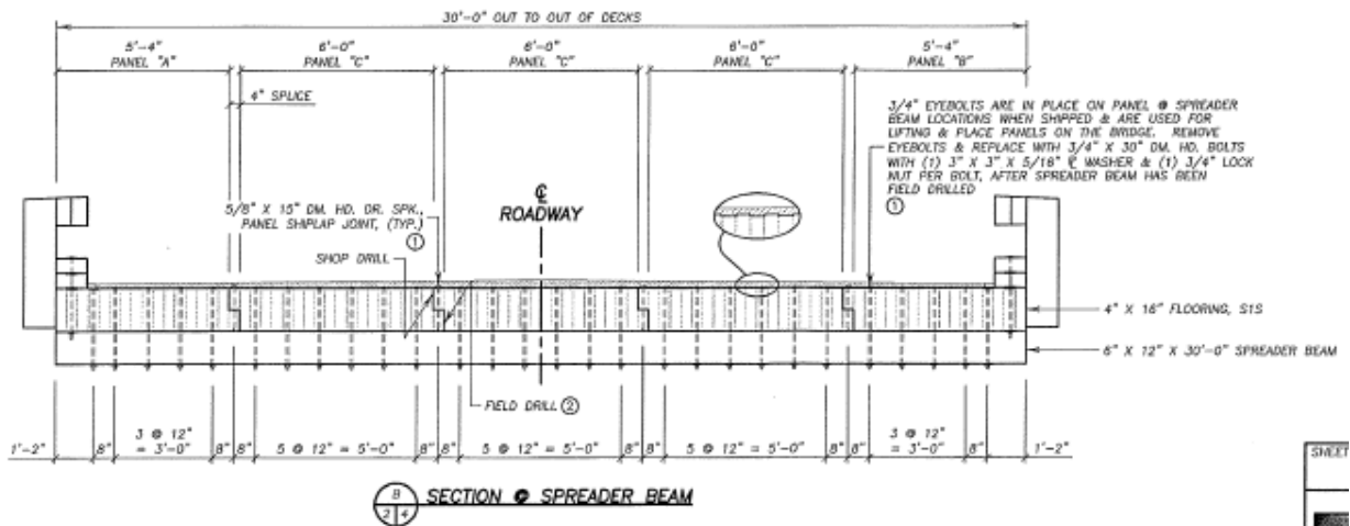
Figure 4-47 Sauk County Bridge B560224 Section View
