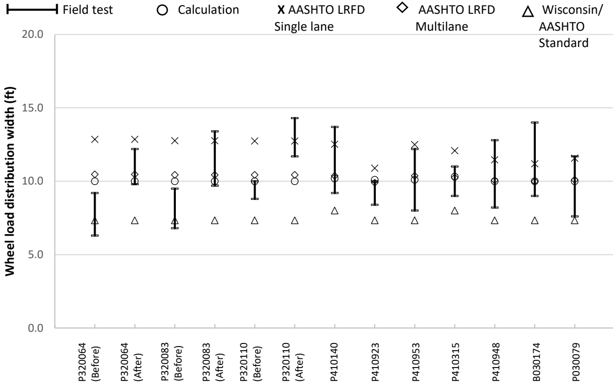
Figure 6-4 Validation of equation by field test data
