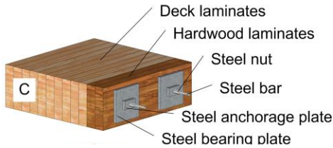
c) Bearing plates used for hardwood decks according to AASHTO;
