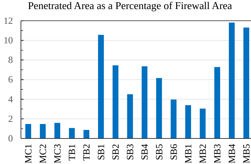
Figure 11. Penetrated area as a percentage of firewall area for the 16 buses surveyed
