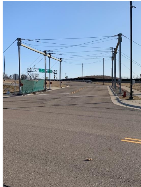
Figure 16: Simulated tree canopy without its suspended camouflage netting installed.
