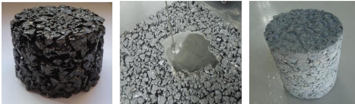
(a) Asphalt pervious concrete (b) Pouring cement mortar (c) CCAM cylinder sample
