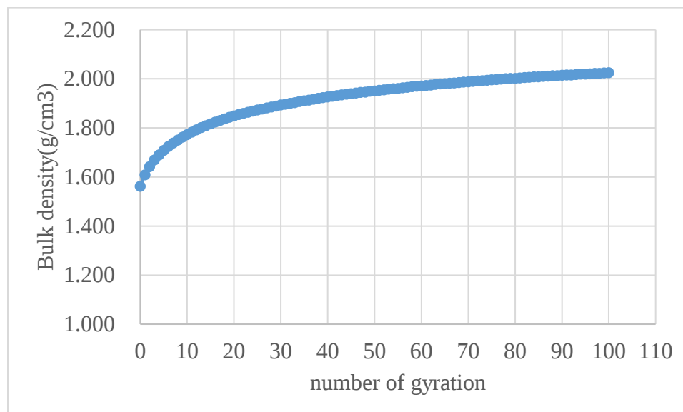
Figure 3.3. Density-gyrations curve
