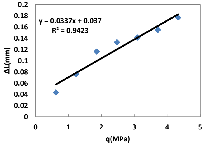
Figure 4.8. Regression of resilient deformation
