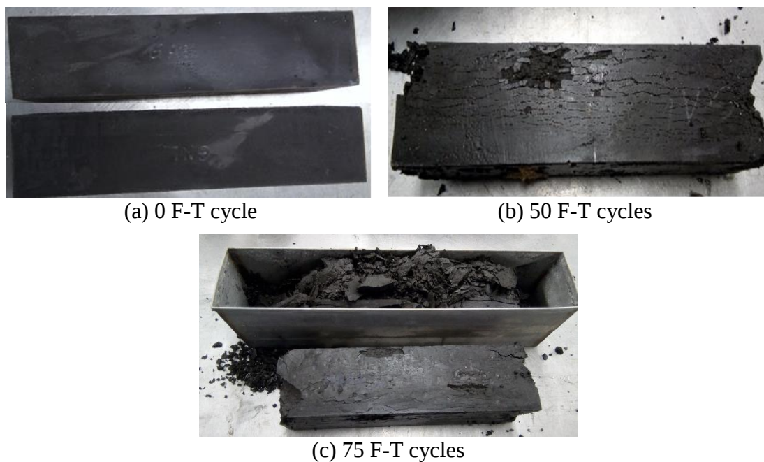
Figure 4.20. ESG after different F-T cycles
