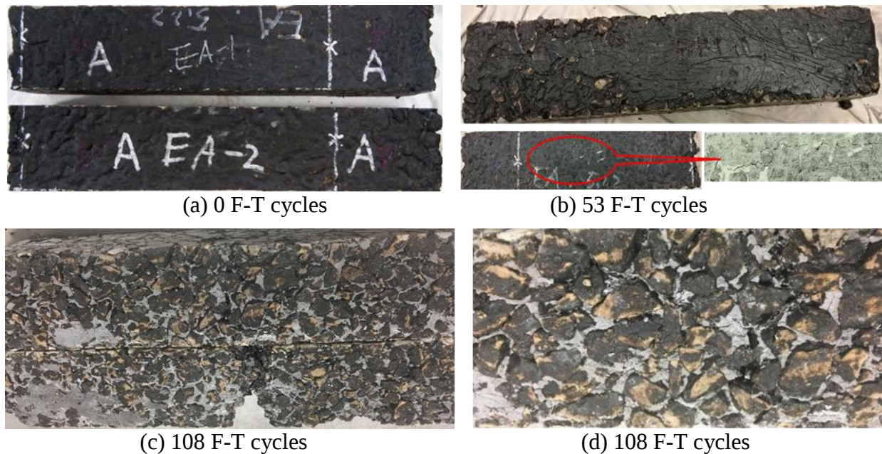
Figure 4.23. The CCAM-ESG after different F-T cycles
