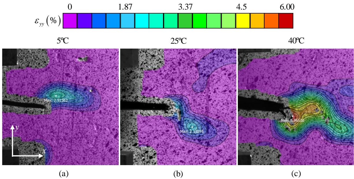
Figure 4.8 – Contours of longitudinal percent strain, \varepsilon_{yy} (%) at the maximum load during fracture tests
