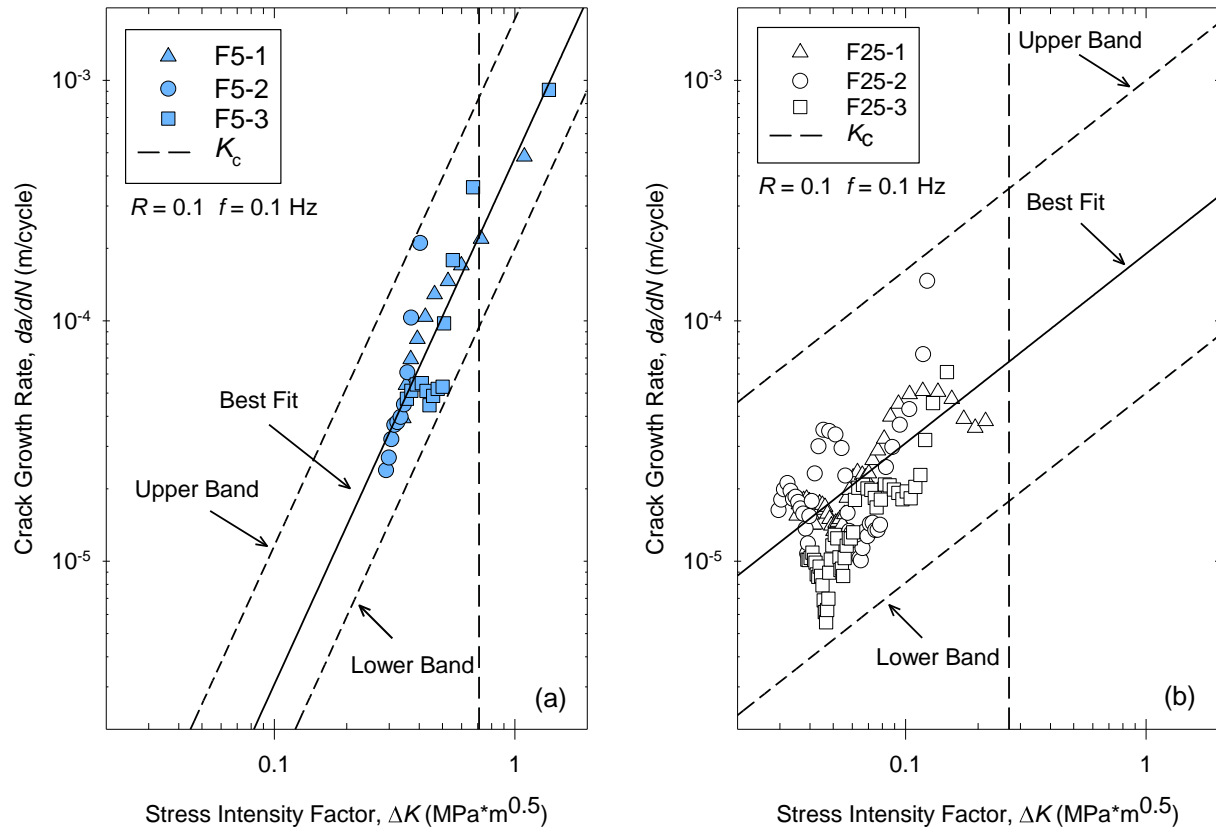
Figure 4.13 – Summary of fatigue crack growth data (a) 5°C and (b) 25°C
