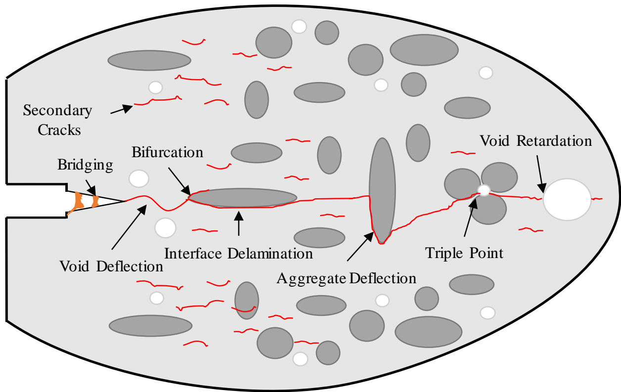
Figure 4.15 – Cracking mechanisms in HMAs
