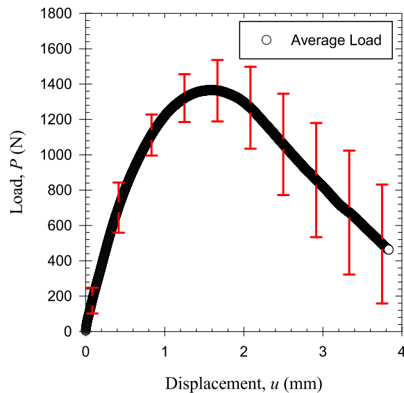
Figure 2.6. Average load-displacement curve for 24\pm 1.5\text{mm} SCB specimens according to AASHTO TP105
