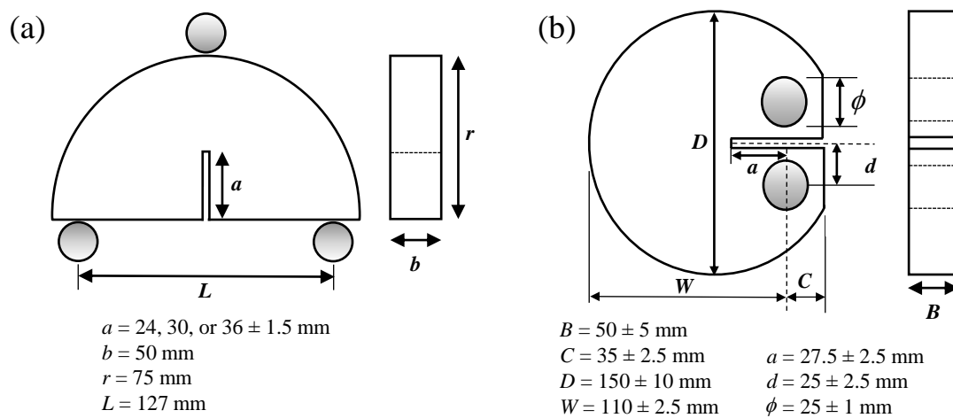
Figure 2.4. Schematic and dimensions of (a) SCB and (b) DCT specimen
