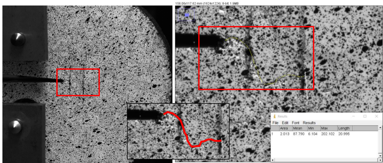
Figure 4.5 – Crack length measurement
