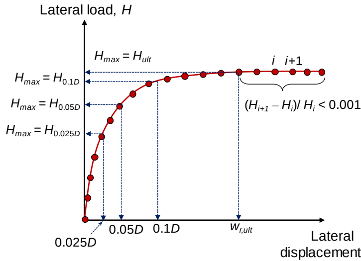
Figure 2.2 Graphical illustrations of ultimate lateral capacity criteria used in this study
