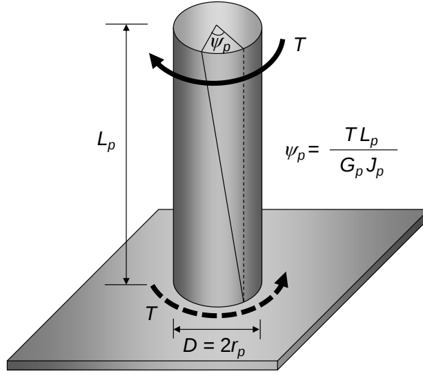
Figure 2.3 Angle of twist of a cylinder subjected to a torque
