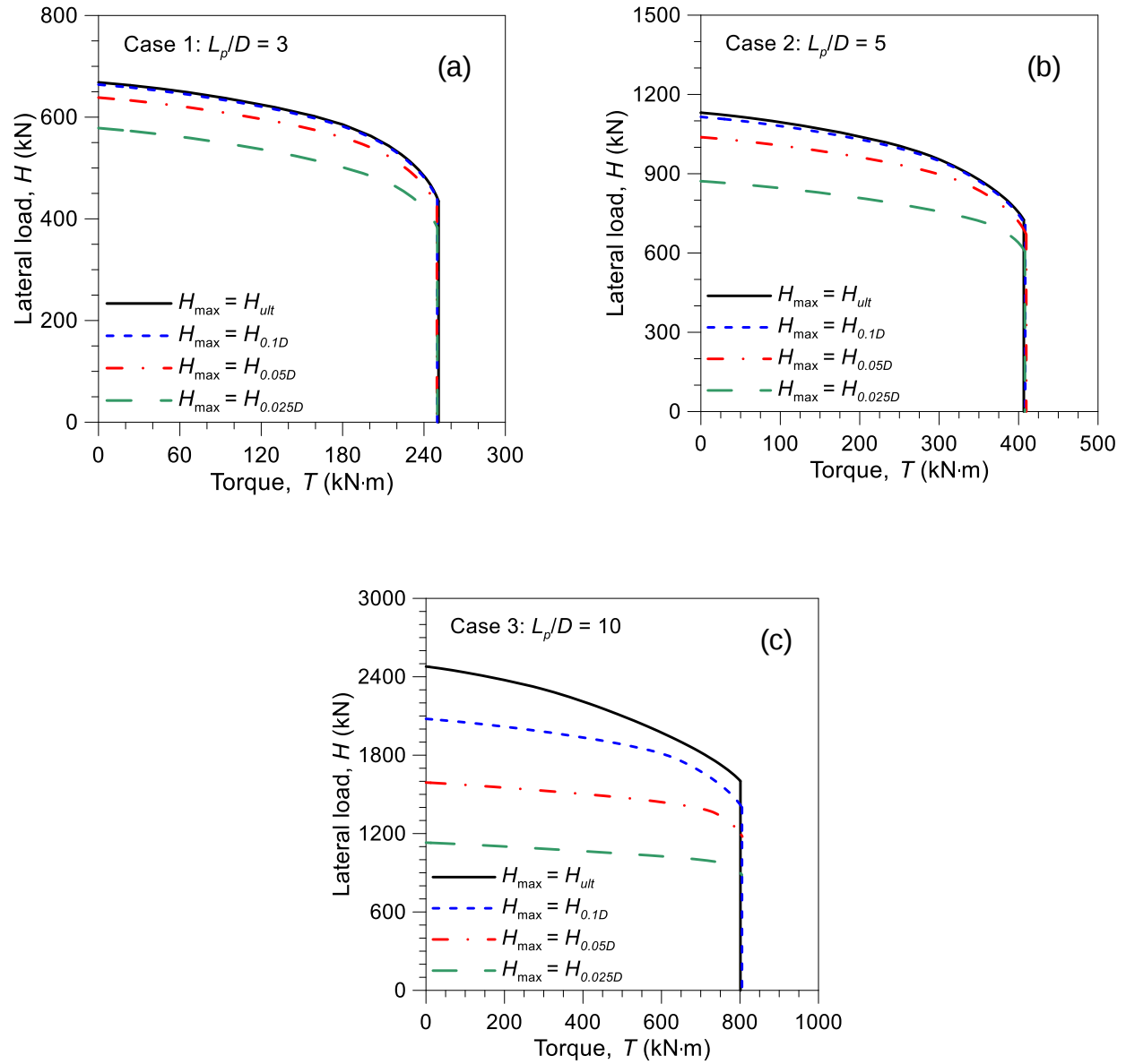
Figure 2.7. Note that four different definitions of H_{\max} (i.e., H_{\max} = H_{ult} , H_{0.1D} , H_{0.05D} , and H_{0.025D} ), as presented in Figure 2.2 and Table 2.1, were used to plot the failure envelopes. Accordingly, a lateral displacement was gradually increased until reaching w_{r,ult} for each definition of H_{\max} , and then an angle of twist \psi_p of the drilled shaft was increased while keeping the lateral displacement constant at w_{r,ult} .
