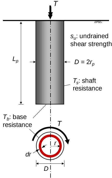
Figure 2.4 Torsional resistances of the foundation in soil
