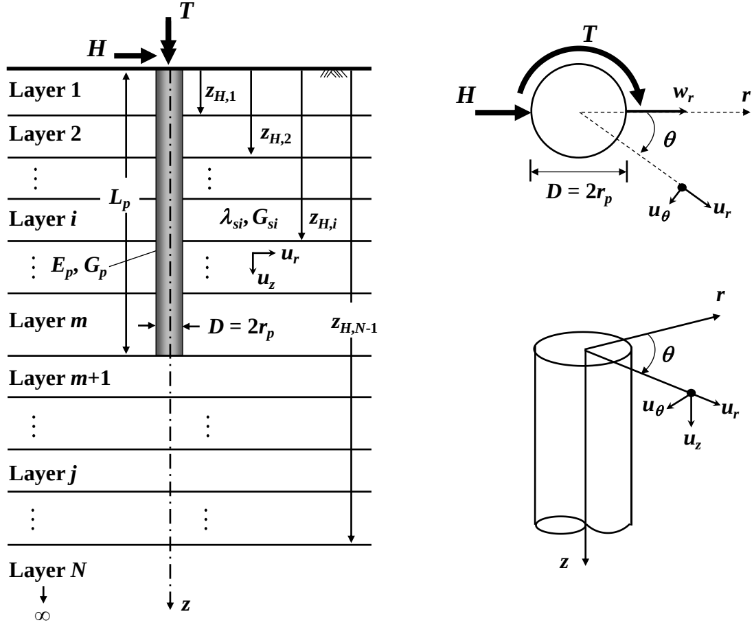
Figure 3.1 Geometry of the foundation-soil system
