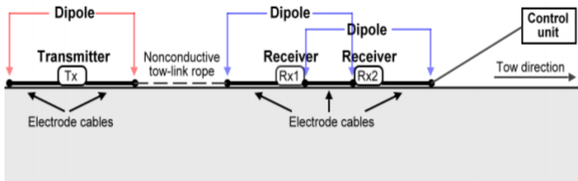
Figure 2-2. A schematic of the OhmMapper capacitively coupled AC resistivity system with one transmitter dipole and two receiver dipoles arranged in dipole-dipole configuration (Lucius et al. 2008) (5)
