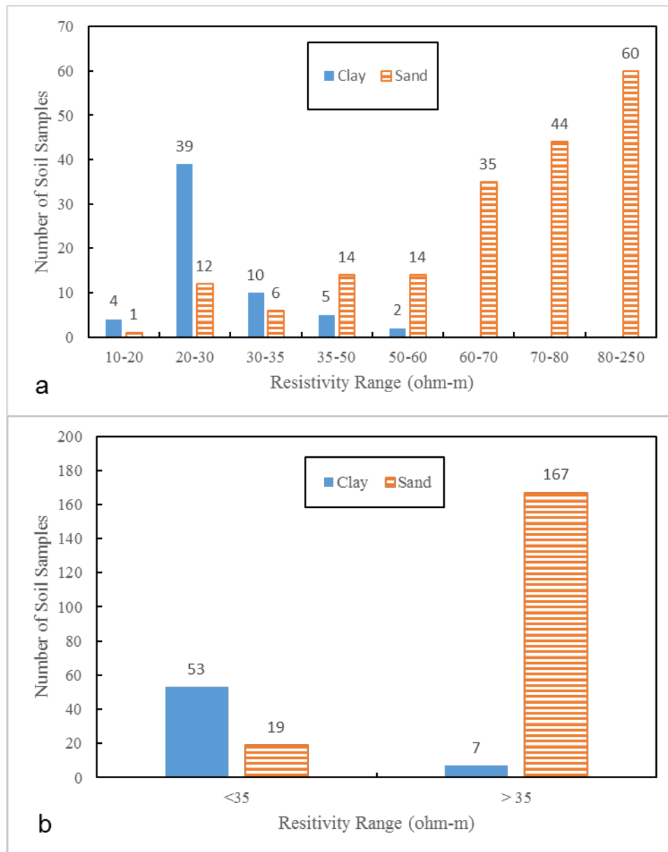
Figure 4-8. a) Distribution of soil samples b) Distribution of soil samples either side of hypothetical resistivity separator between clay and sand samples based on their resistivity at landside of Mel Price site
