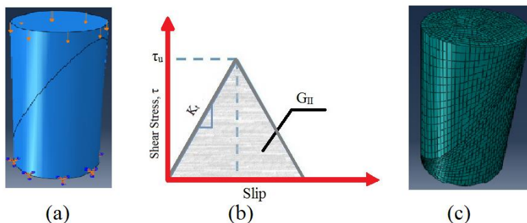
Figure 38: FE model using ABAQUS simulation environment: (a) Boundary conditions (b) Bilinear shear stress-slip relation where \kappa_c is shear contact stiffness, G_{II} is mode II fracture energy and \tau_u is maximum shear stress (c) Meshed model using 74,524 elements.
