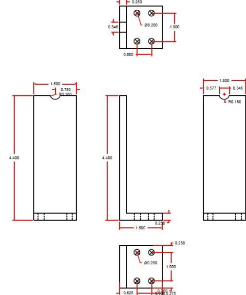
(f) Loading frame: Right support
