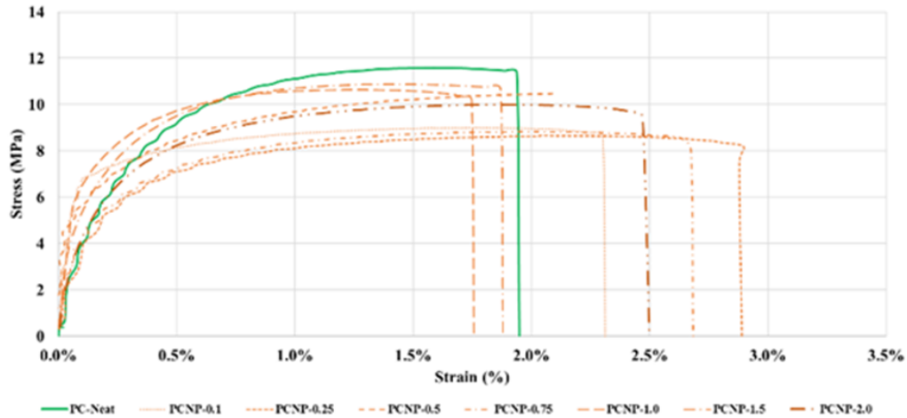
(b) NCP mixtures incorporating P-MWCNTs stress-strain curves for tensile test
