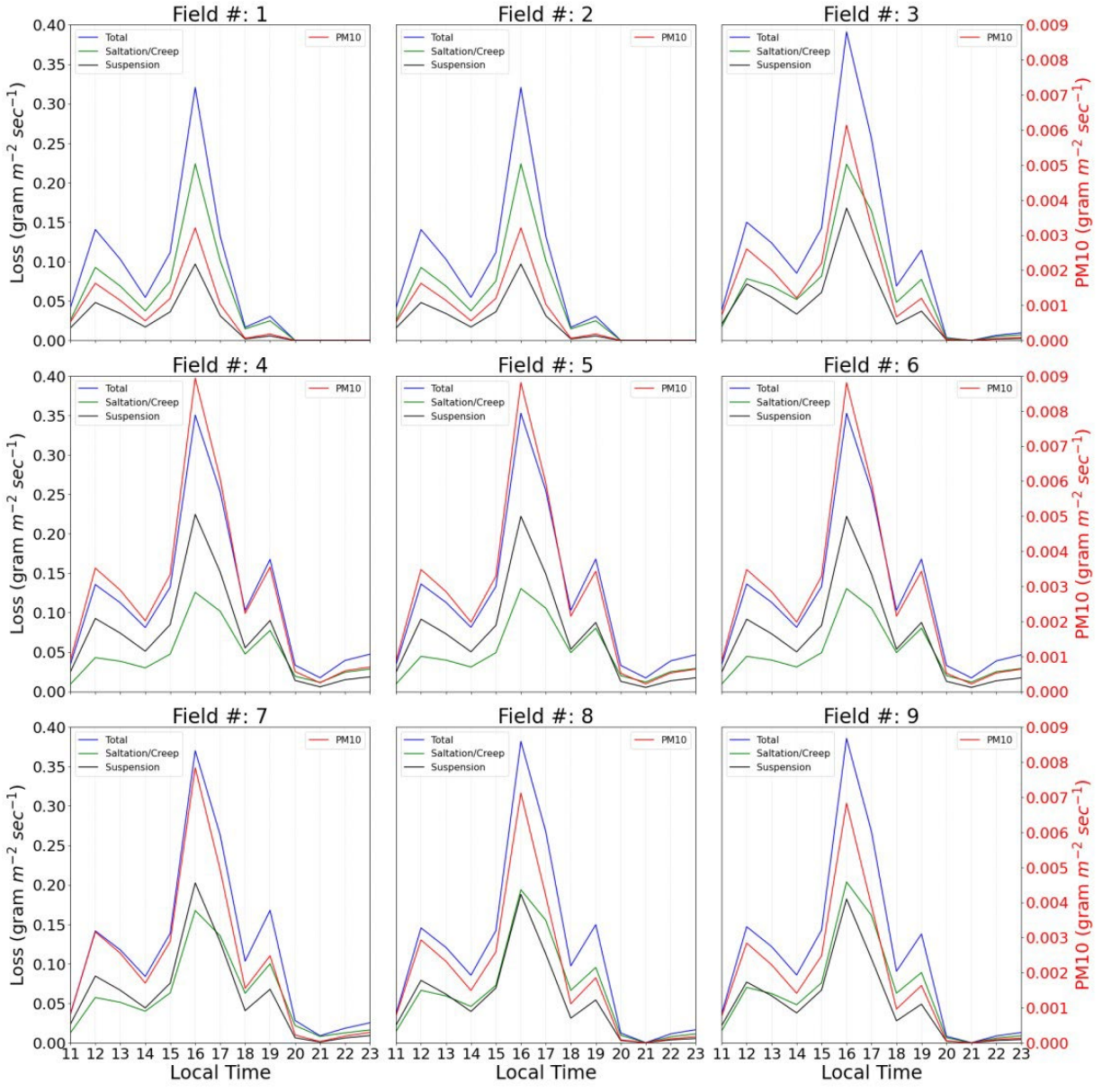
Figure 25. SWEEP simulated soil loss in terms of total, saltation/creep, suspension, and PM 10 from the Road Forks field during the dust event of February 3, 2020.
