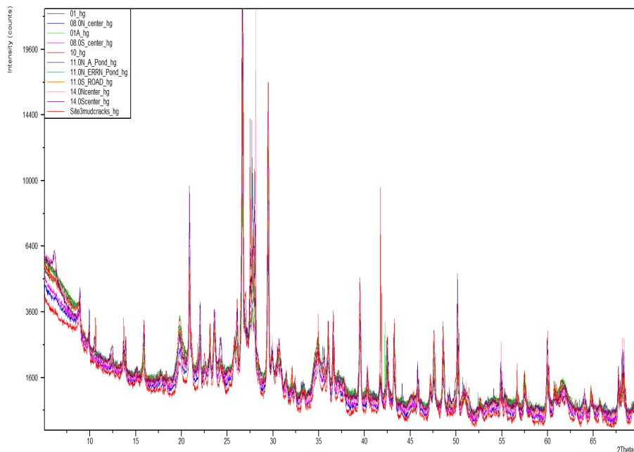
Figure 16. X-ray diffraction outputs of selected Lordsburg Playa sediments, showing similarity of composition.
