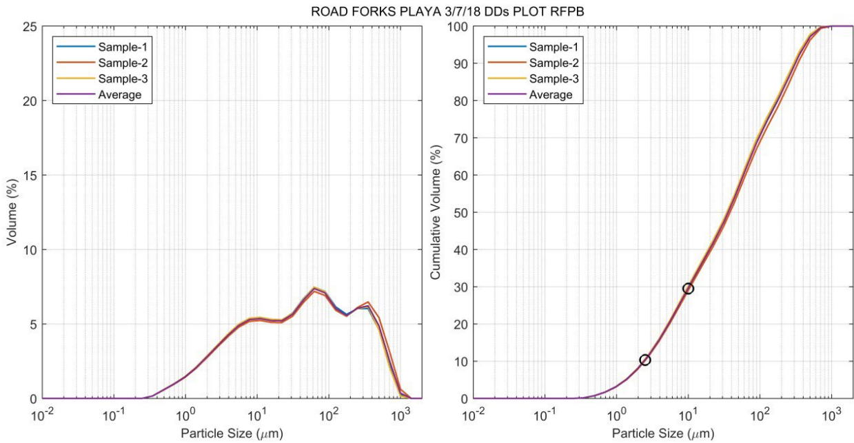
Figure 13. Grain size distribution of the soil at the Road Forks field.
