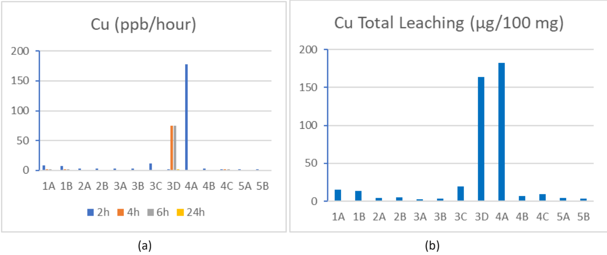
Figure 17. Comparison of (a) Cu leaching rate of Lordsburg Playa sediment samples in ppb/hour and (b) total Cu leaching for each sample.
