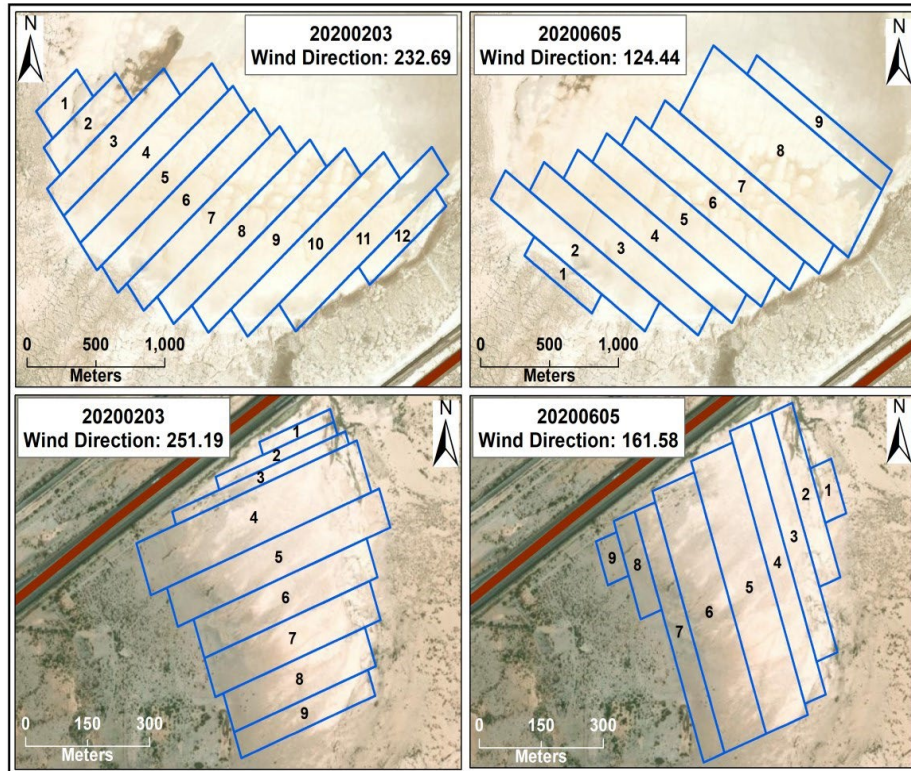
Figure 10. Geometry of field locations at North Playa (top) and Road Forks (bottom).
