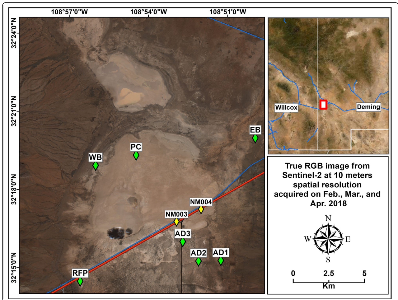
Figure 2. Location of Lordsburg Playa in southwestern North America.
