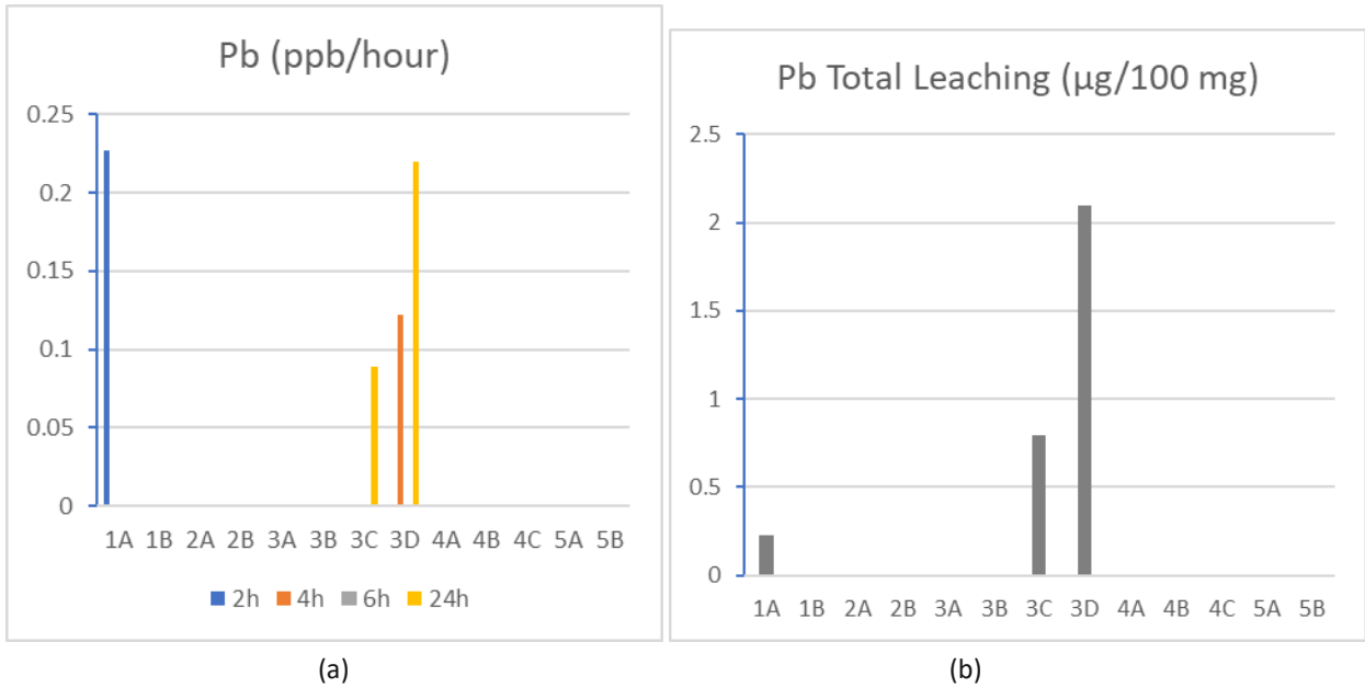
Figure 18. Comparison of (a) Pb leaching rate of Lordsburg Playa sediment samples in ppb/hour and (b) total Pb leaching for each sample.
