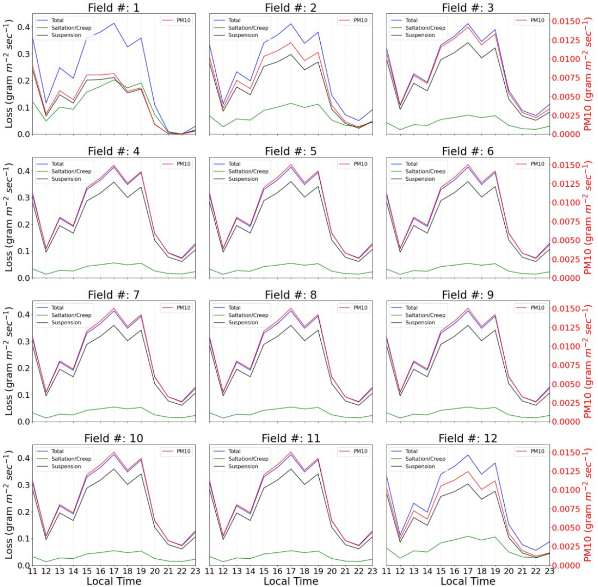
Figure 23. SWEEP simulated soil loss in terms of total, saltation/creep, suspension, and PM 10 from the North Playa field during the dust event of February 3, 2020.
