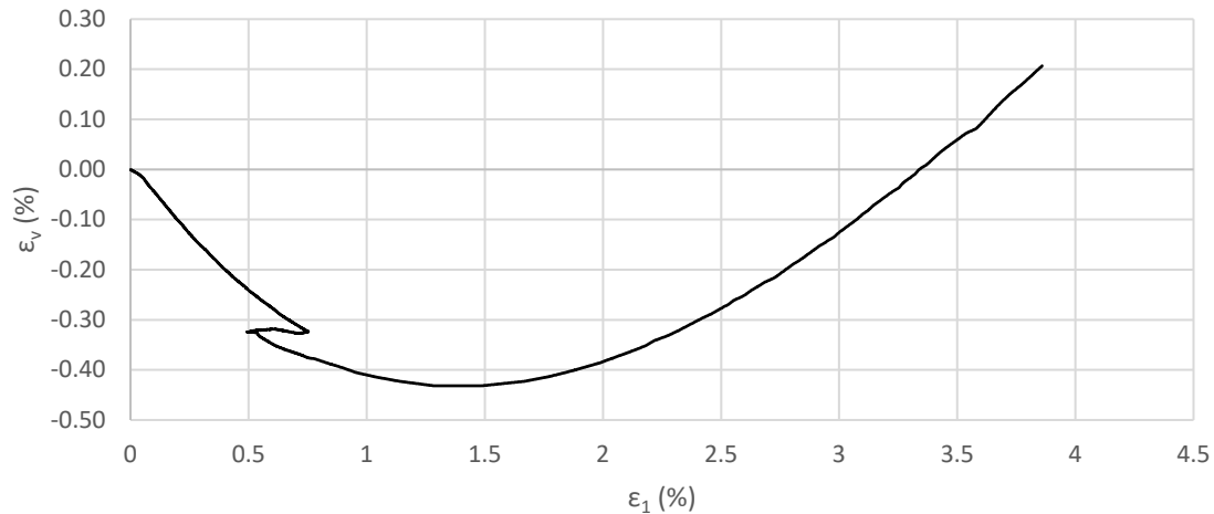
Figure 16. Volume change measurement
