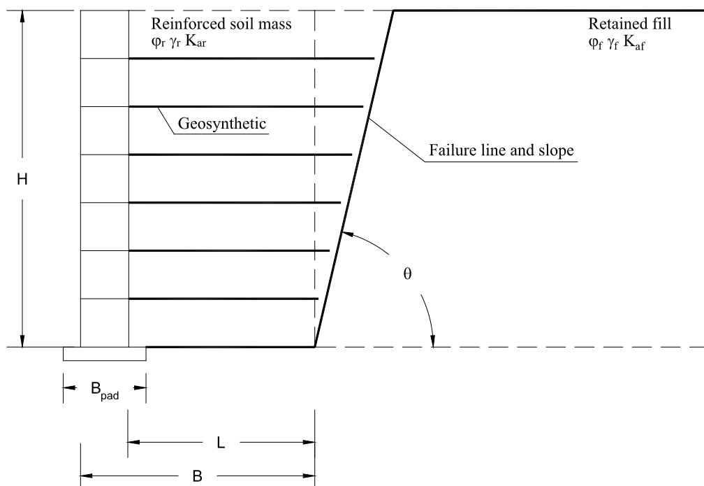
c) Truncated base wall Figure 64. Failure assumptions
