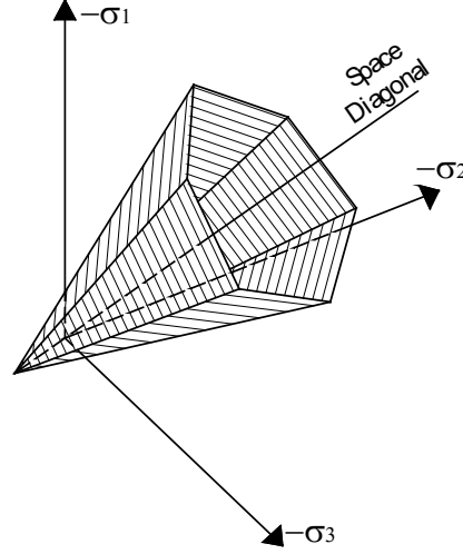
Figure 49. Mohr-Coulomb failure criteria in principal stress space
