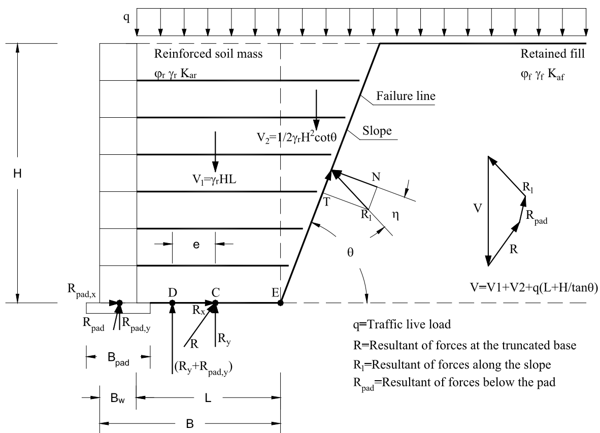
c) Truncated base wall Figure 64. Failure assumptions
