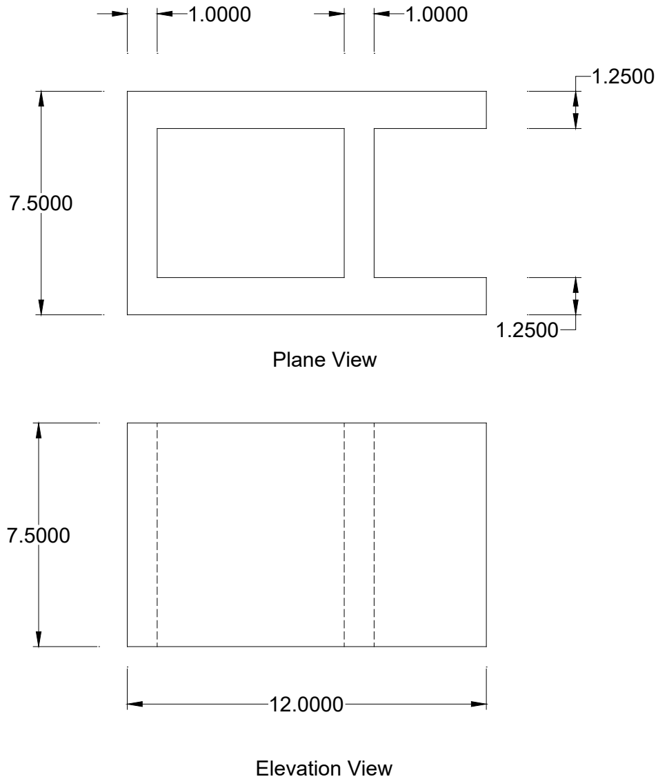
Figure A7. Block facing for the interface test
