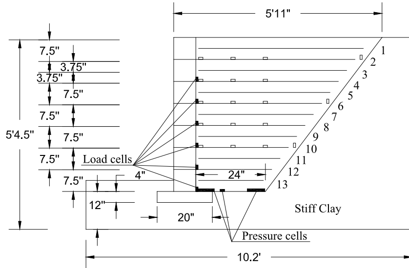
Figure 33. No. 3 GRS Wall (53°)
