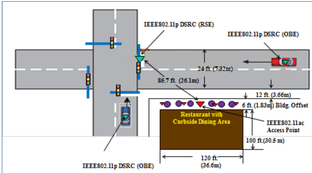
Figure 6-1. Test Geometry for Outdoor Restaurant with an IEEE 802.11ac Access Point at an Intersection with an Installed RSE
