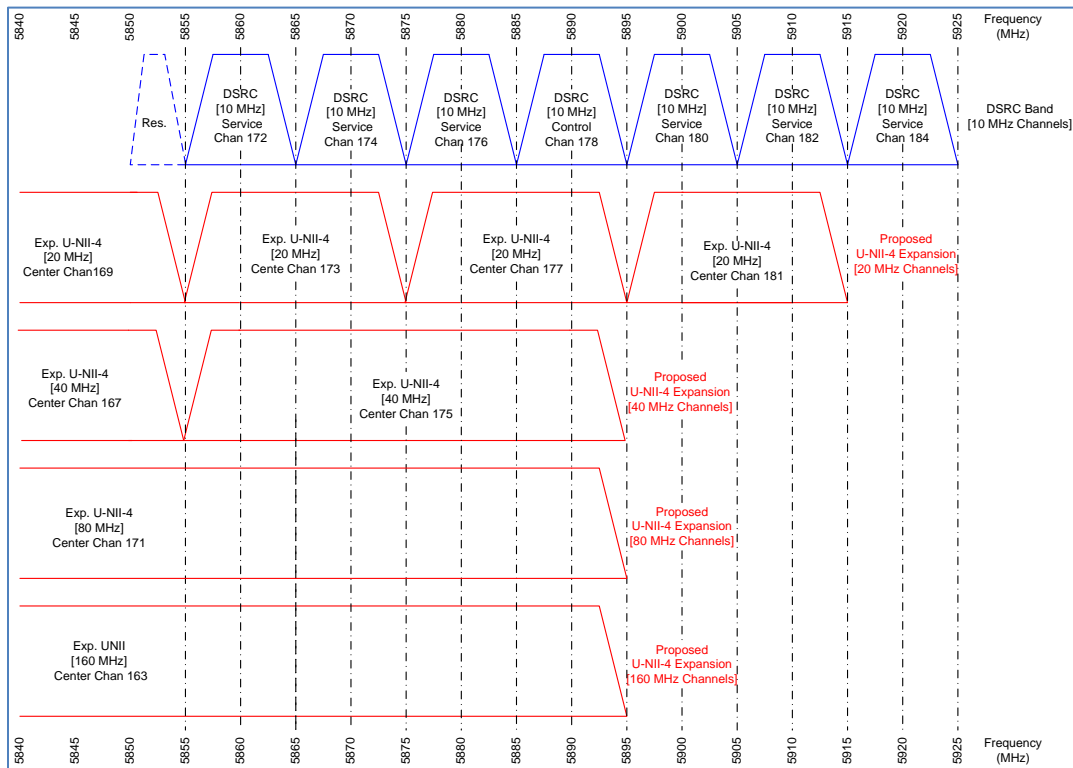
Figure 1-3 U-NII-4 overlap with the DSRC band 10
