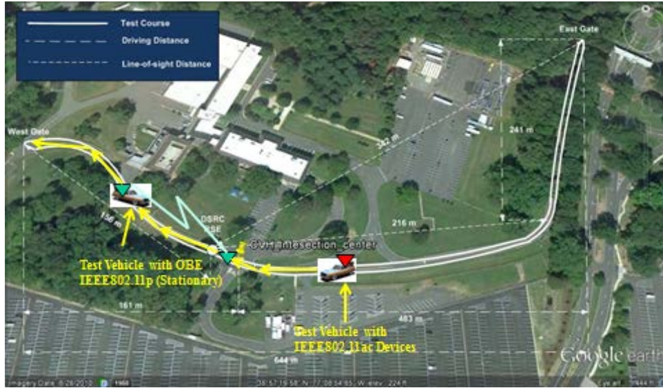
Figure 6-5. Location of Test Vehicles Associated with In-Vehicle IEEE 802.11ac Compatibility Testing with OBEs in Other Vehicles and RSE
