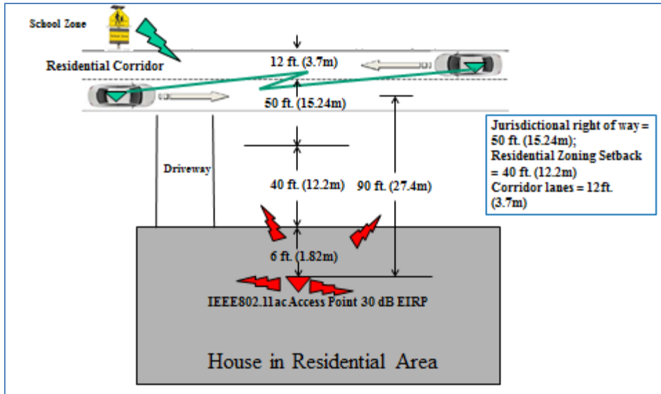
Figure 6-2. Residential Street with Homes Having IEEE 802.11ac Access Points with Passing Vehicles Having DSRC Devices and Possibly a School Zone Warning RSE
