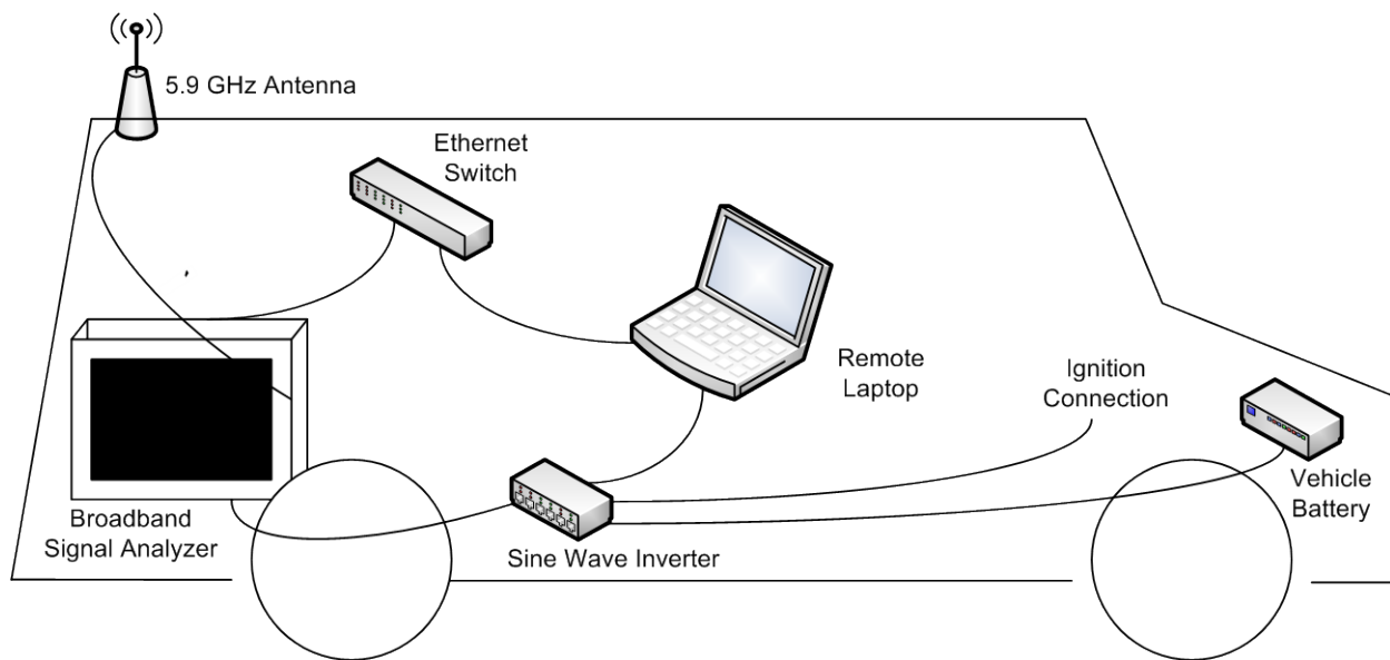
Figure 4-5 RF Signal Measurement Mobile Configuration
