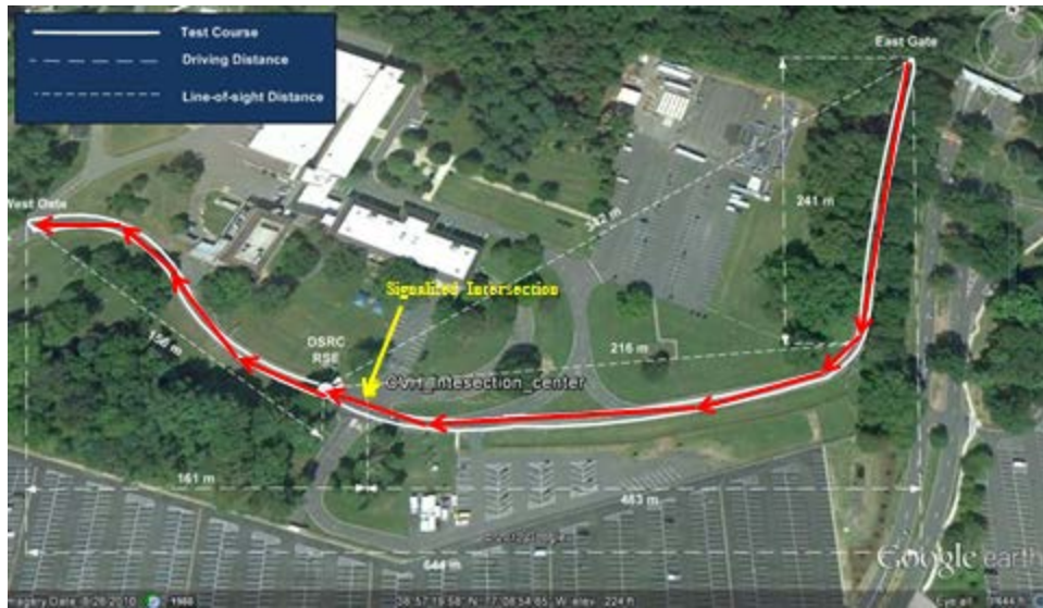
Figure 5-1. Baseline Test of IEEE 802.11p and IEEE 802.11ac Radios
