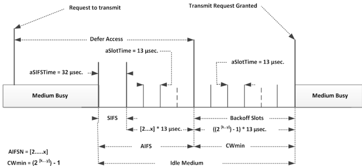
B-1 Figure 1. Breakdown of interframe spacing
