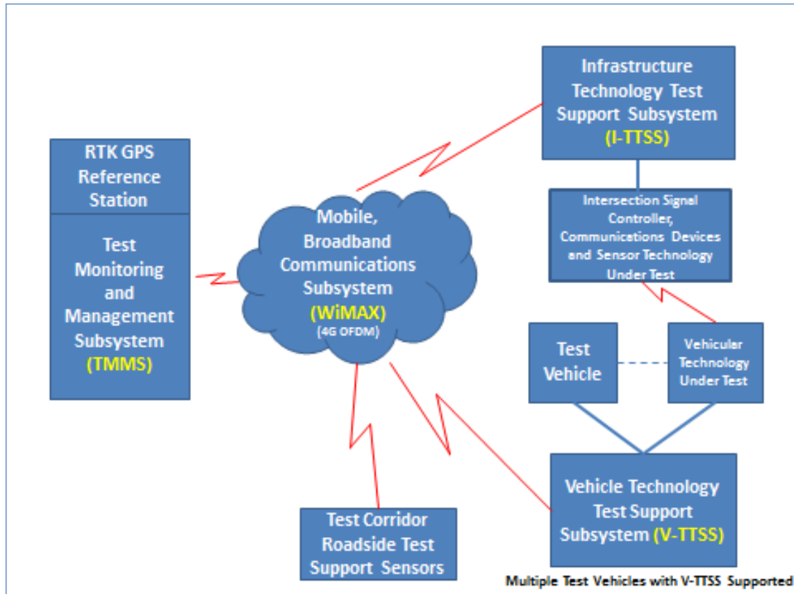
Figure 4-3 Simplified Overview of CVHT System
