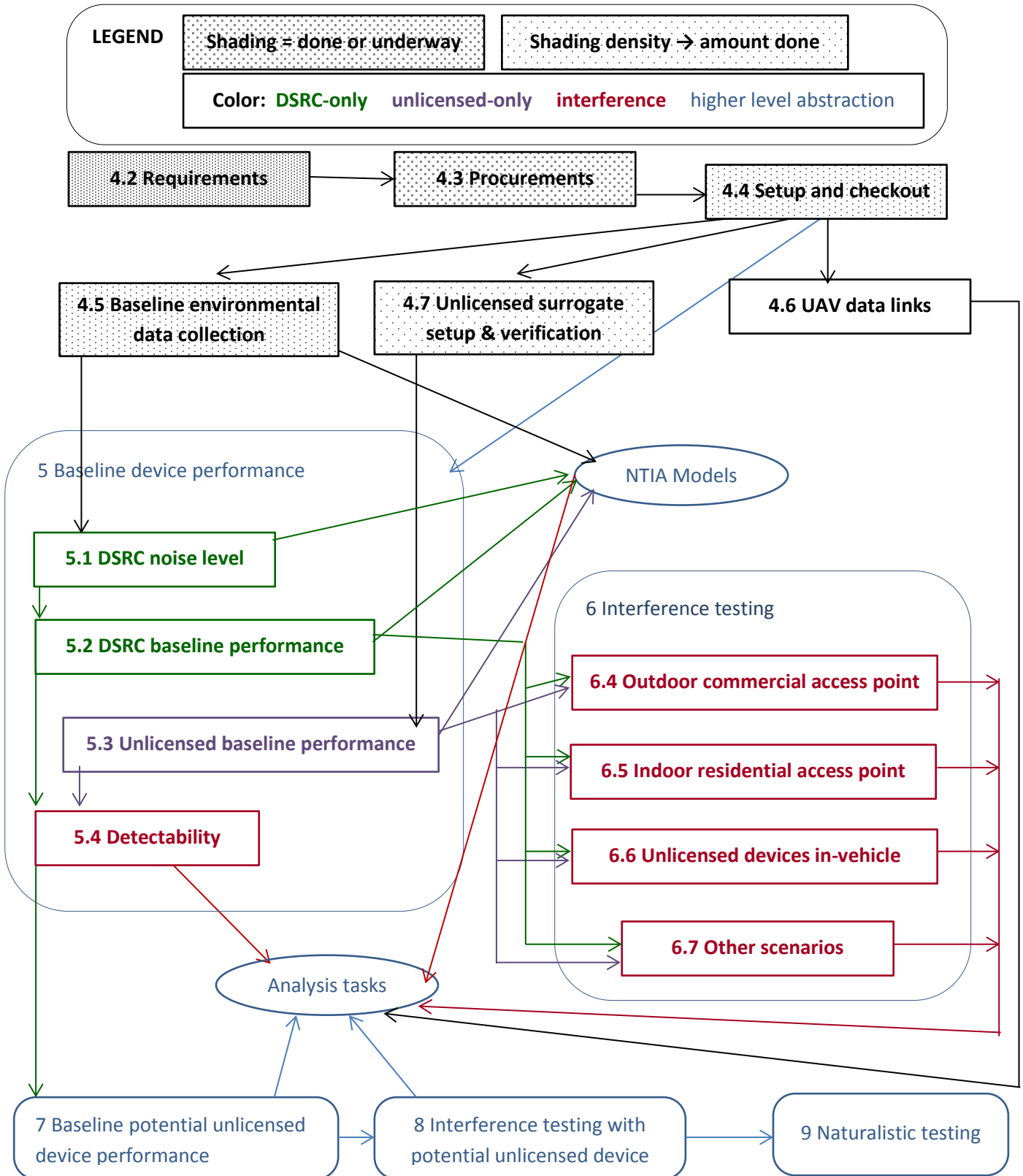
Figure 3-1 Test activity dependencies
