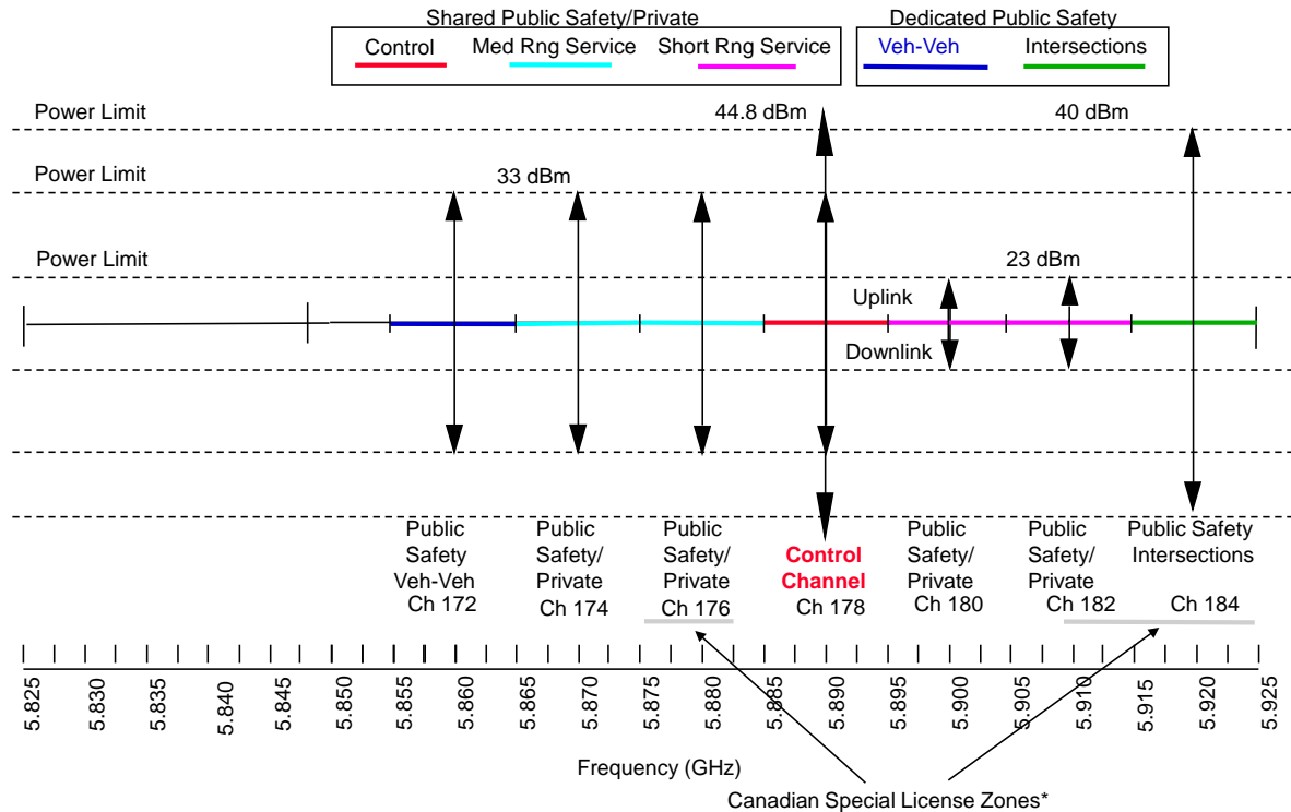
Figure 1-1 DSRC Channel Plan in the ITS Band 6 7
