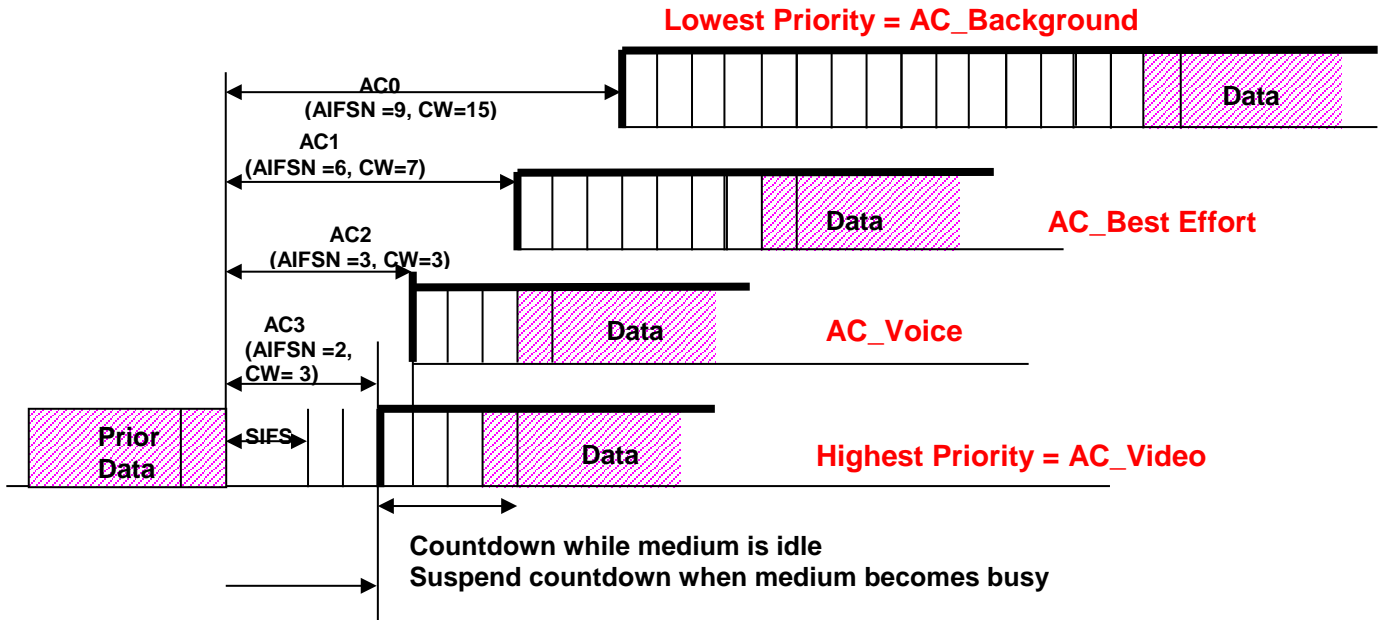
B-2 Figure 2. Depiction of 802.11 default EDCA parameters (Source: John Kenny, Toyota)
