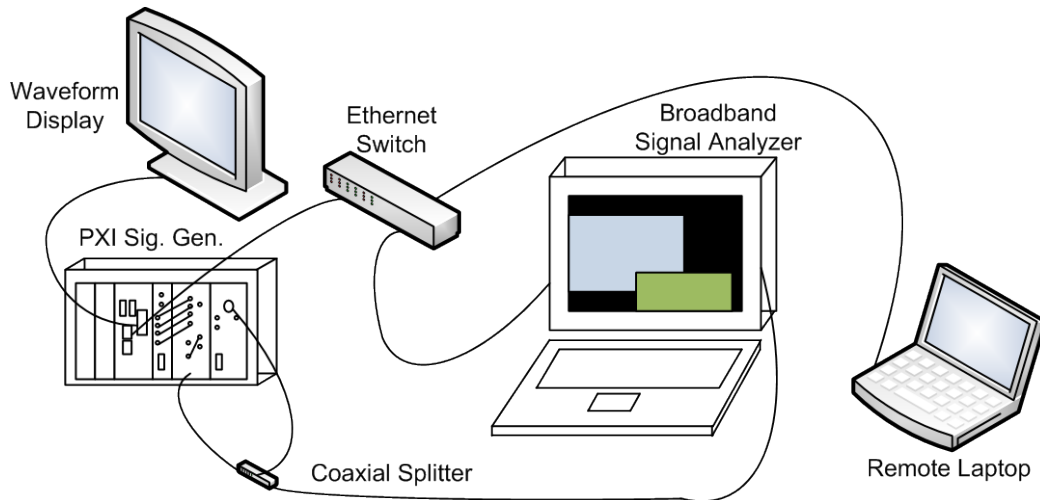
Figure 4-1 RF Signal Measurement Lab Configuration
