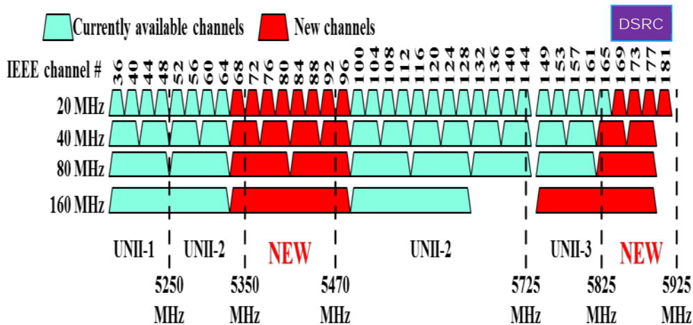
Figure 1-2 Proposed new U-NII-4 band
