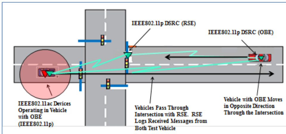
Figure 6-4. Test with IEEE 802.11ac Devices Transmitting in a Vehicle
