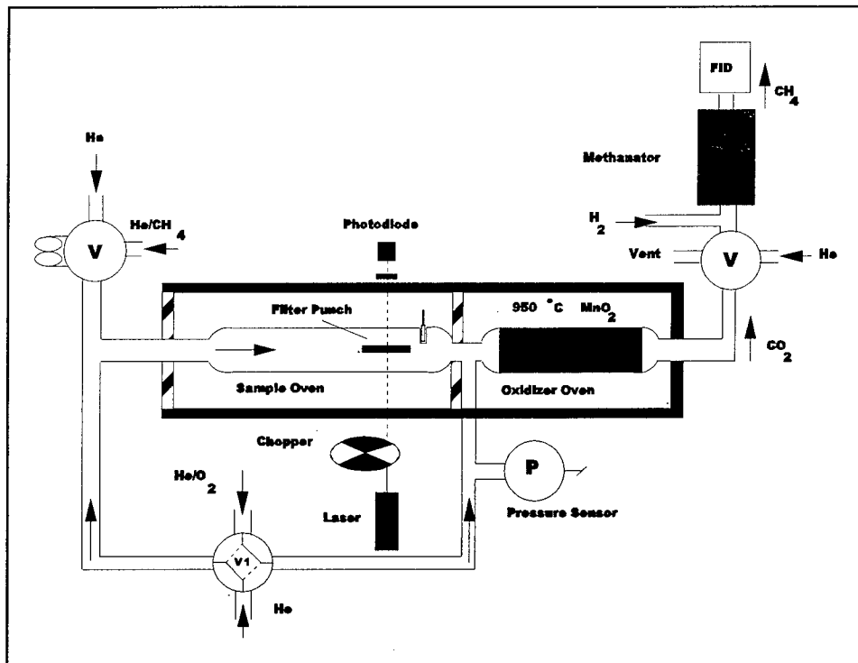
Figure 1. Schematic of Thermal-Optical Analyzer.
