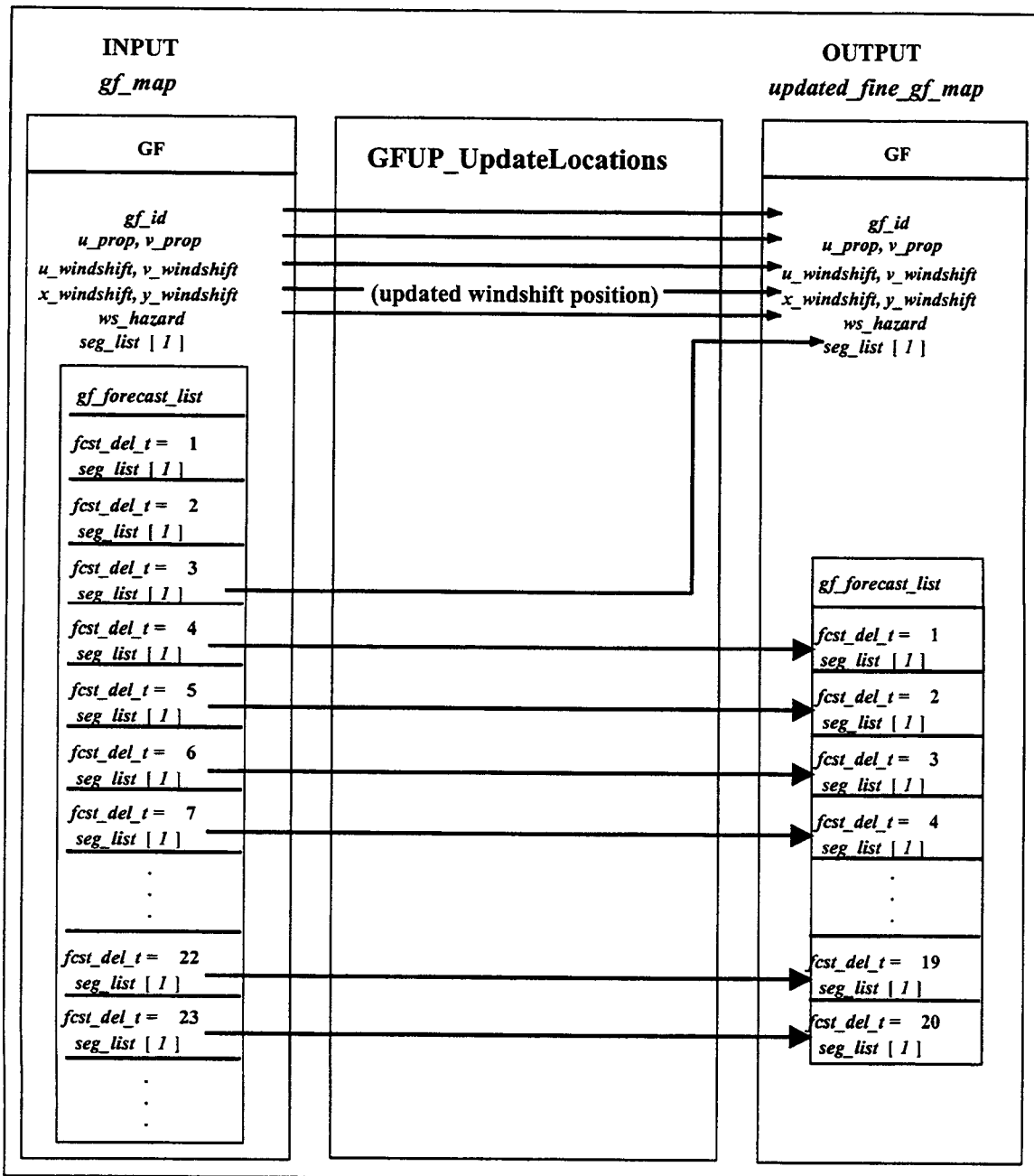
Figure 3. Data flow diagram for the GFUP_UpdateLocations function showing mapping of the data from a single GF in an input GF_MAP ( gf_map ) into a corresponding GF in the output GF_MAP ( updated_fine_gf_map ). For this illustration, a total delay ( migfa processing delay + G_update_timer_val ) of 3 minutes is assumed. (Not all fields of the GF data structure are shown.)
