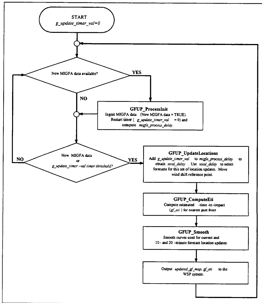
Figure 2. GFUP algorithm functional flow diagram.
