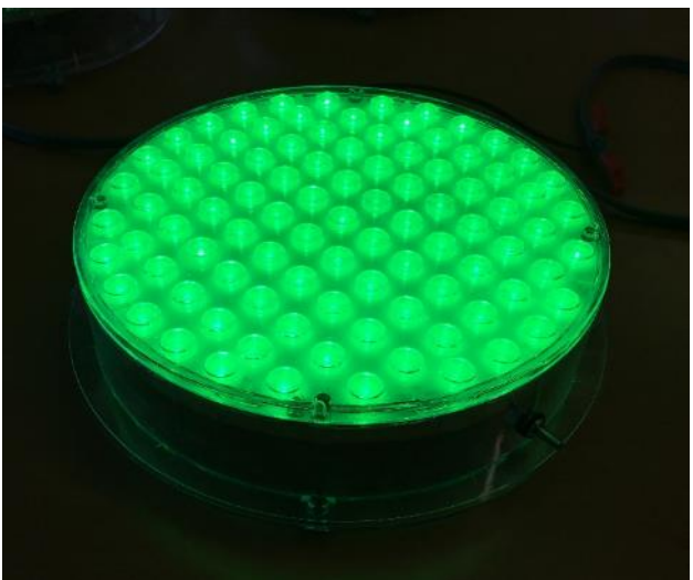
Figure 1: Prototypes of the new type of self-de-icing LED signals (Red, Yellow, Green) for highway signalized intersections
