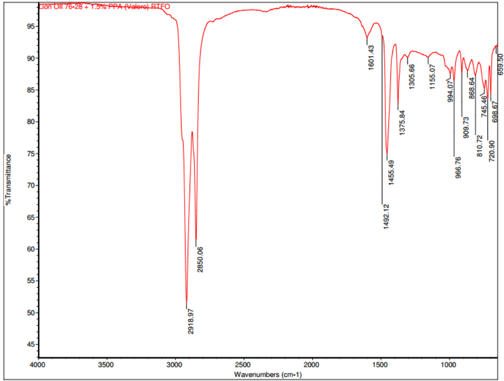
Figure D13 FTIR result for S3 PG 76-28 + 1.5% P1
