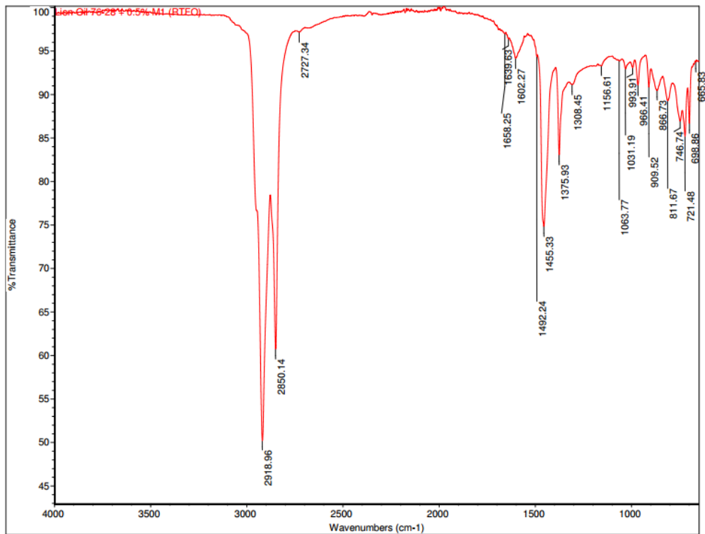
Figure D10 FTIR result for S3 PG 76-28 + 0.5% W1
