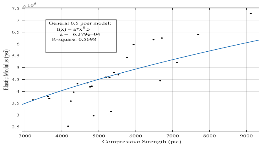
Figure 4.7. 0.5 Power Model for Elastic Modulus
