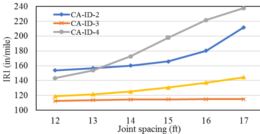
Figure 7.8. Impact of Joint Spacing on Pavement Roughness
