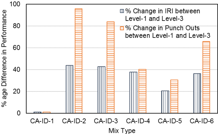
Figure 7.31. Percent Change in CRCP Performance Between Level1 and Level-3 Inputs
