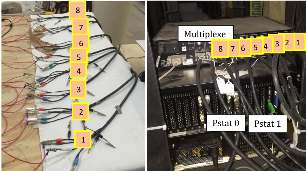
Figure 16. Polarization Resistance Electrodes
