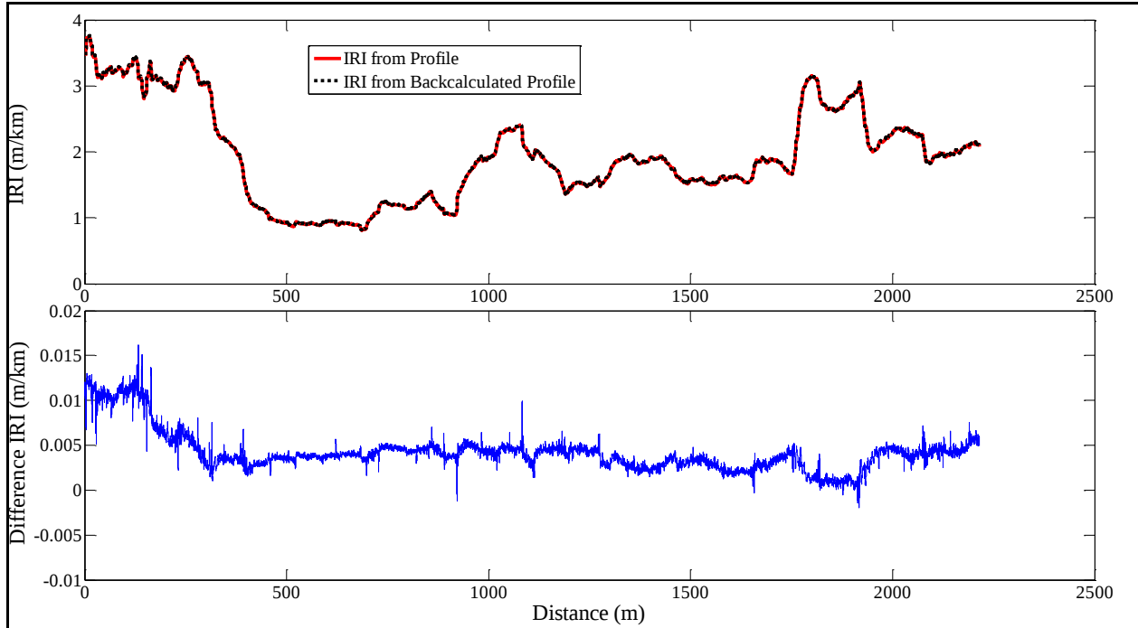
Figure 3. Accuracy of IRI calculation; calculated IRI (top) and difference between calculated IRI (bottom).
