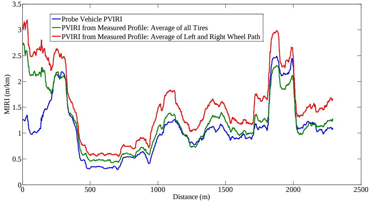
Figure 5. Effect of approximating full car model with average quarter car models.
