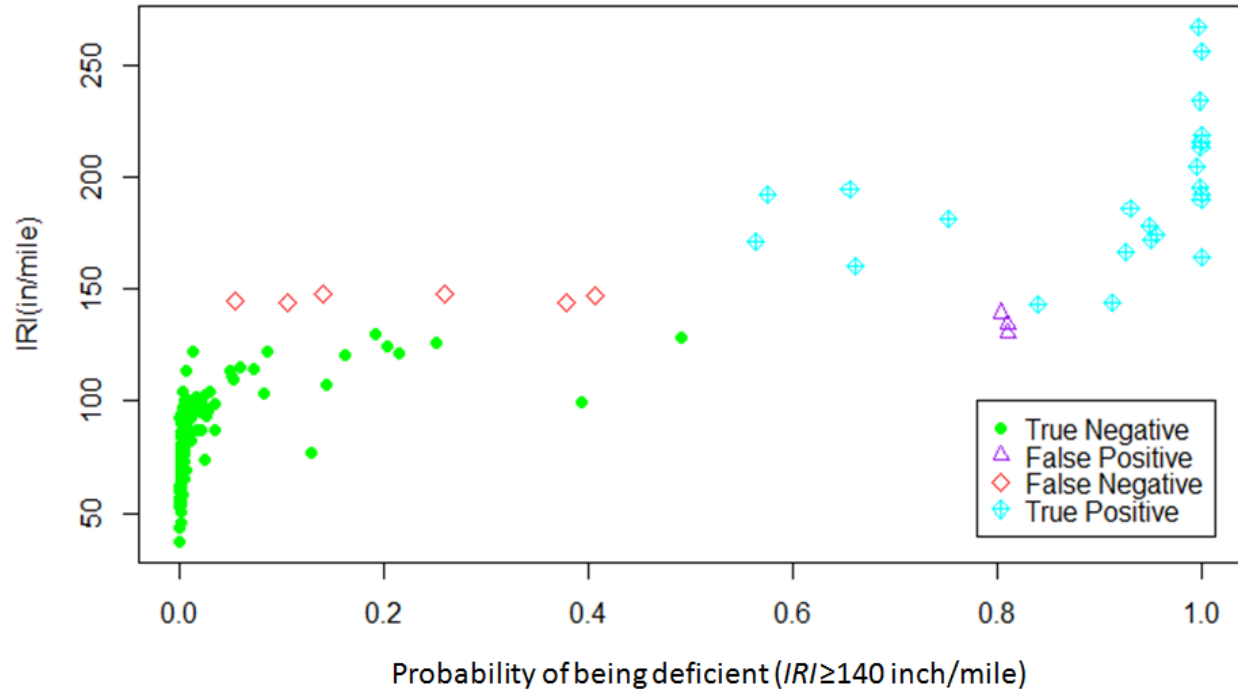
Figure 10. IRI values and the estimated probability
