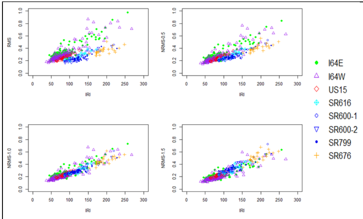
Figure 9. Scatter plots of IRI vs. RMS/NRMS acceleration.
