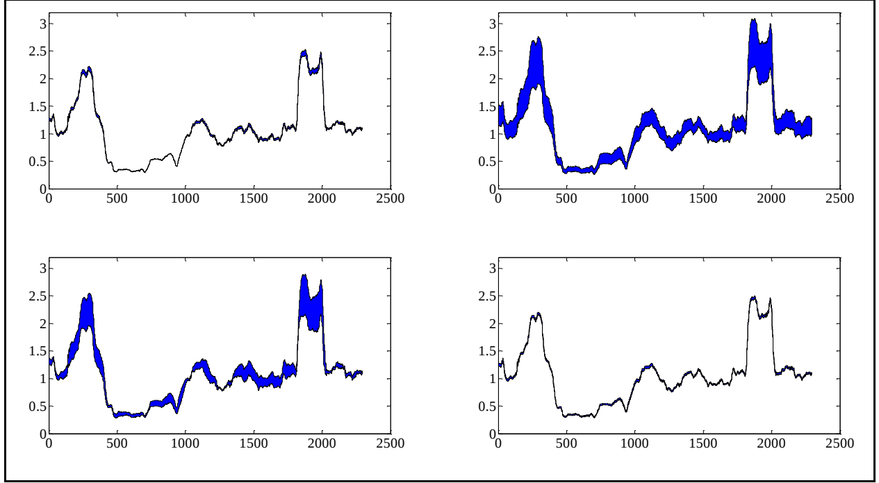
Figure 6. Effect of quarter-car parameters on PVRI; Top Left k_1 ; Top Right: C ; Bottom Left: k_2 ; Bottom Right: \mu
