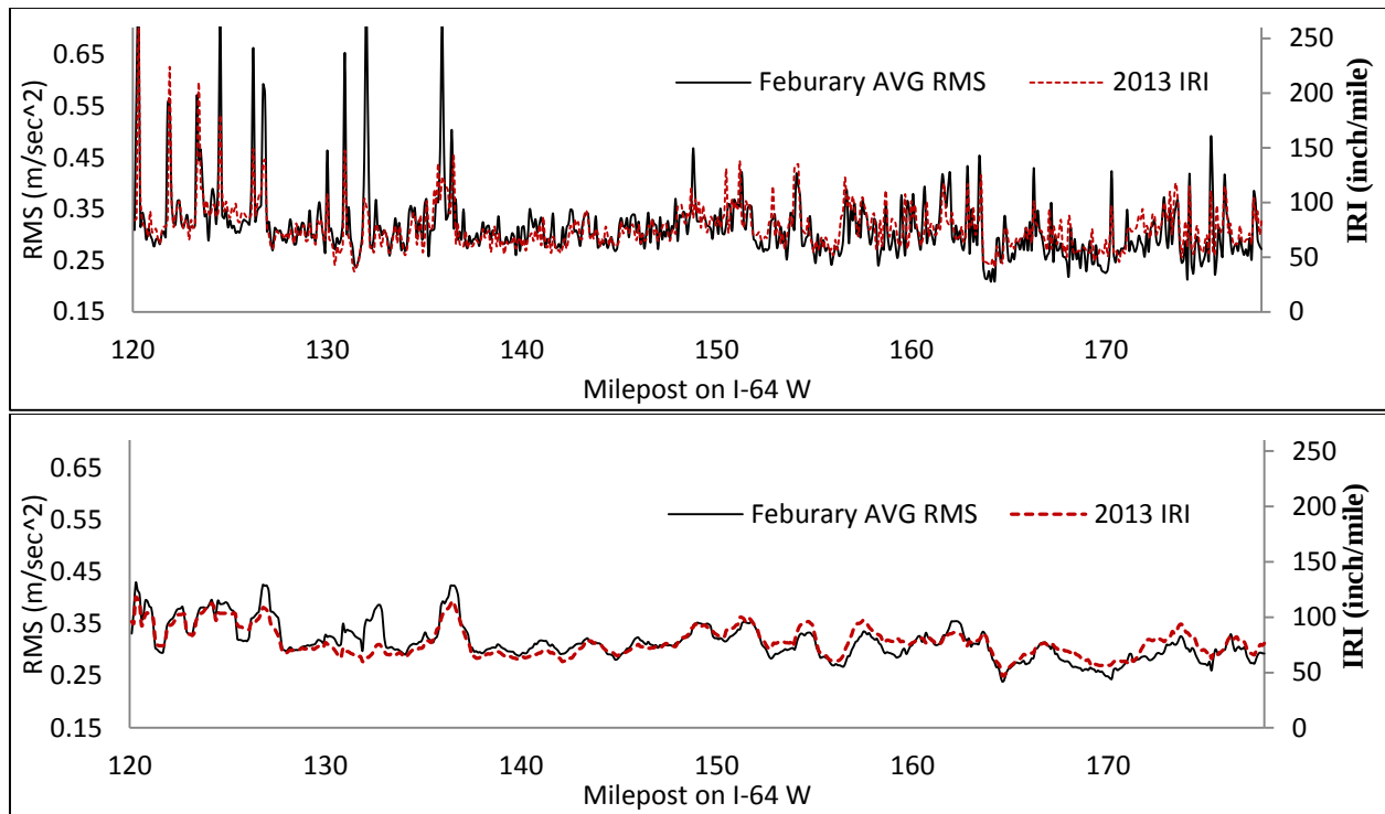
Figure 7. IRI Compared to RMS Acceleration on I-64 W; Top: Original 0.1-mile data; Bottom: Moving average using a 1-mile window.
