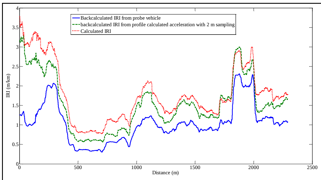
Figure 4. Effect of sampling rate on the calculated IRI.
