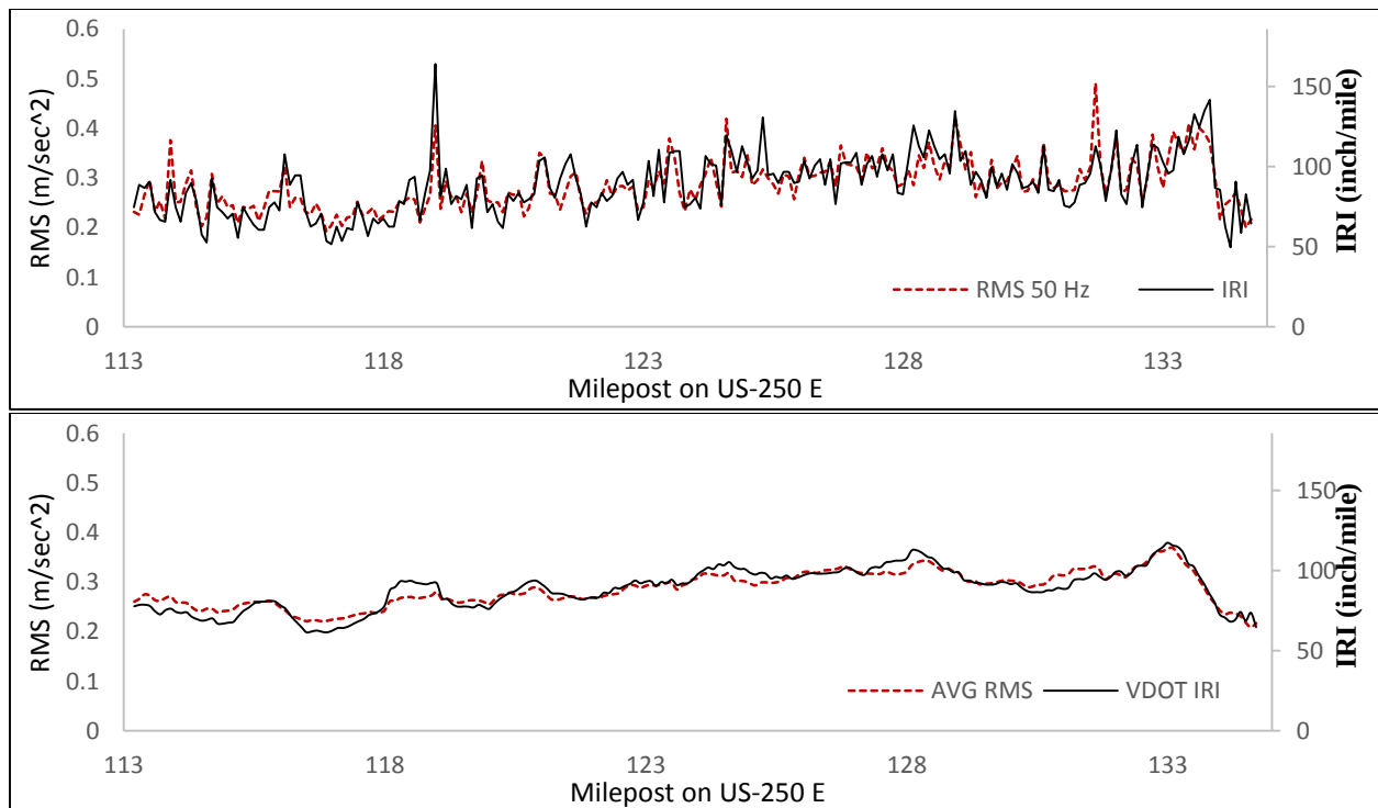
Figure 8. IRI Compared to RMS Acceleration on US-250 E; Top: Original 0.1-mile data; Bottom: Moving average using a 1-mile window
