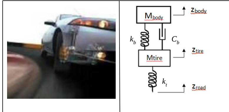
Figure 1. Schematic of quarter-car model used to measure roughness.
