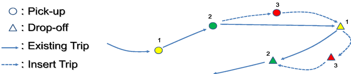
Figure 6 - Insertion algorithm
