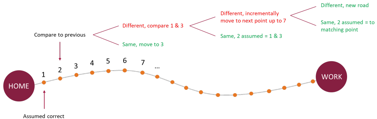
Figure 6. Map matching algorithm.
