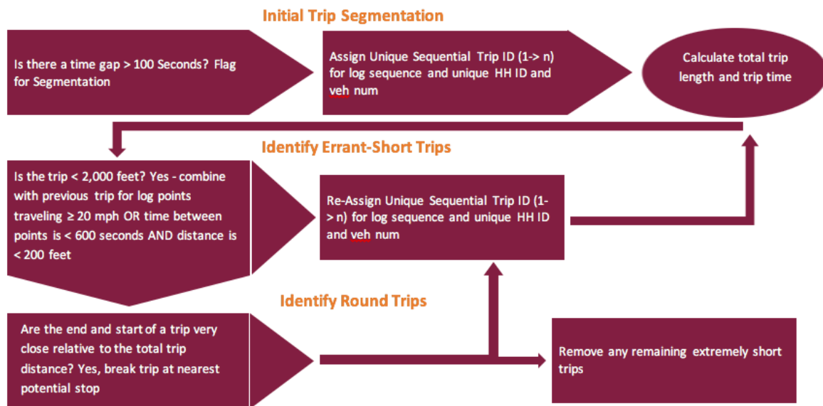
Figure 4. GPS trip segmentation algorithm.
