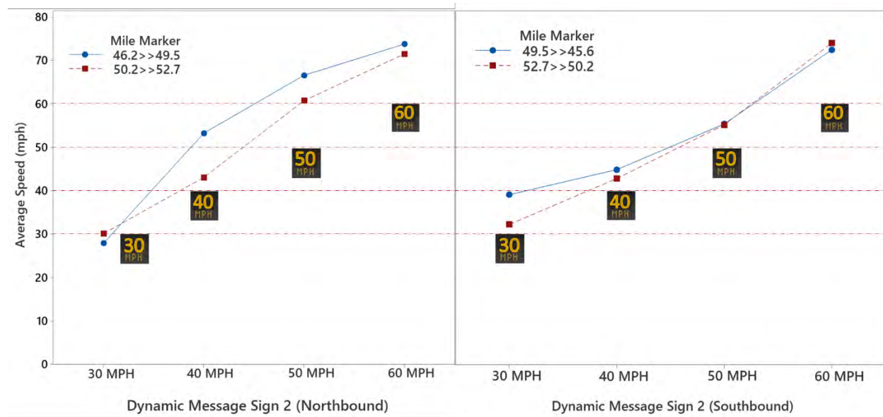
Figure 3-28 Two-way interaction between DMS2 and the aggregated mile markers for both directions on mean speed
