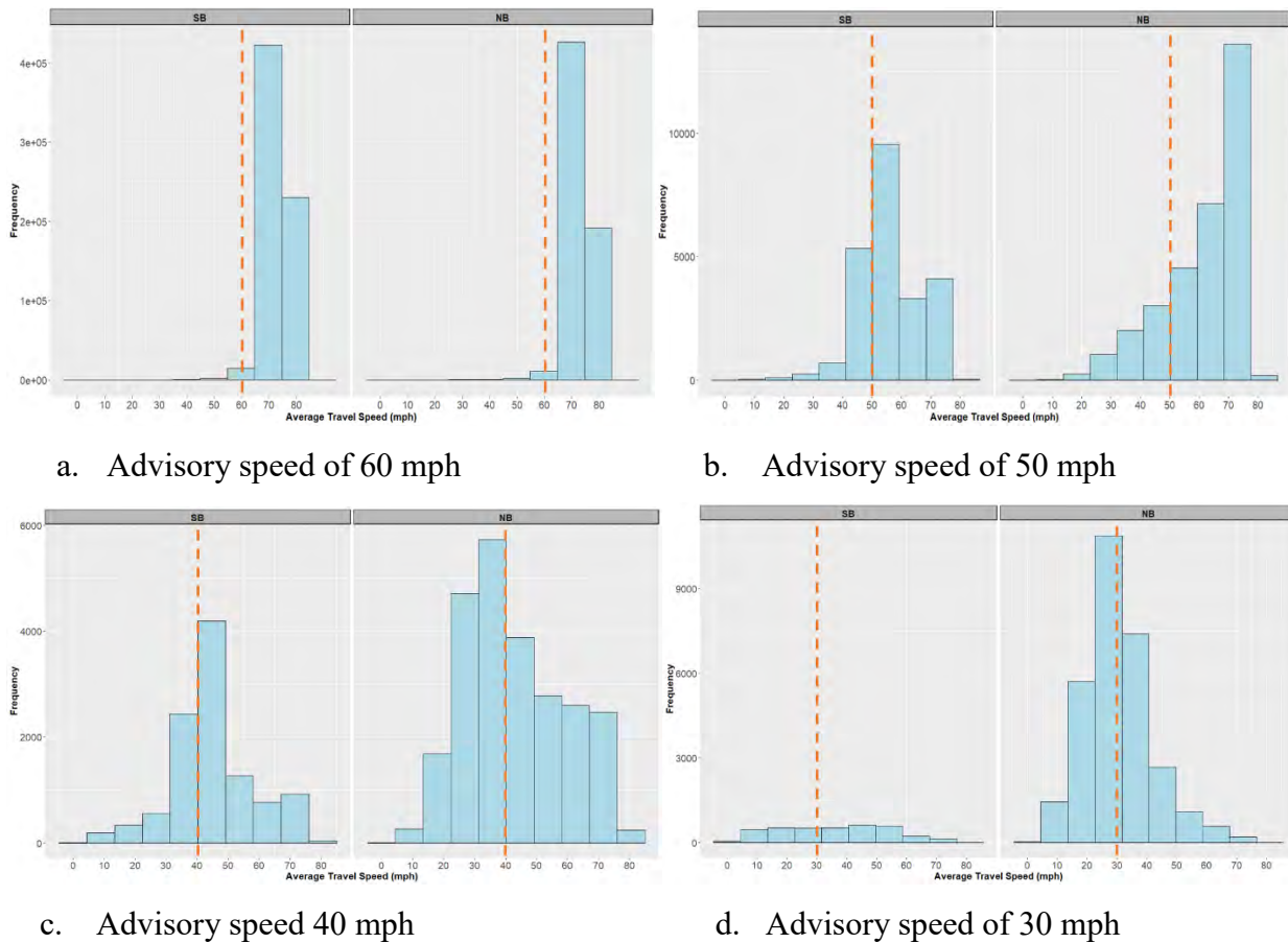
Figure 3-23 Number of observations of actual travel speed under various advisory speeds
