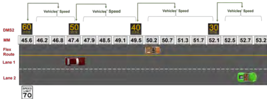
Figure 3-22 Example of travel speed and advisory speed data integration
