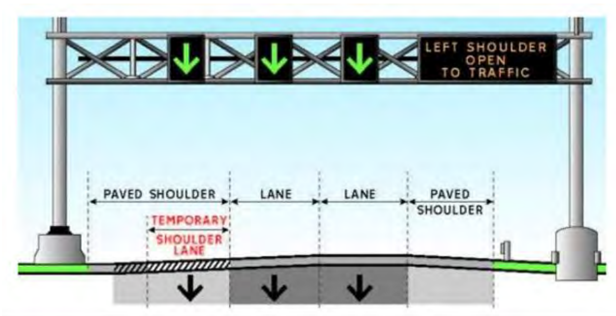
Figure 1-2 US-23 utilizes the inside shoulder as a dynamic lane
