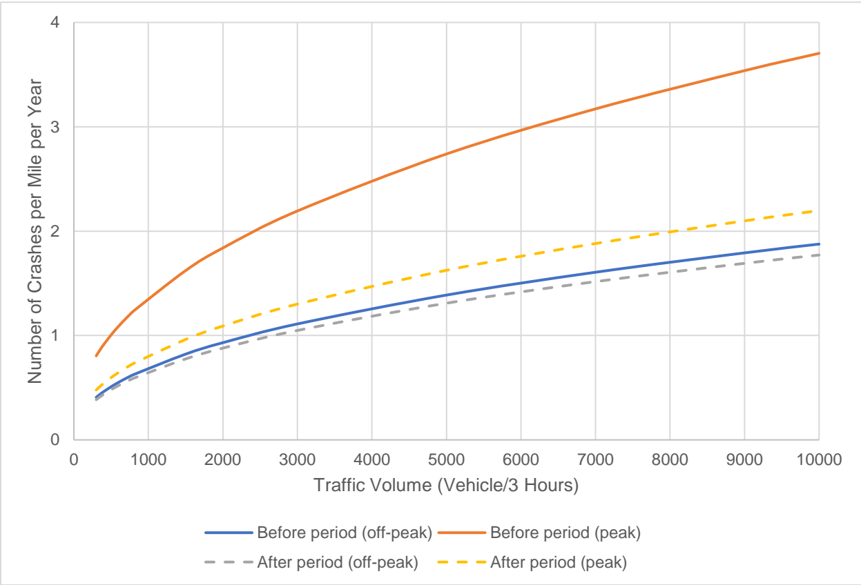
Figure 4-3 Crashes per mile per year by traffic volume on southbound direction
