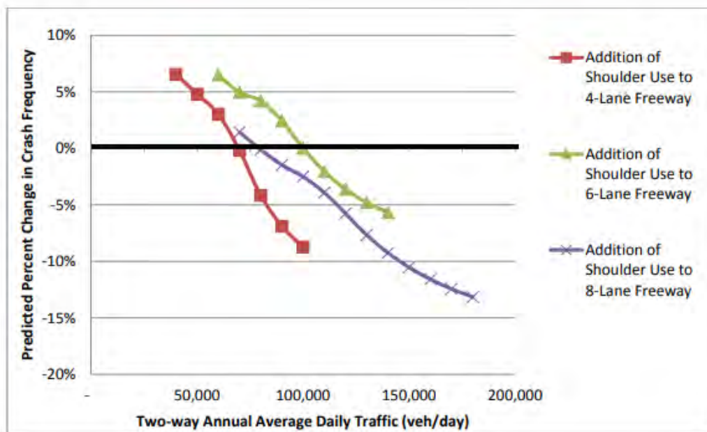
Figure 2-1 Crash frequency for part-time shoulder ATM with narrow lanes
