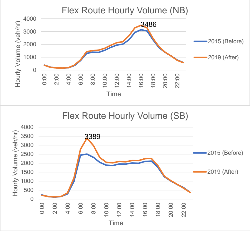
Figure 3-6 Hourly volume of US-23 Flex route
