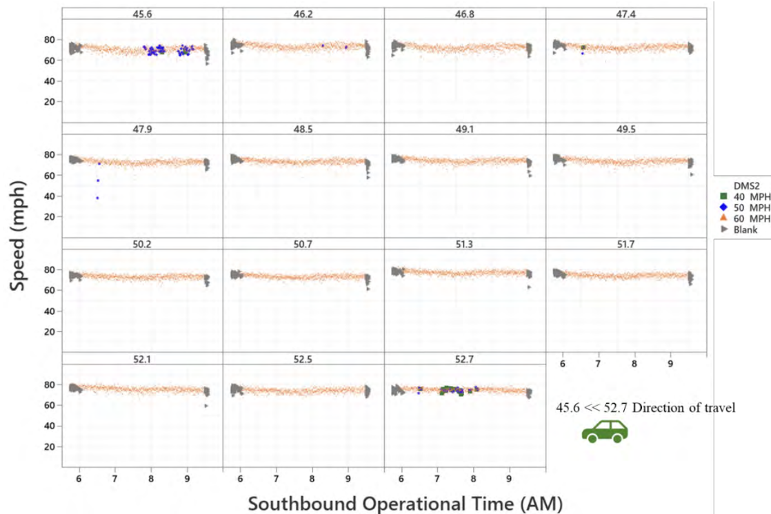
Figure 3-27 Southbound drivers’ speed profile during only weekdays, 15 minutes before the operational time, during, and after
