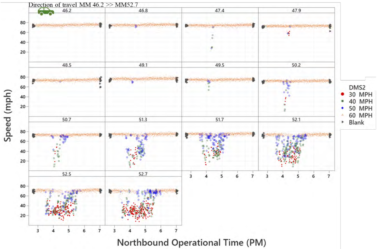
Figure 3-26 Northbound drivers' speed profile during only weekdays, 15 minutes before the operational time, during, and after
