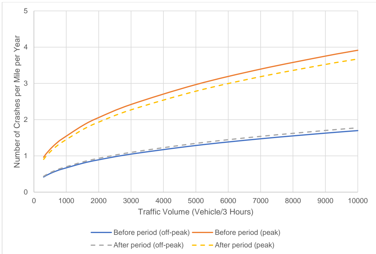
Figure 4-2 Crashes per mile per year by traffic volume on northbound direction
