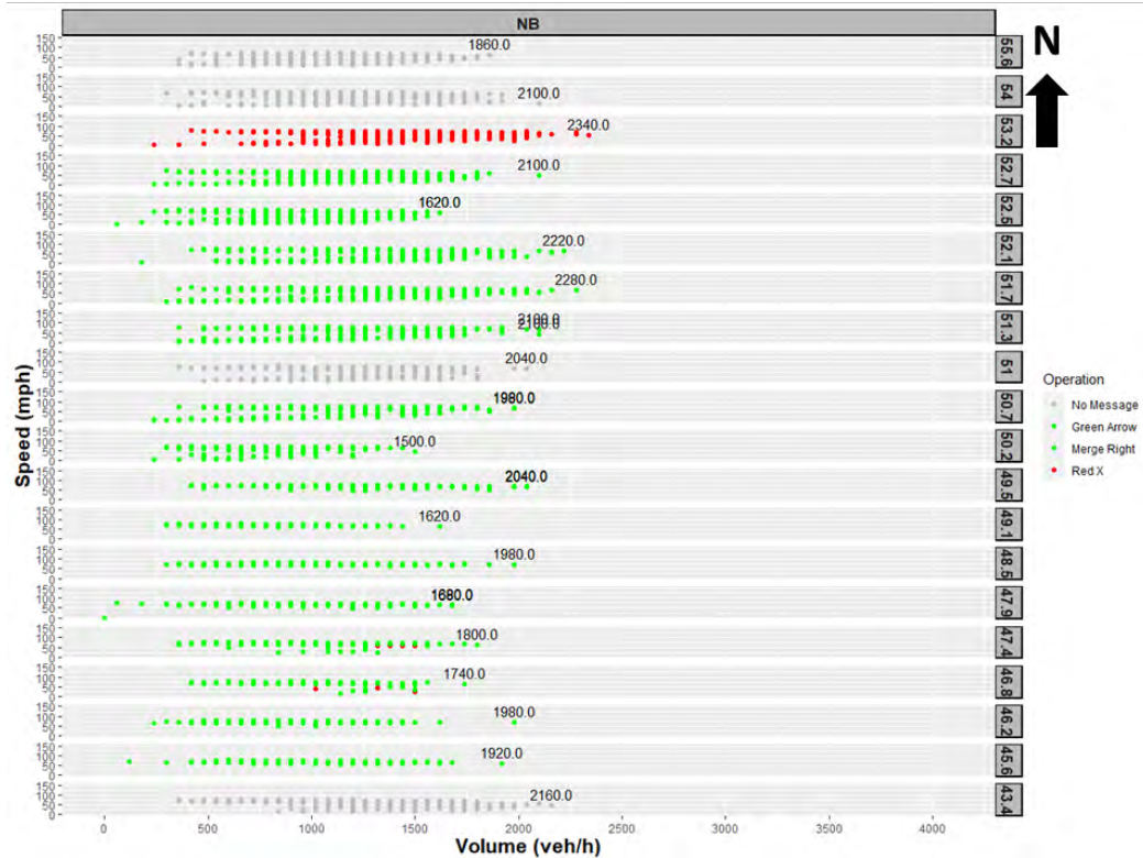
Figure 3-19 Northbound speed - flow curves for US-23 Flex route during weekday peak period on lane-by-lane basis
