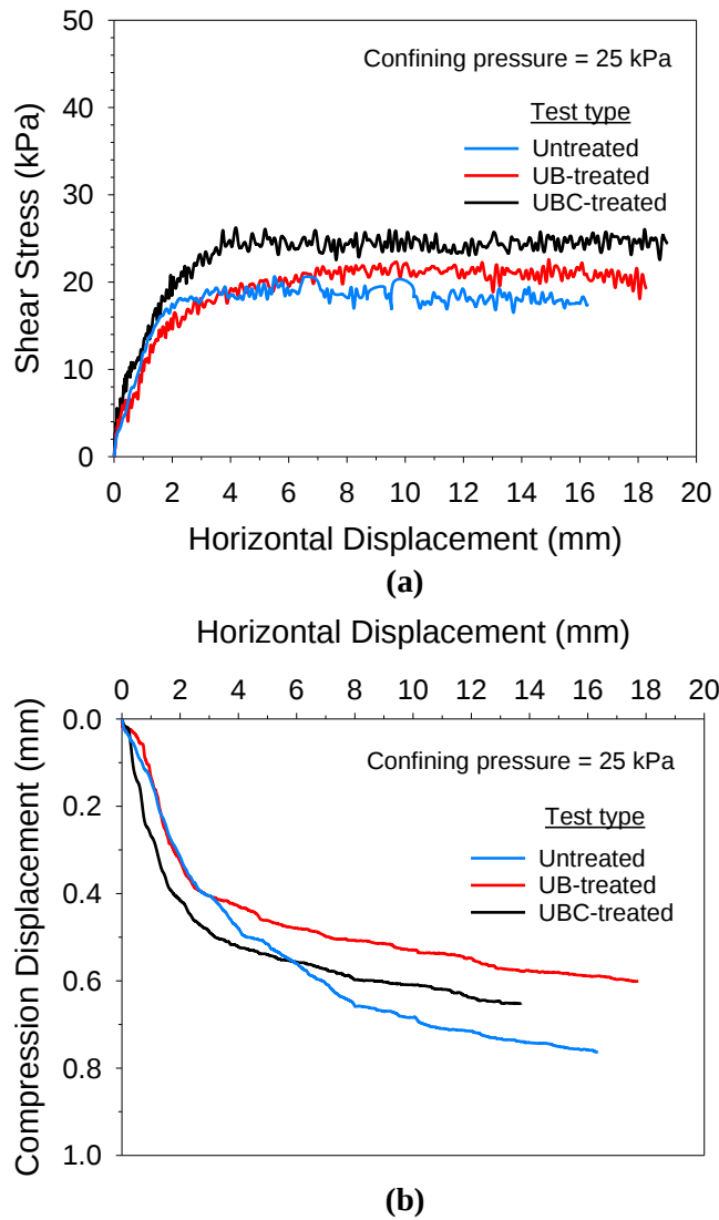
Figure 8. Direct shear test results of the silt samples at the confining pressure of 25 kPa: (a) shear stress versus horizontal displacement and (b) compression displacement versus horizontal displacement.
