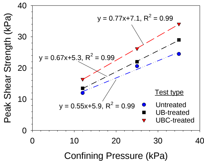
Figure 11. Peak failure envelopes of untreated, UB-treated, and UBC-treated samples.
