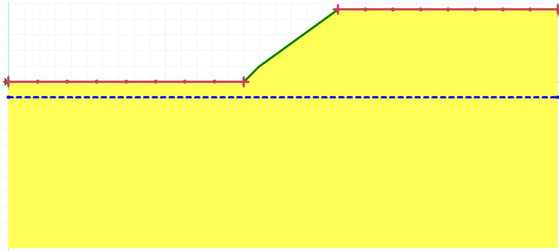
Figure 6. Geometry of the embankment slope in SLOPE/W.
