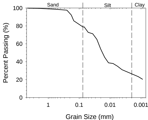
Figure 1. Particle size distribution of the silt.
