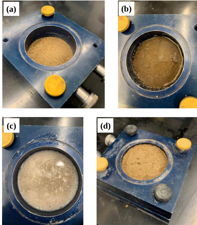
Figure 3. Direct shear sample preparation: (a) compacted silt in the bottom split box, (b) urea medium suspended with bacteria cells or deionized water filled in the split box, (c) cementation medium added into the split box, and (d) compacted silt added into the top split box.
