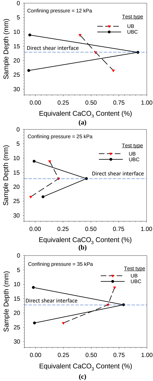
Figure 10. Equivalent \text{CaCO}_3 content distributions along the sample depth at confining pressures of: (a) 12 kPa, (b) 25 kPa, and (c) 35 kPa.
