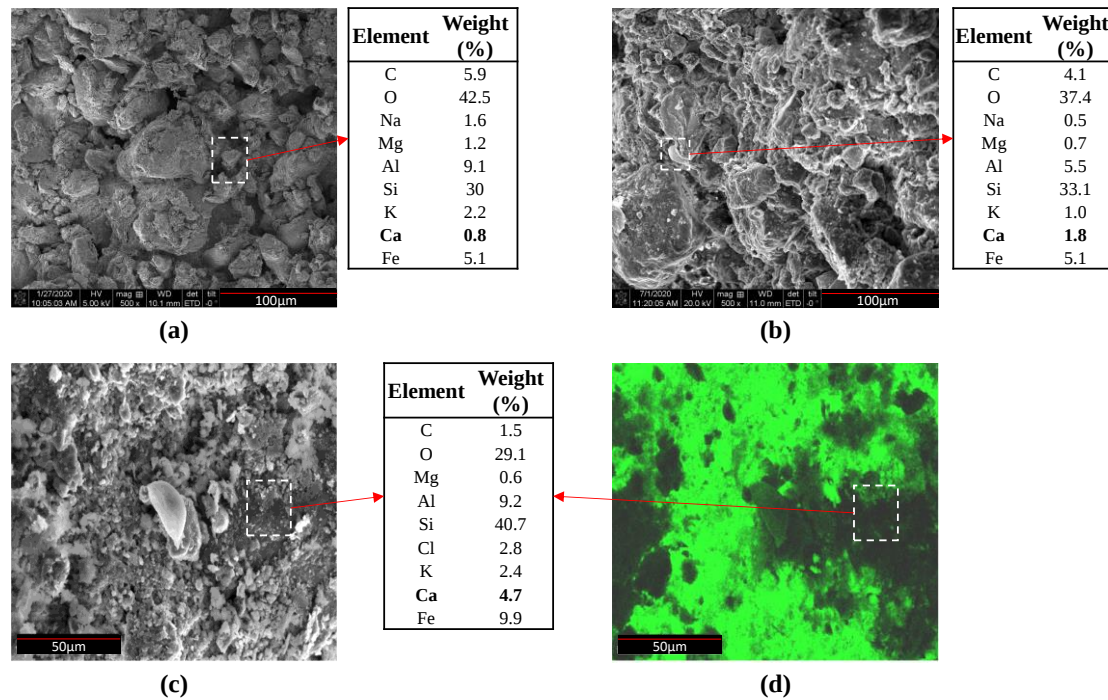
Figure 12. SEM imaging and EDS results of (a) untreated, (b) UB-treated, and (c) UBC-treated samples; and (d) calcium element mapping of the UBC-treated sample.
