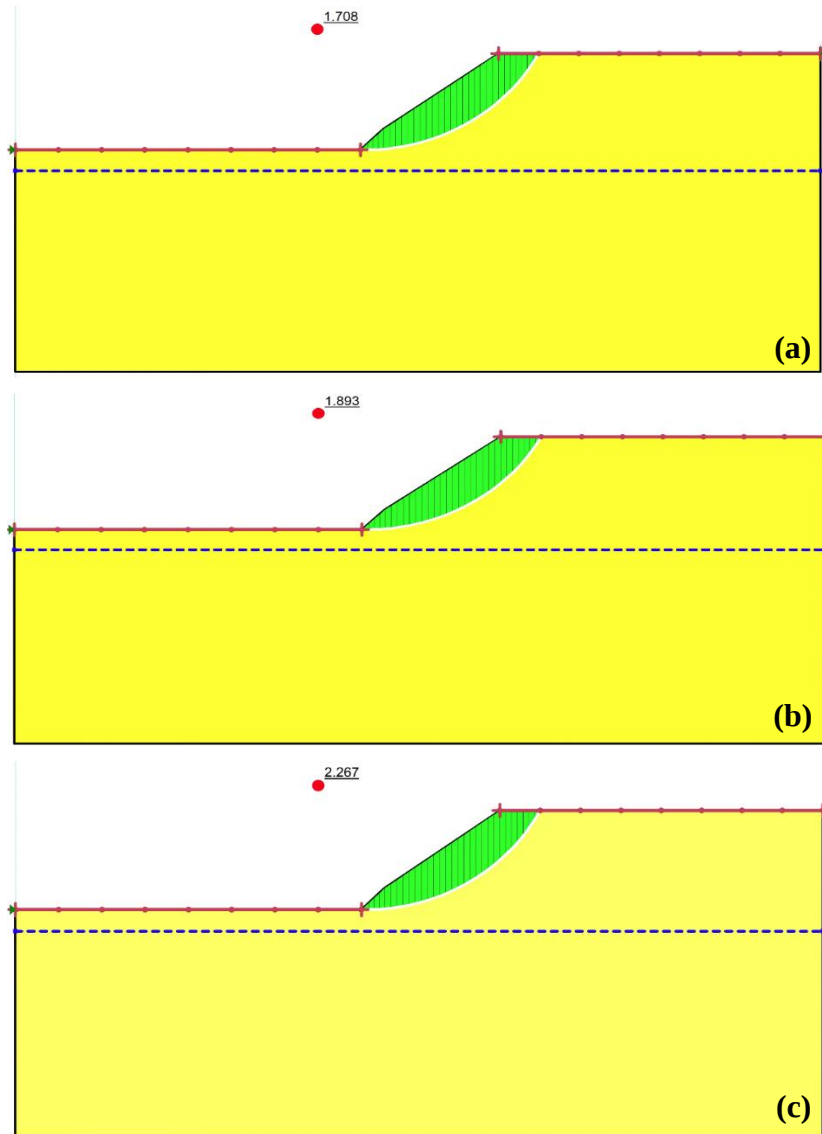
Figure 21. SLOPE/W analysis results: (a) untreated slope, (b) UB-treated slope, and (c) UBC-treated slope.
