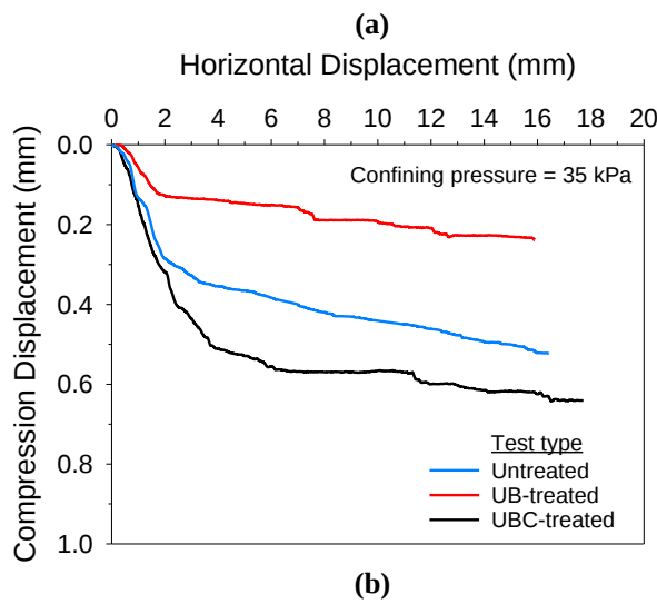
Figure 9. Direct shear test results of the silt samples at the confining pressure of 35 kPa: (a) shear stress versus horizontal displacement and (b) compression displacement versus horizontal displacement.
