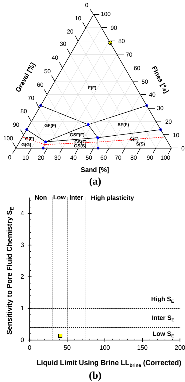
Figure 2. Revised soil classification system (RSCS) results: (a) soil-specific triangular chart and (b) fines classification chart.
