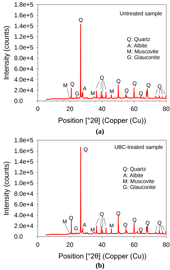
Figure 13. X-Ray Diffraction (XRD) patterns of (a) untreated and (b) UBC-treated samples.
