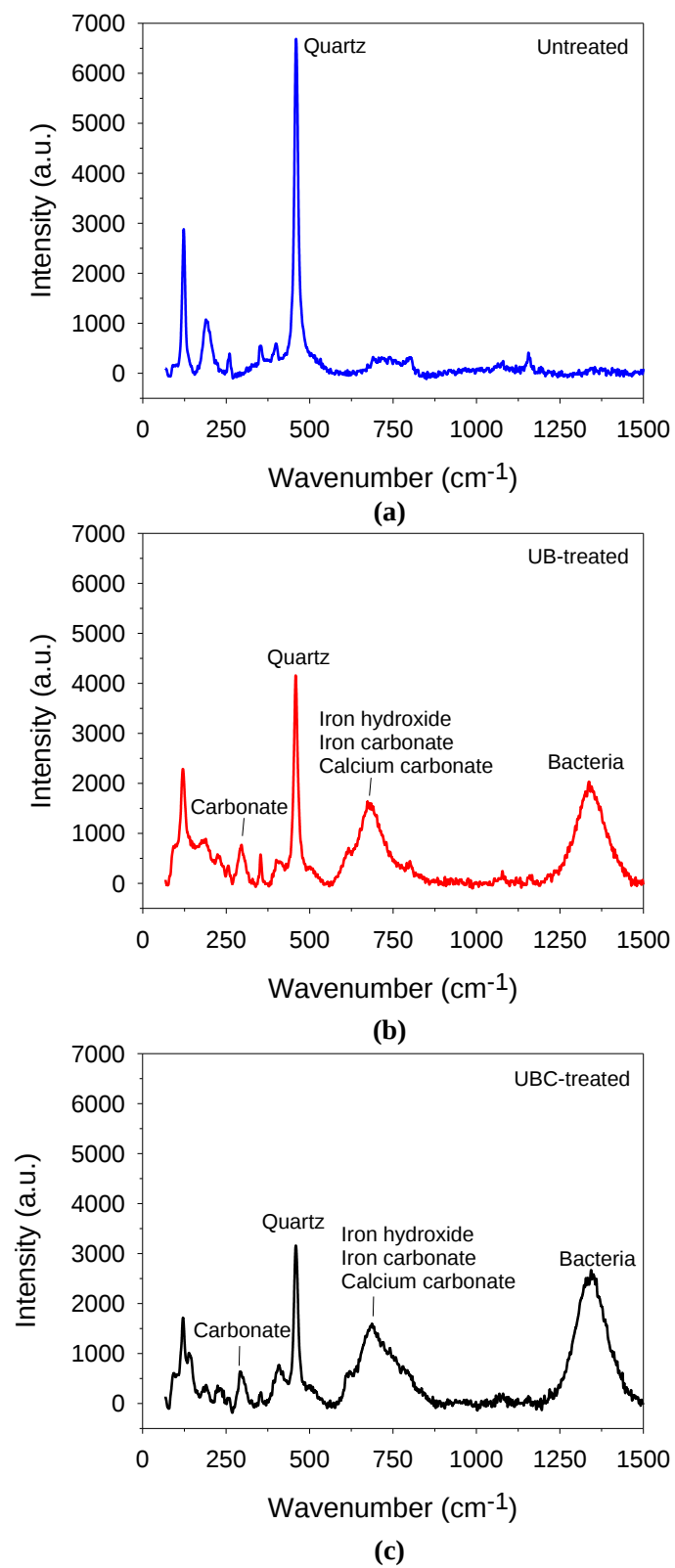
Figure 14. Raman spectra of (a) untreated, (b) UB-treated, and (c) UBC-treated samples.
