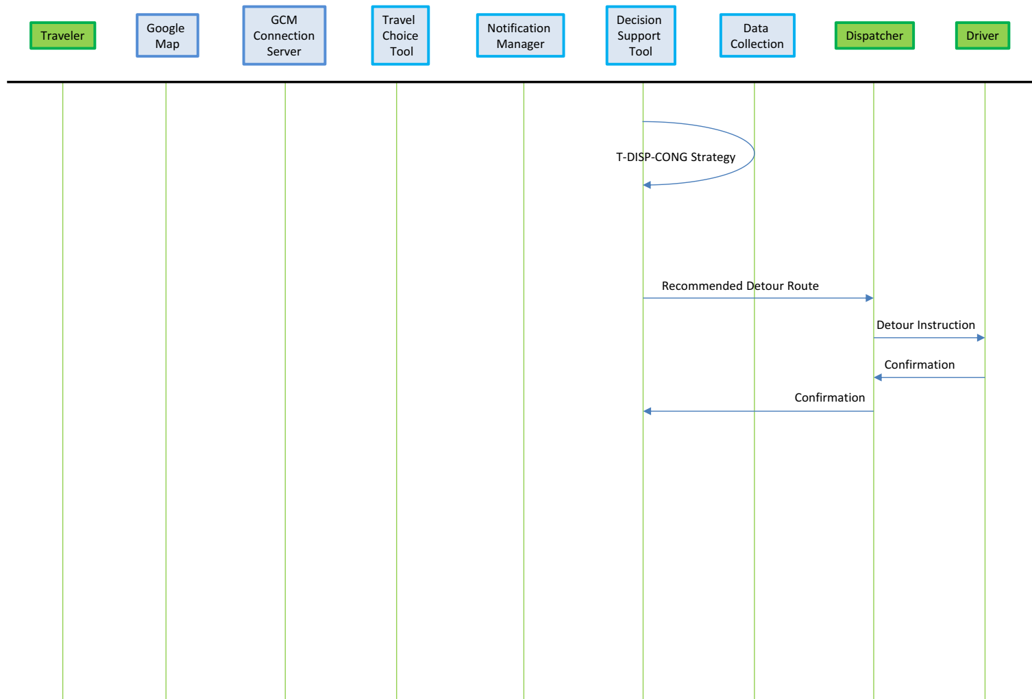
Figure 7. Sequence Diagram of Scenario 2(a) Route Deviation to Avoid Congestion
