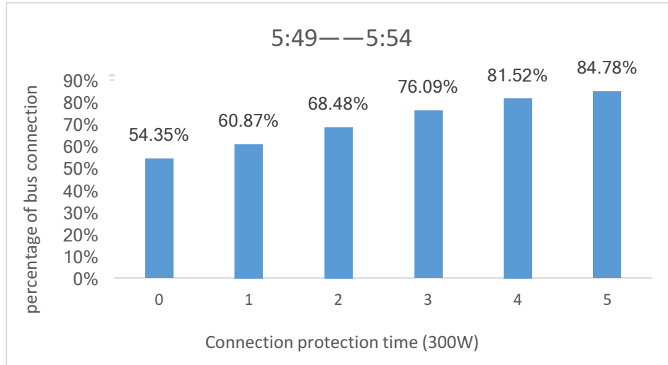
Figure 29. Connection success rate of T-CONNECT of 380W to 300W (trip 1090) at Hillcrest P & R
