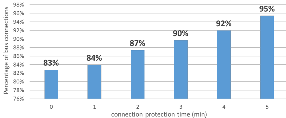
Figure 31. Connection success rate of T-CONNECT of 388W to 300W (trip 1087) at Hillcrest P & R
