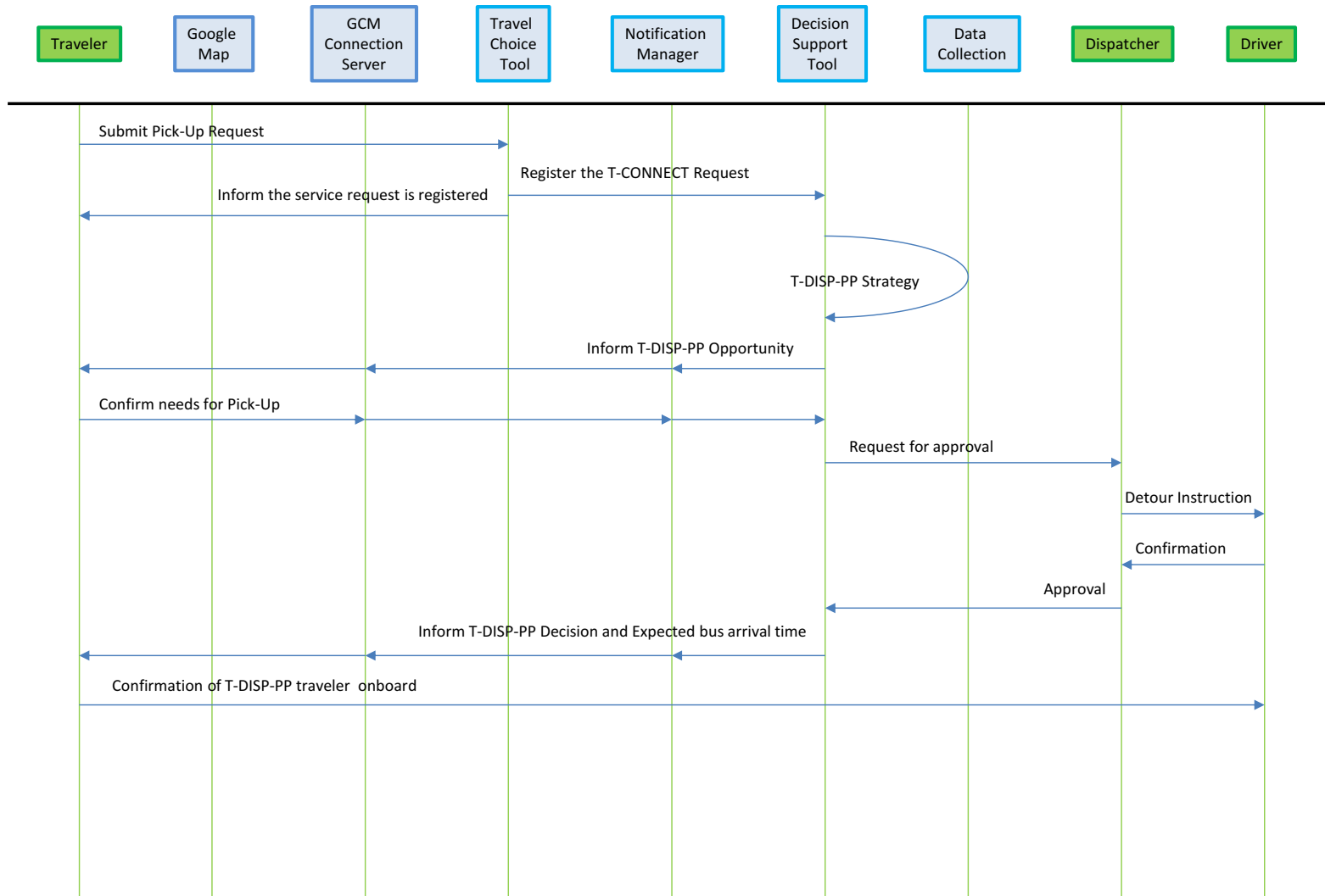
Figure 8. Sequence Diagram of Scenario 2(b) Route Deviation to Pick Up Passenger
