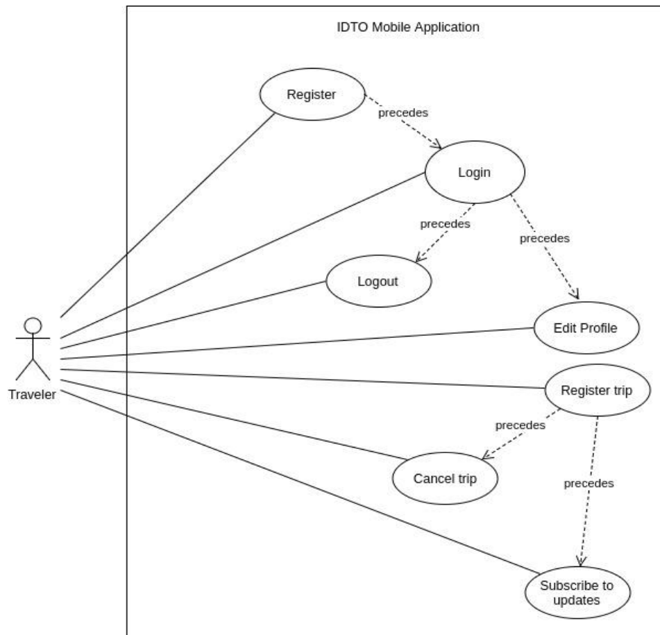
Figure 16. Interactions on the Mobile App Interface
