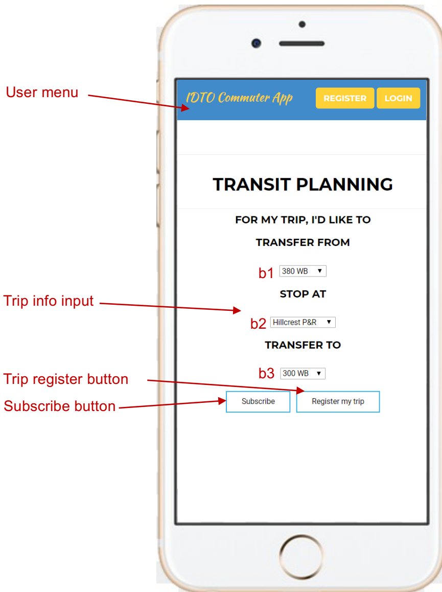
Figure 15. Mobile App Interface
