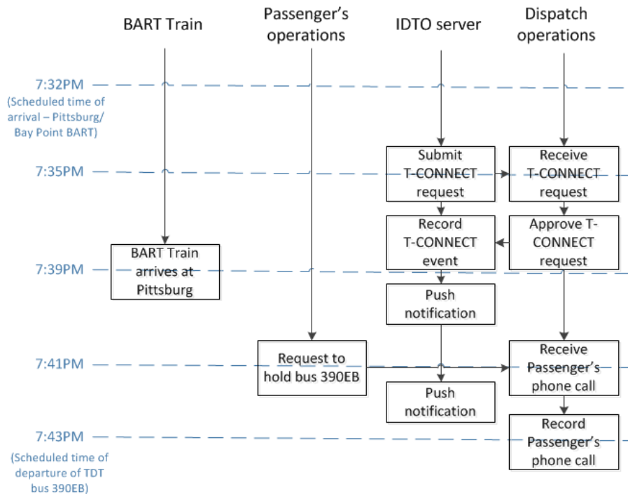
Figure 39. Parallel testing flow of T-CONNECT
