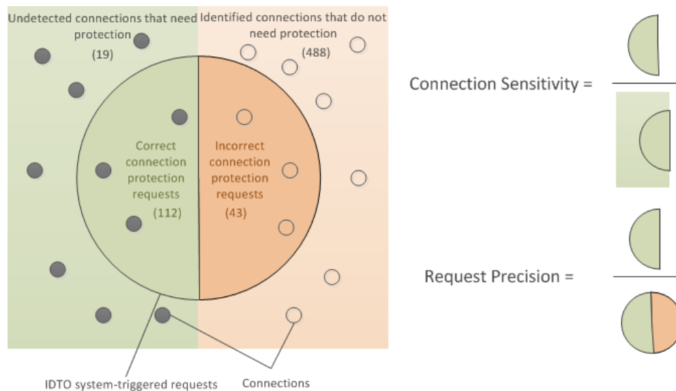
Figure 34. Definitions of connection sensitivity and request precision
