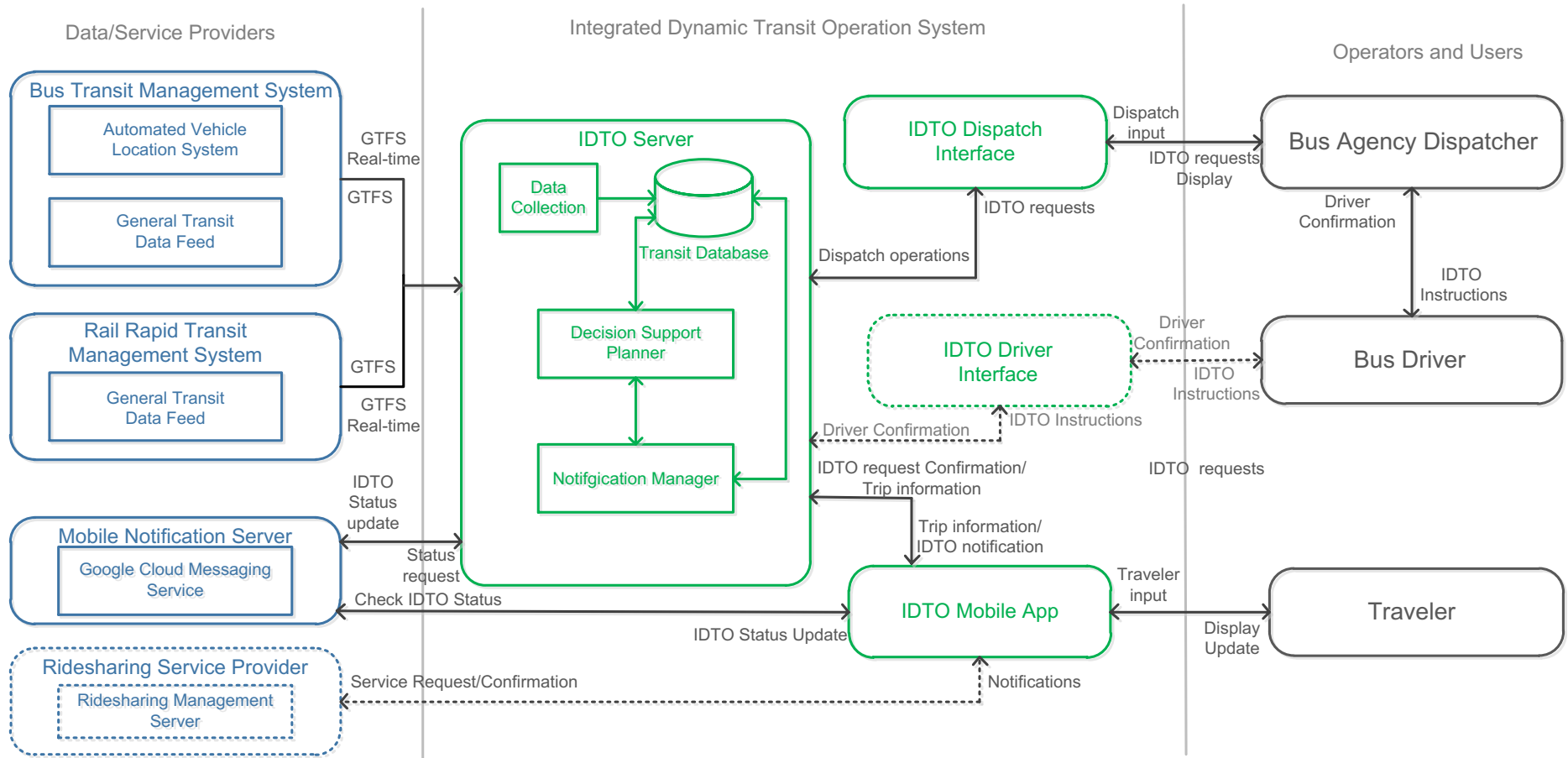
Figure 5. IDTO System Architecture 5
