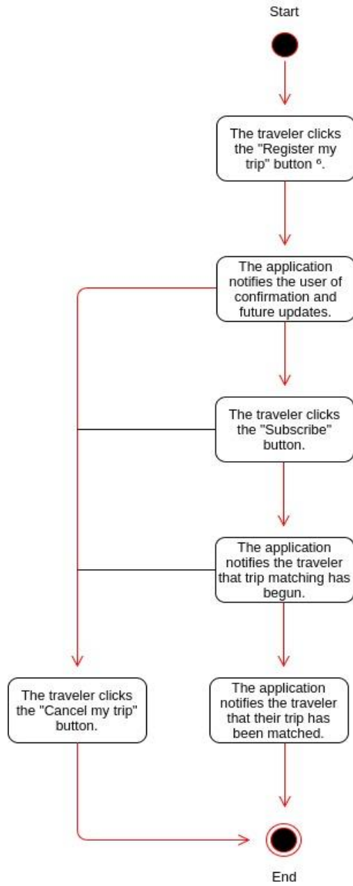
Figure 21. Activity Graph of register and subscribe a trip
