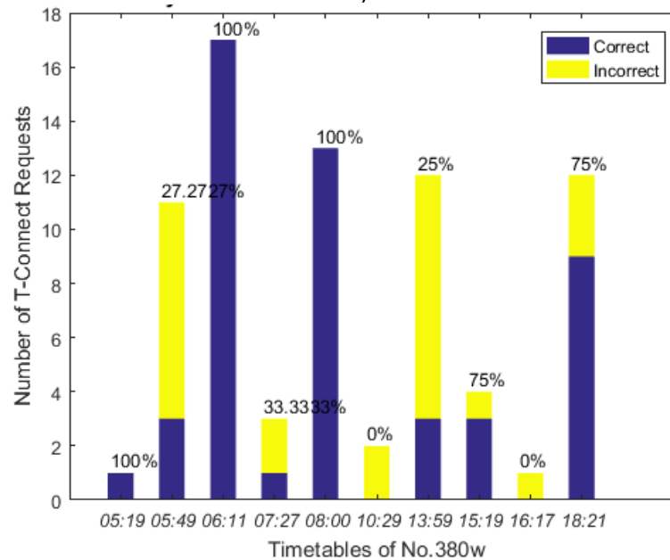
Figure 36. a) Connection sensitivity and b) request precision of T-Connect requests involving bus No. 380w
