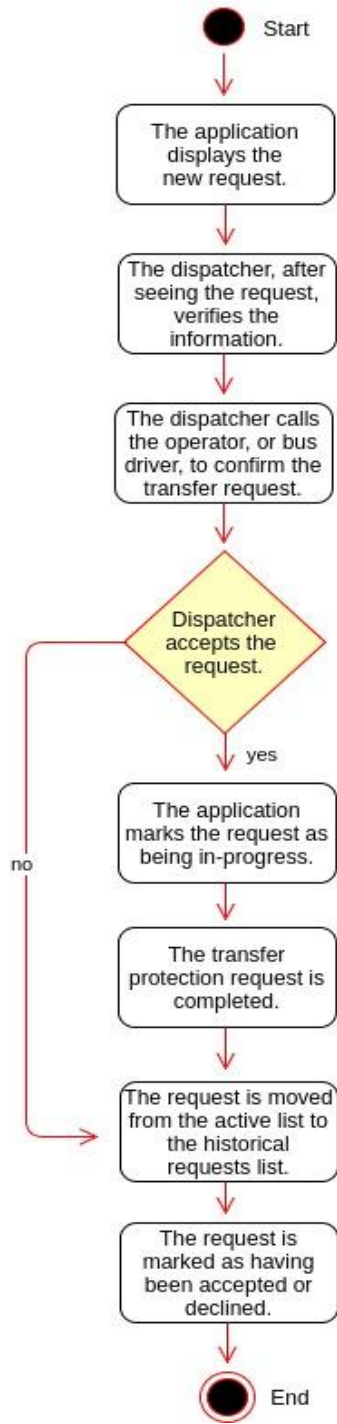
Figure 14. Activity Graph of Dispatcher Interface
