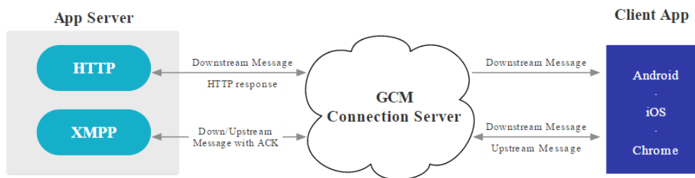
Figure 11. GCM mechanism
