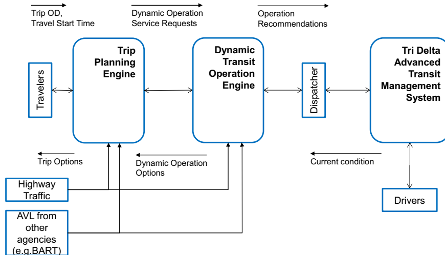
Figure 3. IDTO Conceptual Architecture
