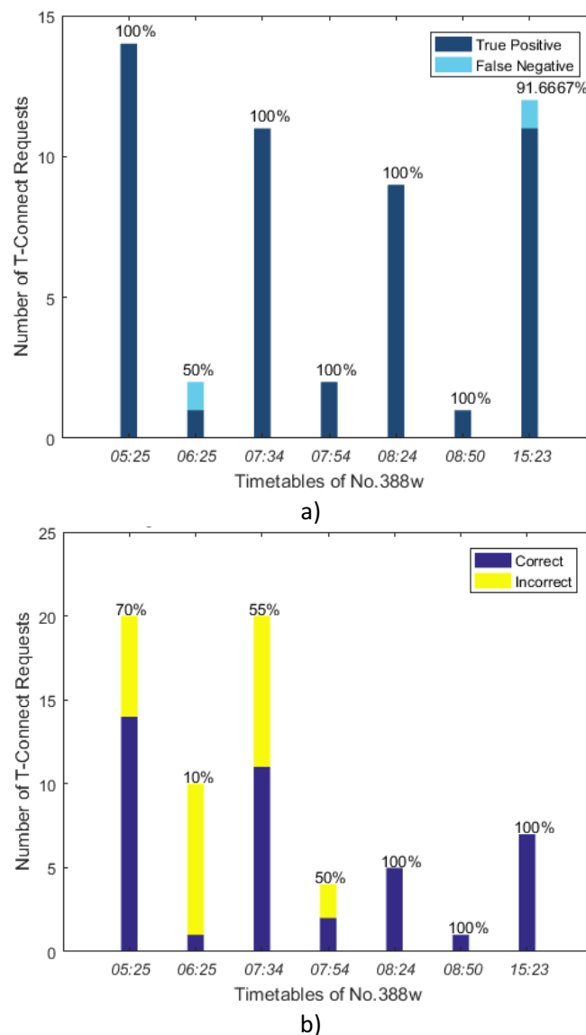
Figure 37. a) Connection sensitivity and b) request precision of T-Connect requests involving bus No. 388w
