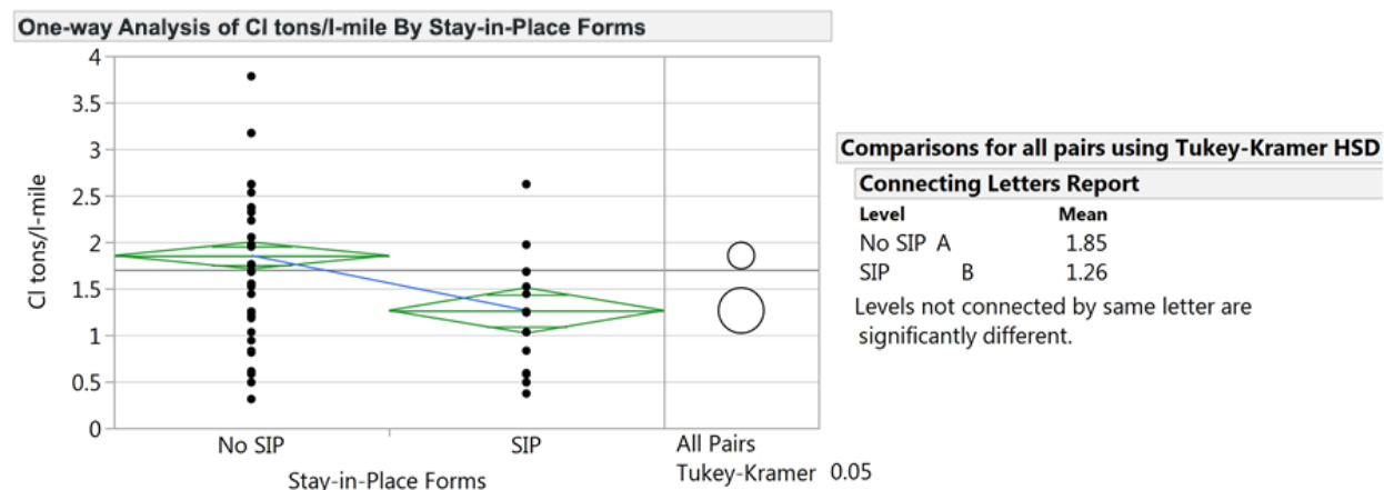
Figure 24. One-way Analysis of Rate of Chloride Application by Presence of Stay-in-Place Forms. SIP = decks with stay-in-place forms; No SIP = decks without stay-in-place forms.
