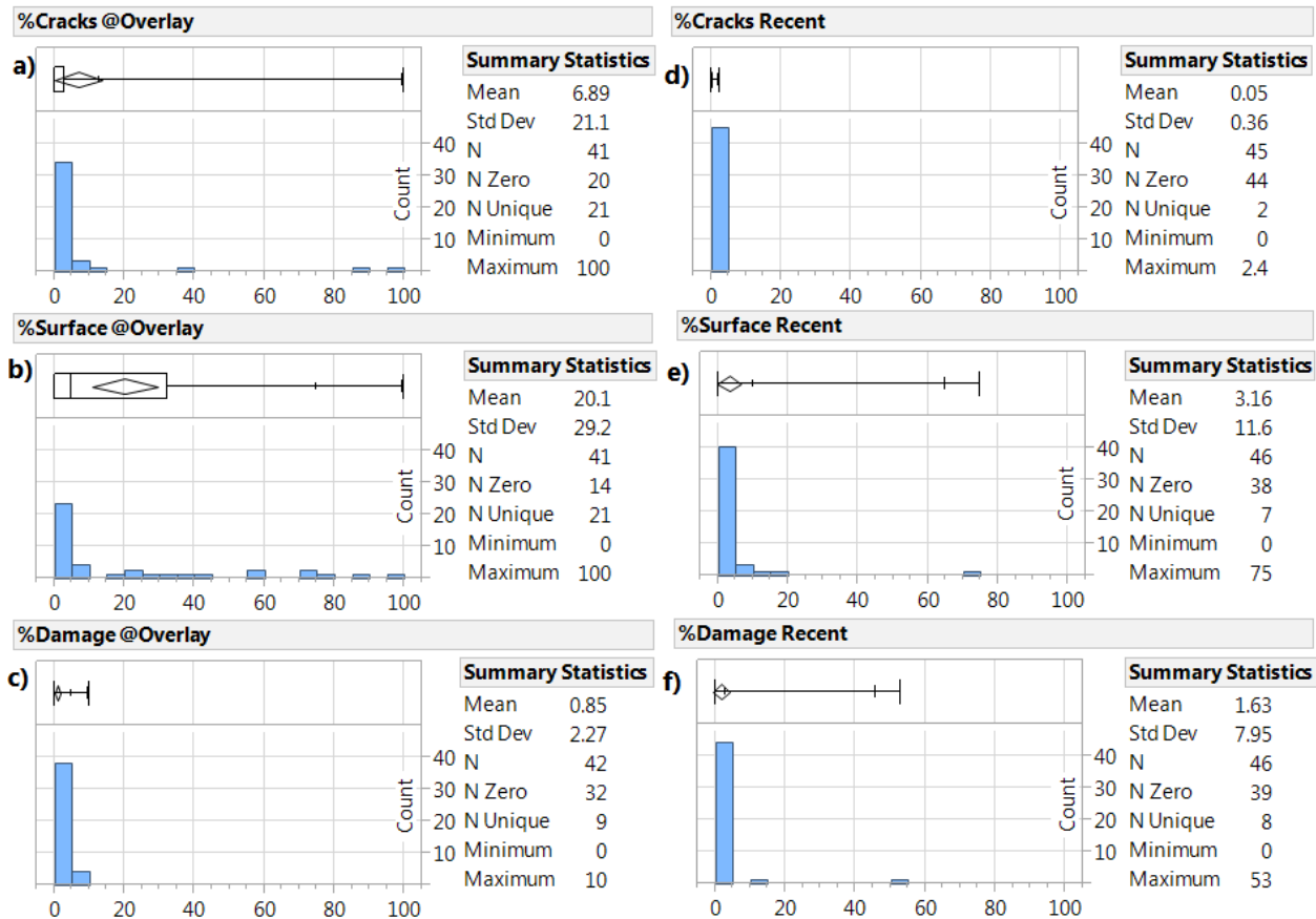
Figure 12. Histograms for Epoxy Concrete Overlays: (a) %Cracks at Overlay; (b) %Surface at Overlay; (c) %Damage at Overlay; (d) %Cracks Recent; (e) %Surface Recent; (f) %Damage Recent
