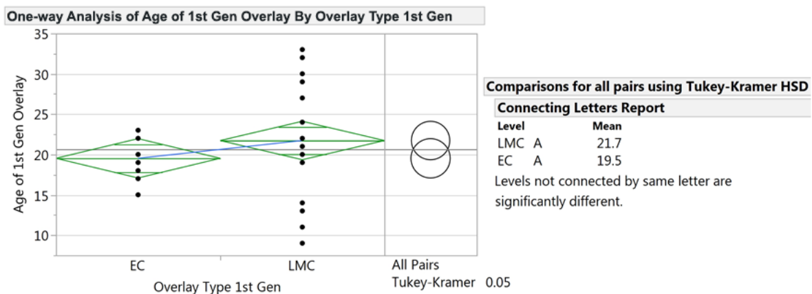
Figure 29. One-way Analysis of Age of First-Generation Overlay and Corresponding Overlay Type. EC = epoxy concrete; LMC = latex-modified concrete.
