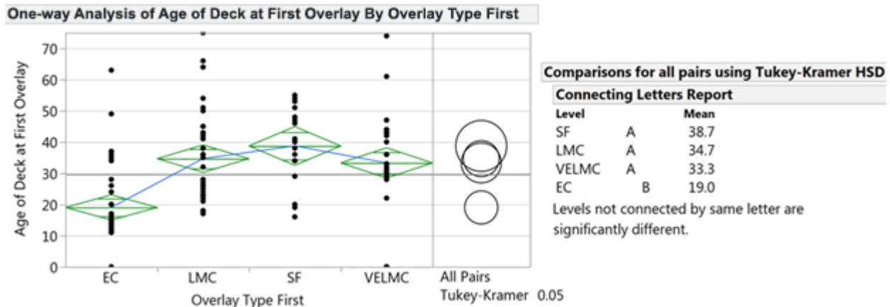
Figure 19. One-way Analysis of Age of Bridge Decks at First Overlay and Overlay Type. EC = epoxy concrete; SF = silica fume; LMC = latex-modified concrete; VELMC = very-early-strength latex-modified concrete.
