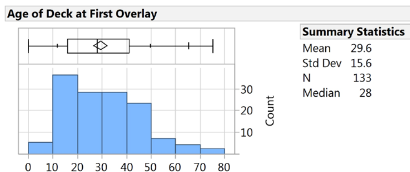
Figure 16. Histogram of Age of Bridge Deck at Time of First Overlay
