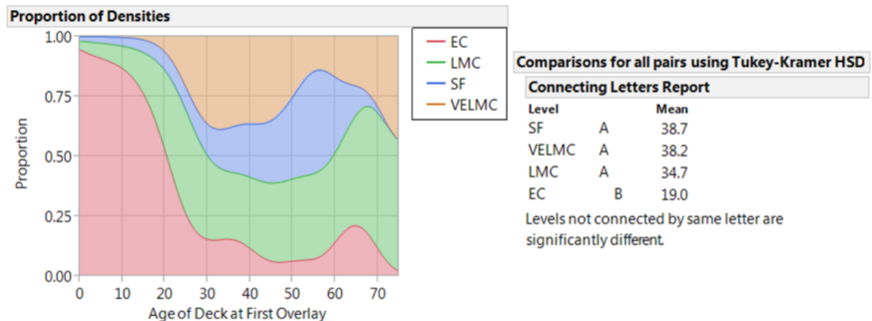
Figure 20. Age of Bridge Decks at First Overlay Excluding Anomalies. EC = epoxy concrete; SF = silica fume; LMC = latex-modified concrete; VELMC = very-early-strength latex-modified concrete.
