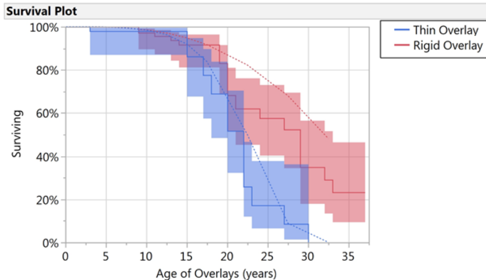
Figure 33. Kaplan-Meier Survival Plot for Age of Thin and Rigid Overlays
