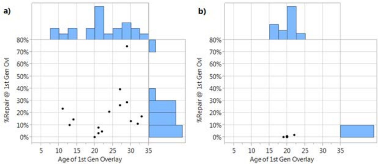
Figure 41. Surface Area Repaired at Time of First-Generation Overlay: (a) latex-modified concrete overlay only; b) epoxy concrete overlay
