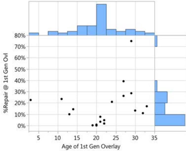
Figure 40. Surface Area Repaired at Time of First-Generation Overlay
