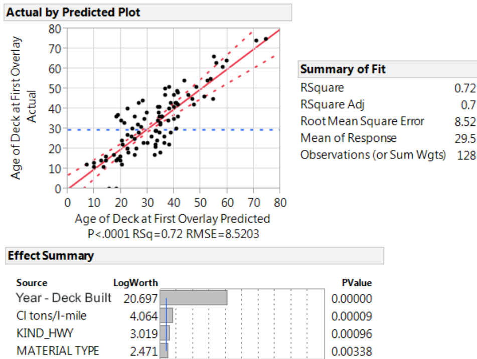
Figure 26. Multiple Regression Model: Age of Bridge Deck at First Overlay
