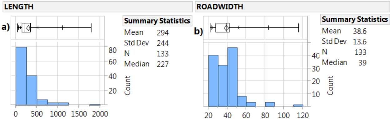
Figure 4. Histograms of (a) Length and (b) Road Width of Bridges
