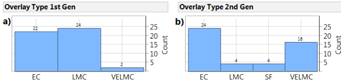
Figure 28. Histograms of Frequency of Overlay Types: (a) first-generation overlay; (b) second-generation overlay. EC = epoxy concrete; SF = silica fume; LMC = latex-modified concrete; VELMC = very-early-strength latex-modified concrete.
