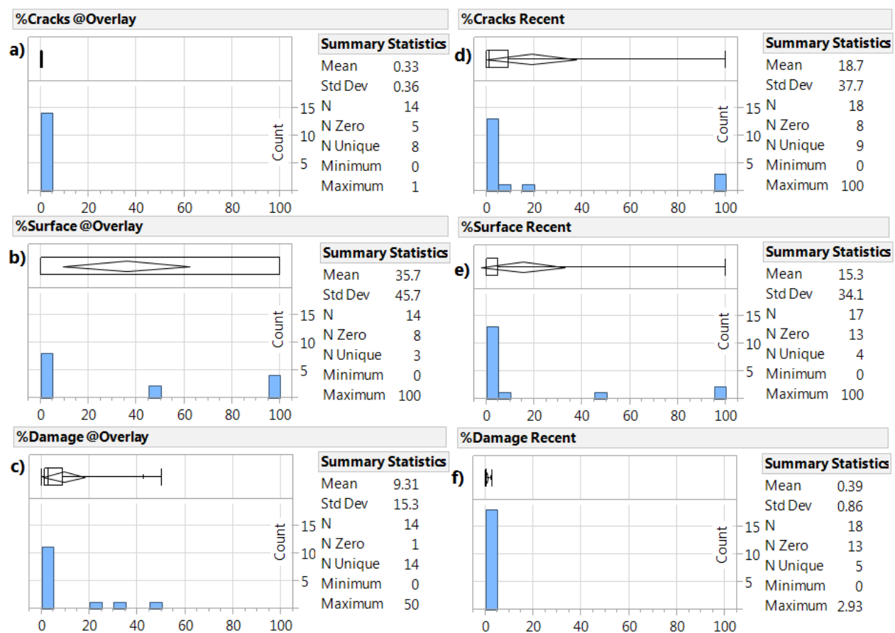
Figure 13. Histograms for Latex-Modified Concrete Overlays: (a) %Cracks at Overlay; (b) %Surface at Overlay; (c) %Damage at Overlay; (d) %Cracks Recent; (e) %Surface Recent; (f) %Damage Recent
