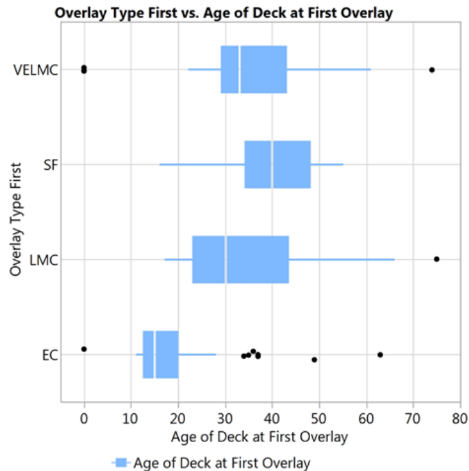
Figure 18. Age of Bridge Decks at First Overlay and Corresponding Overlay Type. VELMC = very-early-strength latex-modified concrete; SF = silica fume; LMC = latex-modified concrete; EC = epoxy concrete.
