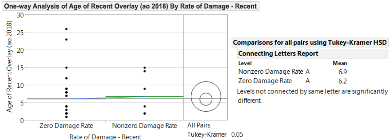
Figure 36. One-way Analysis of Age of Epoxy Concrete Overlays and Rate of Overlay Damage
