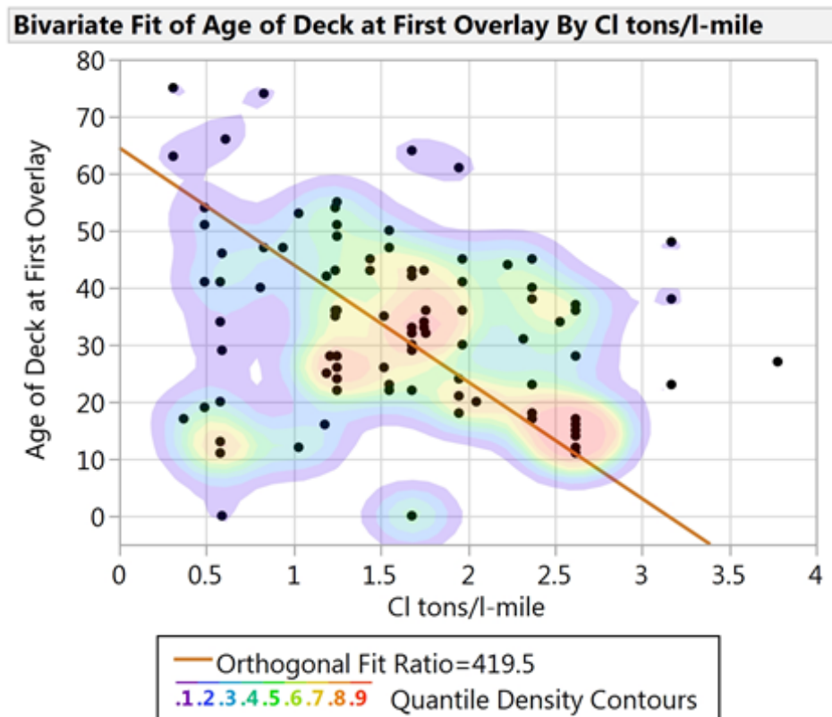
Figure 25. Relationship Between Age of Bridge Deck at First Overlay and Rate of Chloride Application
