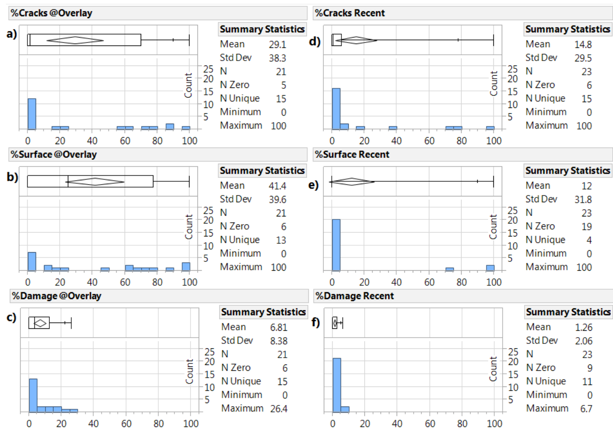
Figure 14. Histograms for Silica Fume Overlays: (a) %Cracks at Overlay; (b) %Surface Wear at Overlay; (c) %Damage at Overlay; (d) %Cracks Recent; (e) %Surface Wear Recent; (f) %Damage Recent
