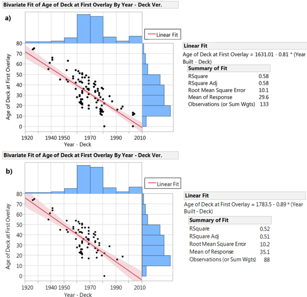
Figure 21. Relationship Between Age of Bridge Deck at First Overlay and Year of Deck Construction: (a) all decks under study; (b) excluding epoxy concrete overlays
