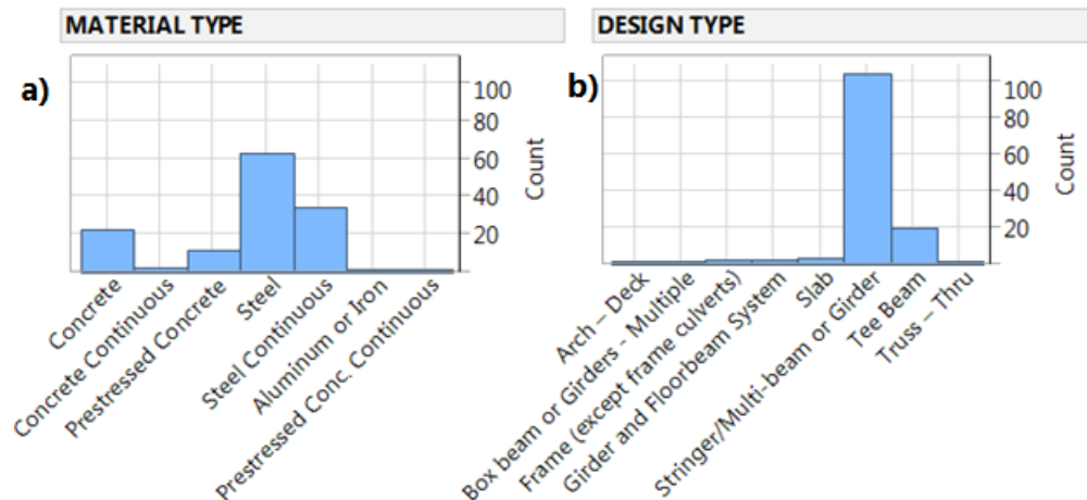
Figure 5. Histograms of (a) Material Type and (b) Design Type of Bridges
