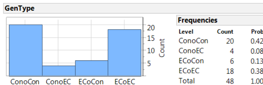
Figure 31. Histogram of Multi-Generational Overlay Profiles. ConoCon = concrete overlay replaces concrete overlay; ConoEC = concrete overlay replaces epoxy concrete overlay; ECoCon = epoxy concrete overlay replaces concrete overlay; ECoEC = epoxy concrete overlay replaces epoxy concrete overlay. For notation purposes, rigid overlays were referred to as concrete overlays.
