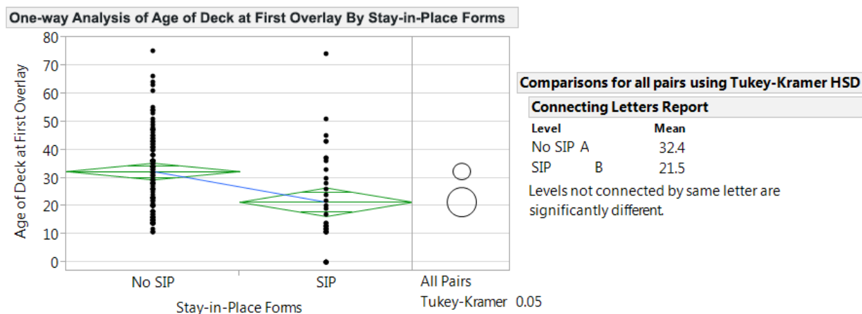
Figure 22. One-way Analysis of Age of Bridge Deck at First Overlay by Presence of Stay-in-Place Forms. SIP = decks with stay-in-place forms; No SIP = decks without stay-in-place forms.
