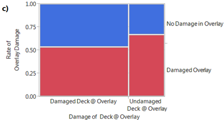
Figure 38. Independence Test: Rate of Damage in Silica Fume Overlays vs. (a) Cracks in Deck at Overlay, (b) Surface Wear of Deck at Overlay, and (c) Damages in Deck at Overlay
