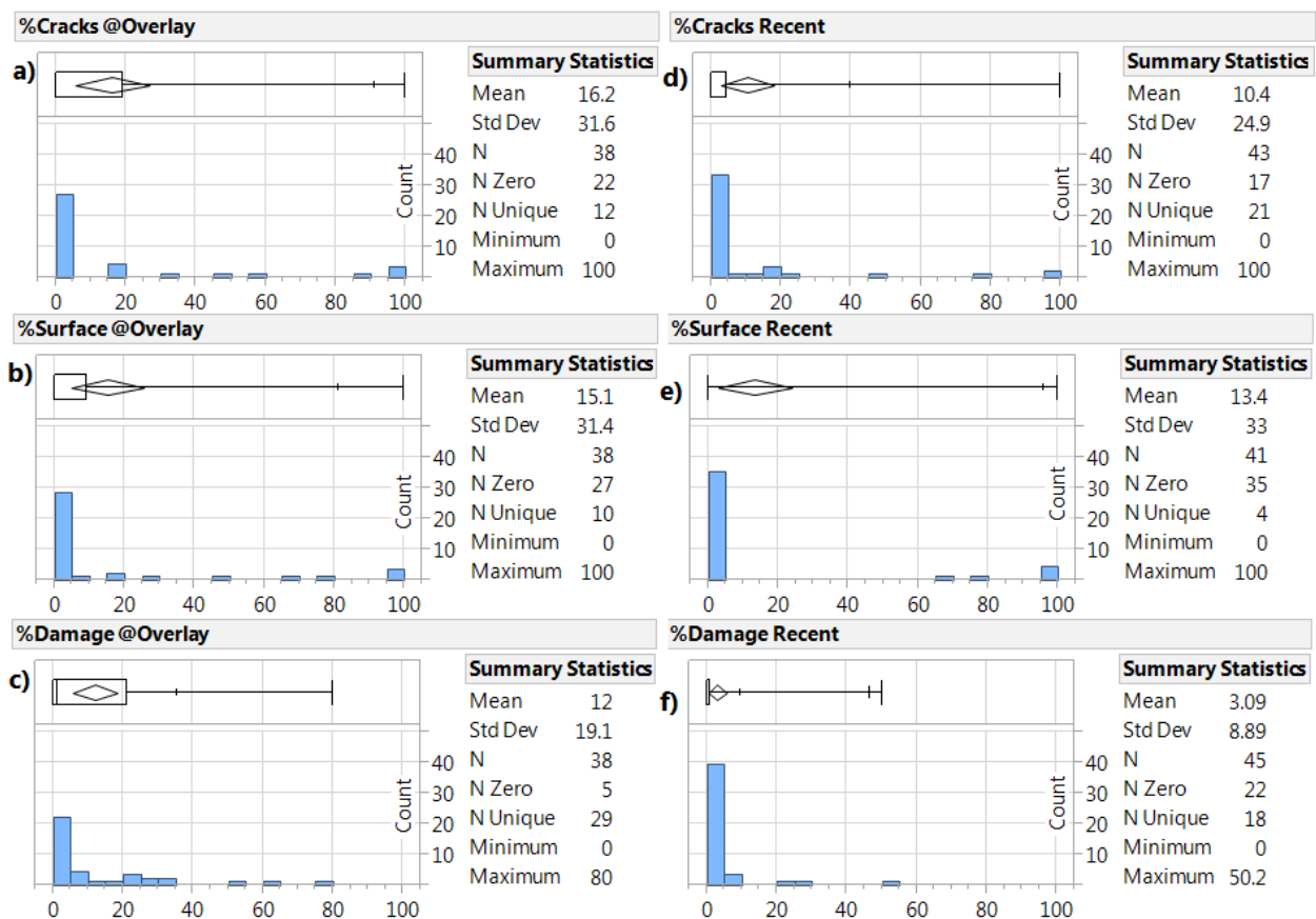
Figure 15. Histograms for Very-Early-Strength Latex-Modified Concrete Overlays: (a) %Cracks at Overlay; (b) %Surface Wear at Overlay; (c) %Damage at Overlay; (d) %Cracks Recent; (e) %Surface Wear Recent; (f) %Damage Recent
