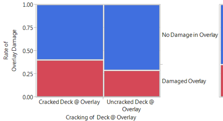
Mosaic Plot
