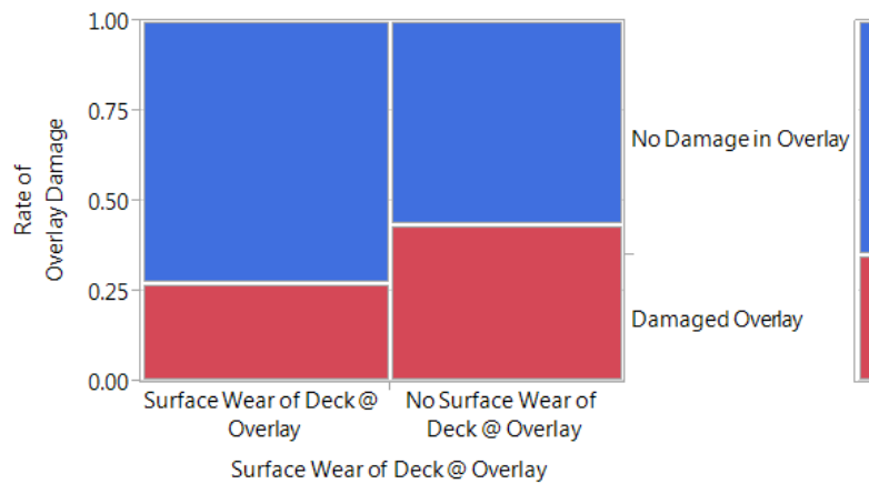
Mosaic Plot
