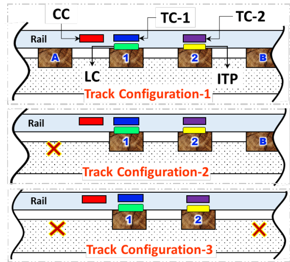
LC: Load Cell ; ITP: Instrumented Tie Plate; CC: Crib Circuit; TC-1: Tie Circuit-1; TC-2: Tie Circuit-2
