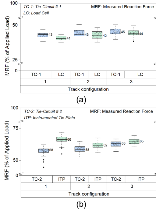
Figure 4: Comparison of TC Results with (a) LCs and (b) ITP
