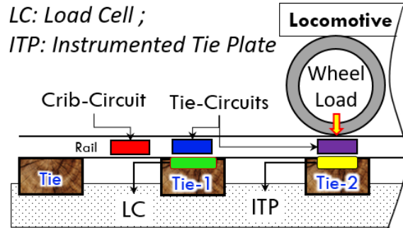
Figure 1: Instrumentation Layout
