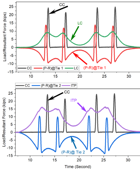
Figure 3: Time Histories from Strain Gauge, LC, and ITP Circuits
