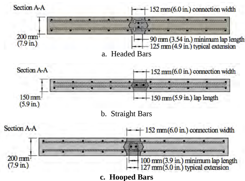
Figure 3.4 UHPC-Filled Deck Panel-to-Panel Longitudinal Joint Detailing (Graybeal, 2010)
