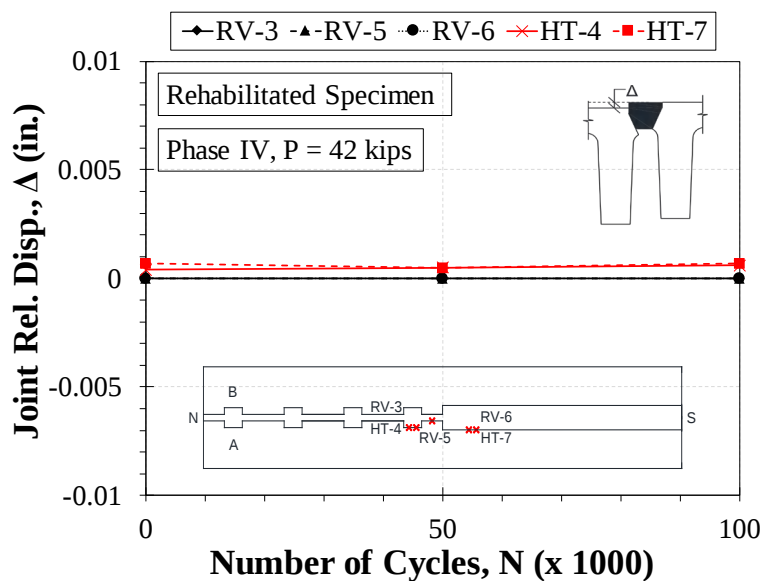
Figure 6.20 Longitudinal Joint Relative Displacement for Rehabilitated Double-Tee Bridge Specimen during Fatigue I Testing
