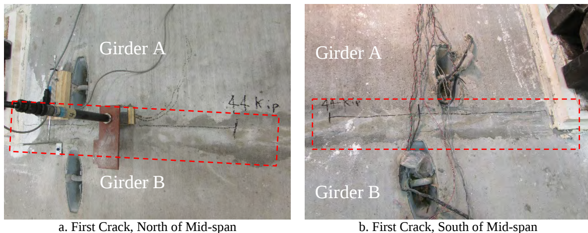
Figure 6.5 Girder-to-Girder Joint Cracking of Conventional Double-Tee Bridge Specimen
