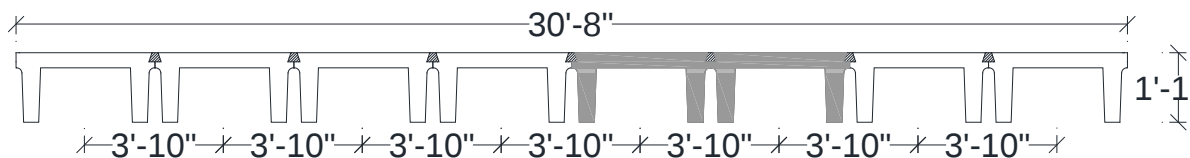
Figure 5.1 Cross-Section of Typical Double-Tee Girder Bridges
