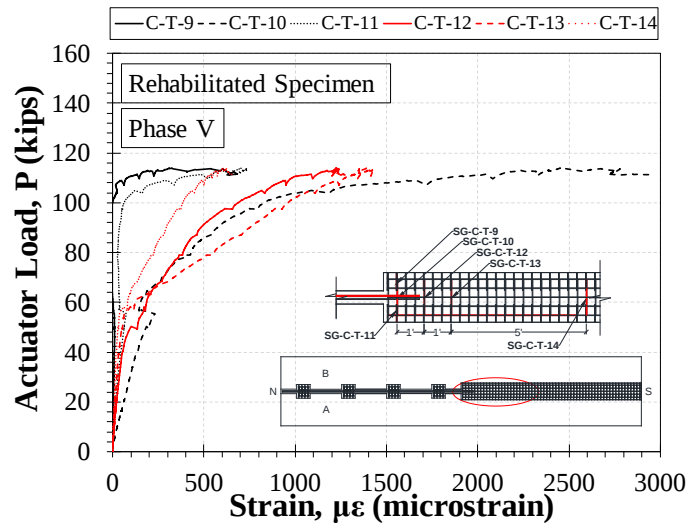
Figure 6.28 Measured Strains of Transverse Reinforcement in LMC Continuous Joint of Rehabilitated Double-Tee Bridge Specimen during Strength Testing
