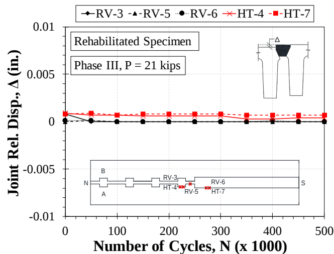
Figure 6.16 Longitudinal Joint Relative Displacements for Rehabilitated Double-Tee Bridge Specimen during Fatigue II Testing
