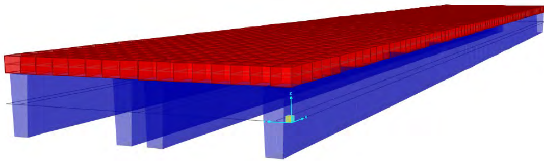
a. Extruded View of FEA Model for Continuous Joint
