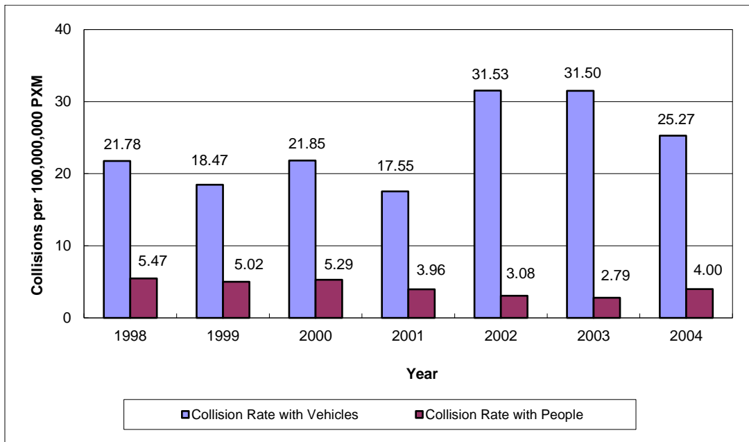
Figure 5. LRT collision rate per 100-million passenger-miles (no suicides) 1998-2004
