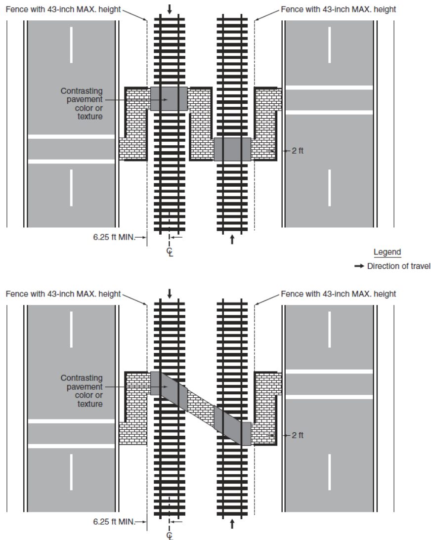
Figure 52. Pedestrian barrier installation at an offset non-intersection grade crossing (MUTCD figure 8C-10)
