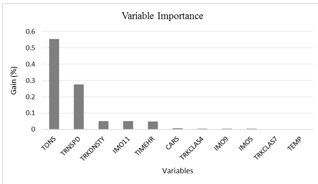
Figure 3.11 Feature importance ranking in monetary loss Source: (Dhingra, Bridgelall, Lu, Szmerekovsky, & Bhardwaj, 2019)
