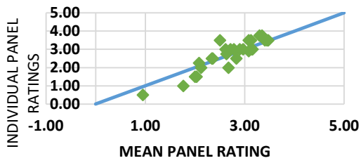
◆ R1 Performance — Unity Line
