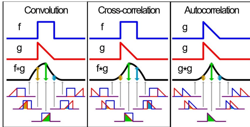
Figure 3.9 Comparison Between Convolution, Cross- Correlation and Autocorrelation, Adapted from (Cmglee [Own Work], 2016)
